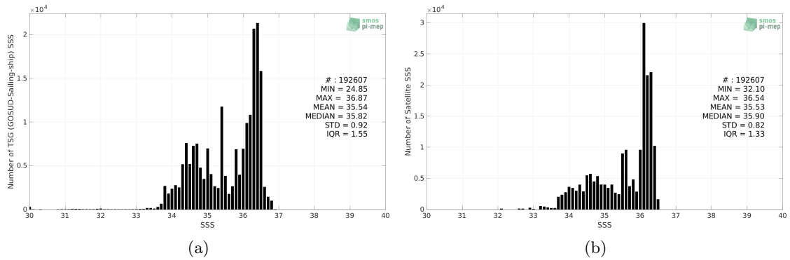
Figure 2: Histograms of SSS from TSG (GOSUD-Sailing-ship) (a) and CCI SSS L4 Merged-OI v3.2 - 30-day running (ESA) (b) considering all match-up pairs per bins of 0.1 over the South Pacific Ocean Pi-MEP region and for the full satellite product period.
