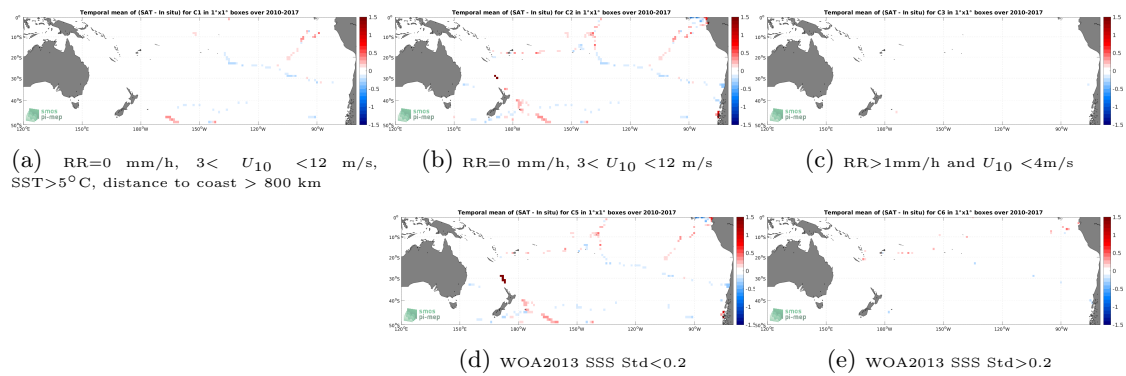
Figure 12: Temporal mean gridded over spatial boxes of size 1^\circ \times 1^\circ of \Delta SSS (CCI SSS L4 Merged-OI v3.2 - 30-day running (ESA) - TSG (GOSUD-Sailing-ship)) for 5 different subdatasets corresponding to:RR=0 mm/h, 3 < U_{10} < 12 m/s, SST >5^\circ\text{C} , distance to coast > 800 km (a), RR=0 mm/h, 3 < U_{10} < 12 m/s (b), RR >1 mm/h and U_{10} < 4 m/s (c), WOA2013 SSS Std <0.2 (d), WOA2013 SSS Std >0.2 (e).
