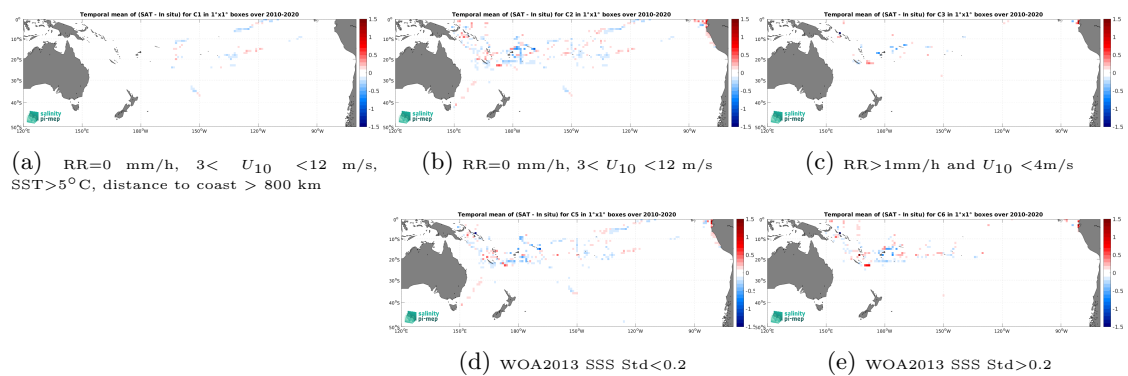
Figure 12: Temporal mean gridded over spatial boxes of size 1^\circ \times 1^\circ of \Delta\text{SSS} (CCI SSS L4 Merged-OI v3.2 - 30-day running (ESA) - TSG (GOSUD-Research-vessel)) for 5 different subdatasets corresponding to:RR=0 mm/h, 3 < U_{10} < 12 m/s, SST >5^\circ\text{C} , distance to coast > 800 km (a), RR=0 mm/h, 3 < U_{10} < 12 m/s (b), RR >1 mm/h and U_{10} < 4 m/s (c), WOA2013 SSS Std <0.2 (d), WOA2013 SSS Std >0.2 (e).
