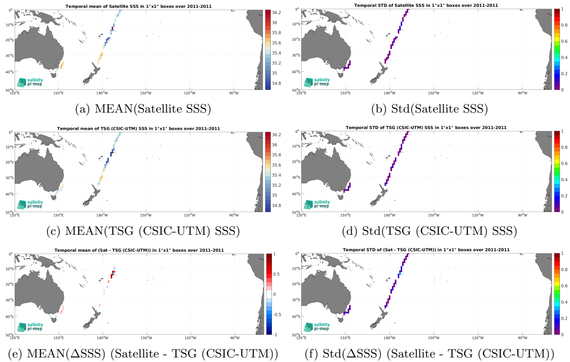
Figure 6: Temporal mean (left) and Std (right) of SSS from CCI SSS L4 Merged-OI v3.2 - 30-day running (ESA) (top), TSG (CSIC-UTM) ( in situ ) dataset (middle), and of \Delta SSS (Satellite - TSG (CSIC-UTM)). Only match-up pairs are used to generate these maps.
