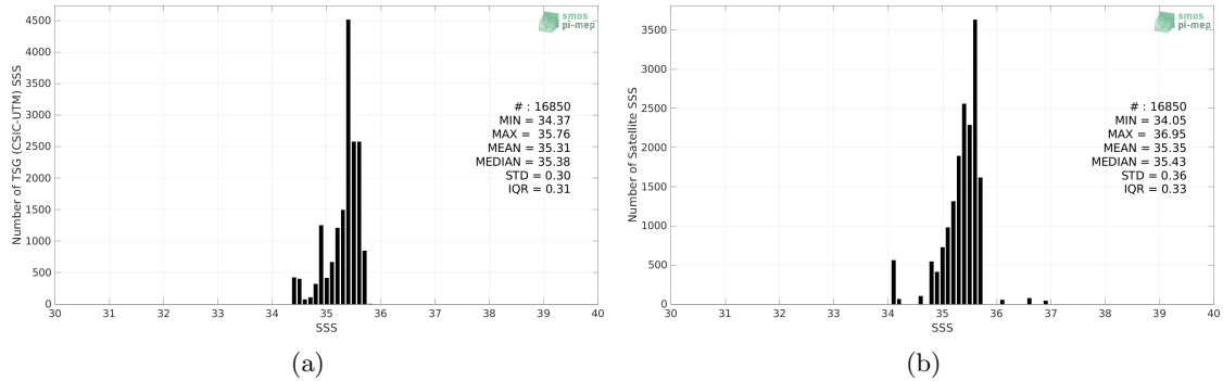
Figure 2: Histograms of SSS from TSG (CSIC-UTM) (a) and CCI SSS L4 Merged-OI v3.2 - 30-day running (ESA) (b) considering all match-up pairs per bins of 0.1 over the South Pacific Ocean Pi-MEP region and for the full satellite product period.
