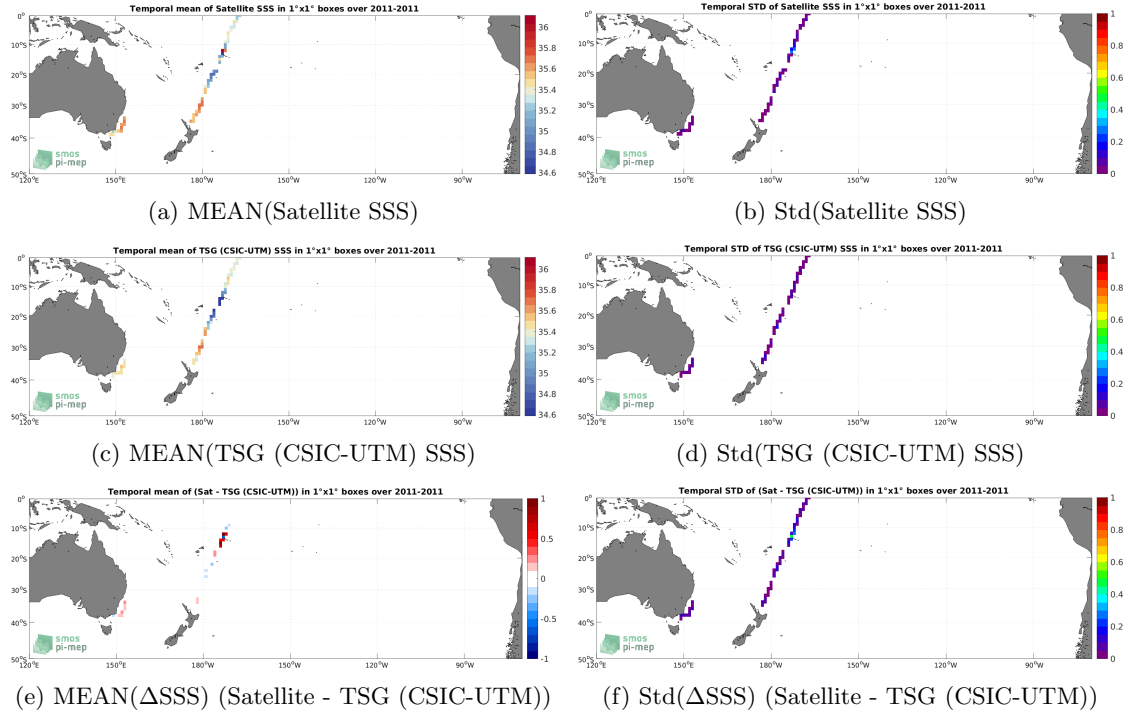
Figure 6: Temporal mean (left) and Std (right) of SSS from CCI SSS L4 Merged-OI v3.2 - 30-day running (ESA) (top), TSG (CSIC-UTM) (middle), and of \Delta SSS (Satellite - TSG (CSIC-UTM)). Only match-up pairs are used to generate these maps.
