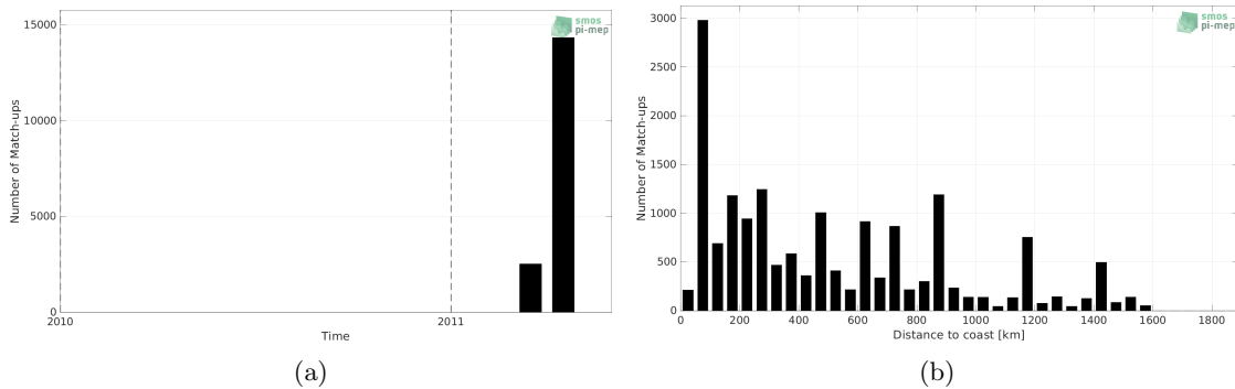
Figure 1: Number of match-ups between TSG (CSIC-UTM) and CCI SSS L4 Merged-OI v3.2 - 30-day running (ESA) SSS as a function of time (a) and as function of the distance to coast (b) over the South Pacific Ocean Pi-MEP region and for the full satellite product period.
