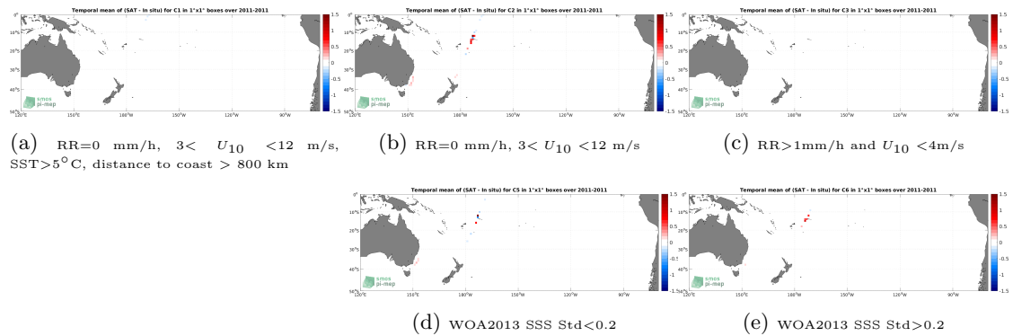
Figure 12: Temporal mean gridded over spatial boxes of size 1^\circ \times 1^\circ of \Delta SSS (CCI SSS L4 Merged-OI v3.2 - 30-day running (ESA) - TSG (CSIC-UTM)) for 5 different subdatasets corresponding to:RR=0 mm/h, 3 < U_{10} < 12 m/s, SST >5^\circ C, distance to coast > 800 km (a), RR=0 mm/h, 3 < U_{10} < 12 m/s (b), RR >1 mm/h and U_{10} < 4 m/s (c), WOA2013 SSS Std <0.2 (d), WOA2013 SSS Std >0.2 (e).
