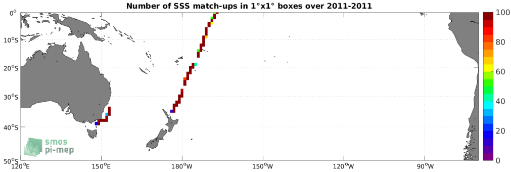
Figure 4: Number of SSS match-ups between TSG (CSIC-UTM) SSS and the CCI SSS L4 Merged-OI v3.2 - 30-day running (ESA) SSS product for the South Pacific Ocean Pi-MEP region over 1^\circ \times 1^\circ boxes and for the full satellite product period.
