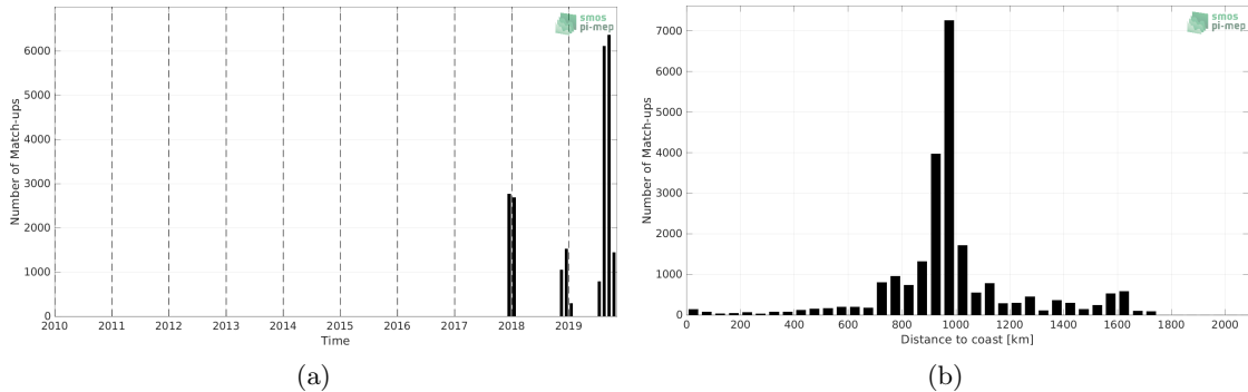
Figure 1: Number of match-ups between Saildrone and CCI SSS L4 Merged-OI v3.2 - 30-day running (ESA) SSS as a function of time (a) and as function of the distance to coast (b) over the South Pacific Ocean Pi-MEP region and for the full satellite product period.
