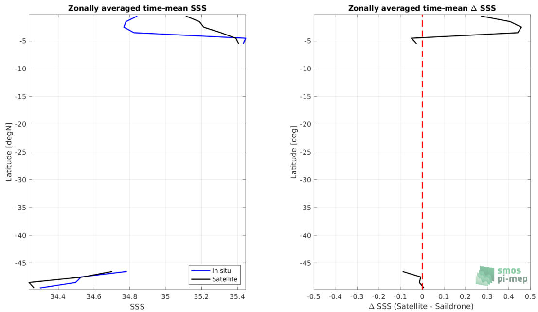
Figure 8: Left panel: Zonal mean SSS from CCI SSS L4 Merged-OI v3.2 - 30-day running (ESA) satellite product (black) and from Sairdronne (blue). Right panel: Zonal mean of \Delta SSS (Satellite - Sairdronne) for all the collected Pi-MEP match-up pairs estimated over the full satellite product period.
