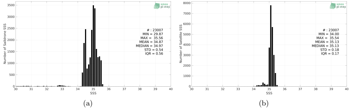
Figure 2: Histograms of SSS from Saildrone (a) and CCI SSS L4 Merged-OI v3.2 - 30-day running (ESA) (b) considering all match-up pairs per bins of 0.1 over the South Pacific Ocean Pi-MEP region and for the full satellite product period.
