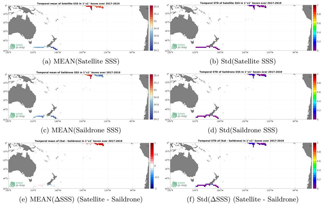
Figure 6: Temporal mean (left) and Std (right) of SSS from CCI SSS L4 Merged-OI v3.2 - 30-day running (ESA) (top), Saildrone (middle), and of \Delta SSS (Satellite - Saildrone). Only match-up pairs are used to generate these maps.
