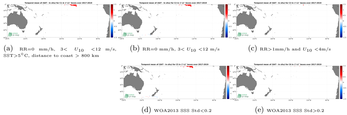
Figure 12: Temporal mean gridded over spatial boxes of size 1^\circ \times 1^\circ of \Delta SSS (CCI SSS L4 Merged-OI v3.2 - 30-day running (ESA) - Saildrone) for 5 different subdatasets corresponding to:RR=0 mm/h, 3 < U_{10} < 12 m/s, SST >5^\circ C, distance to coast > 800 km (a), RR=0 mm/h, 3 < U_{10} < 12 m/s (b), RR >1 mm/h and U_{10} < 4 m/s (c), WOA2013 SSS Std <0.2 (d), WOA2013 SSS Std >0.2 (e).
