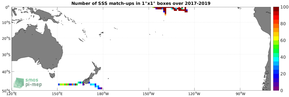
Figure 4: Number of SSS match-ups between Saildrone SSS and the CCI SSS L4 Merged-OI v3.2 - 30-day running (ESA) SSS product for the South Pacific Ocean Pi-MEP region over 1^\circ \times 1^\circ boxes and for the full satellite product period.
