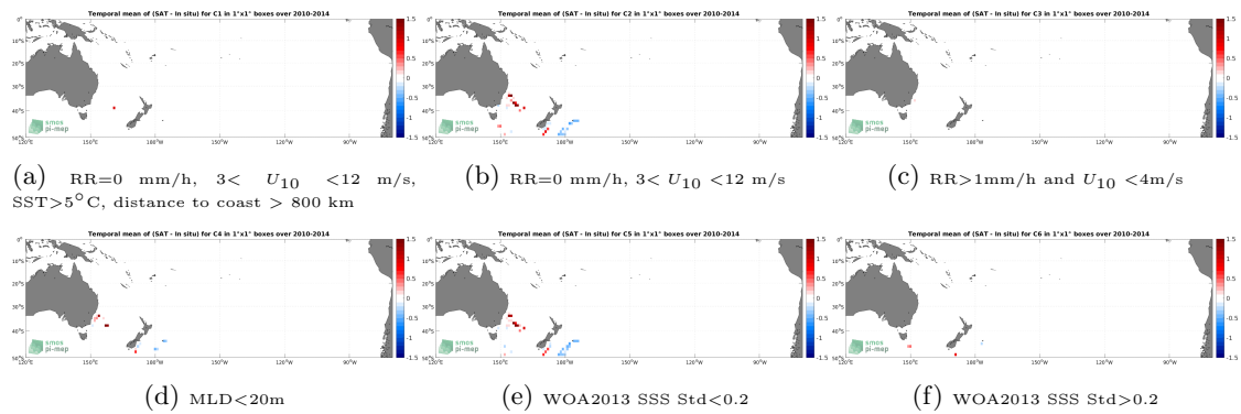
Figure 12: Temporal mean gridded over spatial boxes of size 1^\circ \times 1^\circ of \Delta SSS (CCI SSS L4 Merged-OI v3.2 - 30-day running (ESA) - Marine mammals) for 6 different subdatasets corresponding to:RR=0 mm/h, 3 < U_{10} < 12 m/s, SST >5^\circ C, distance to coast > 800 km (a), RR=0 mm/h, 3 < U_{10} < 12 m/s (b), RR >1 mm/h and U_{10} < 4 m/s (c),MLD <20 m (d),WOA2013 SSS Std <0.2 (e),WOA2013 SSS Std >0.2 (f).
