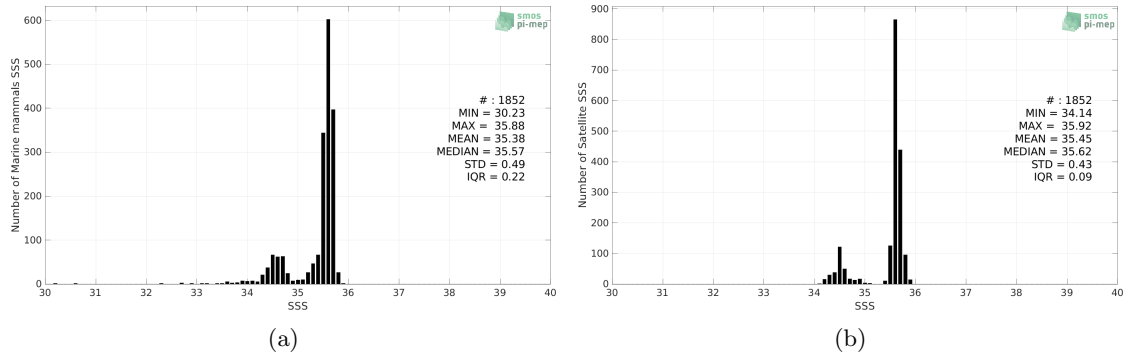
Figure 2: Histograms of SSS from Marine mammals (a) and CCI SSS L4 Merged-OI v3.2 - 30-day running (ESA) (b) considering all match-up pairs per bins of 0.1 over the South Pacific Ocean Pi-MEP region and for the full satellite product period.
