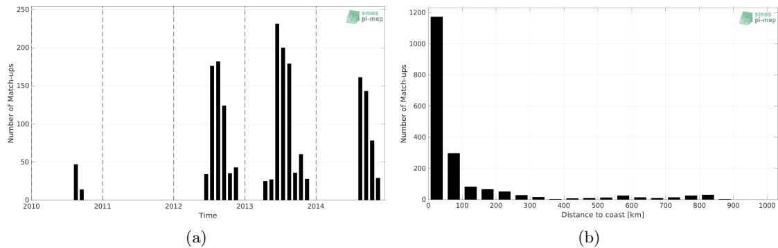
Figure 1: Number of match-ups between Marine mammals and CCI SSS L4 Merged-OI v3.2 - 30-day running (ESA) SSS as a function of time (a) and as function of the distance to coast (b) over the South Pacific Ocean Pi-MEP region and for the full satellite product period.
