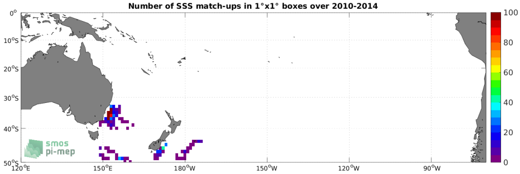
Figure 4: Number of SSS match-ups between Marine mammals SSS and the CCI SSS L4 Merged-OI v3.2 - 30-day running (ESA) SSS product for the South Pacific Ocean Pi-MEP region over 1^\circ \times 1^\circ boxes and for the full satellite product period.
