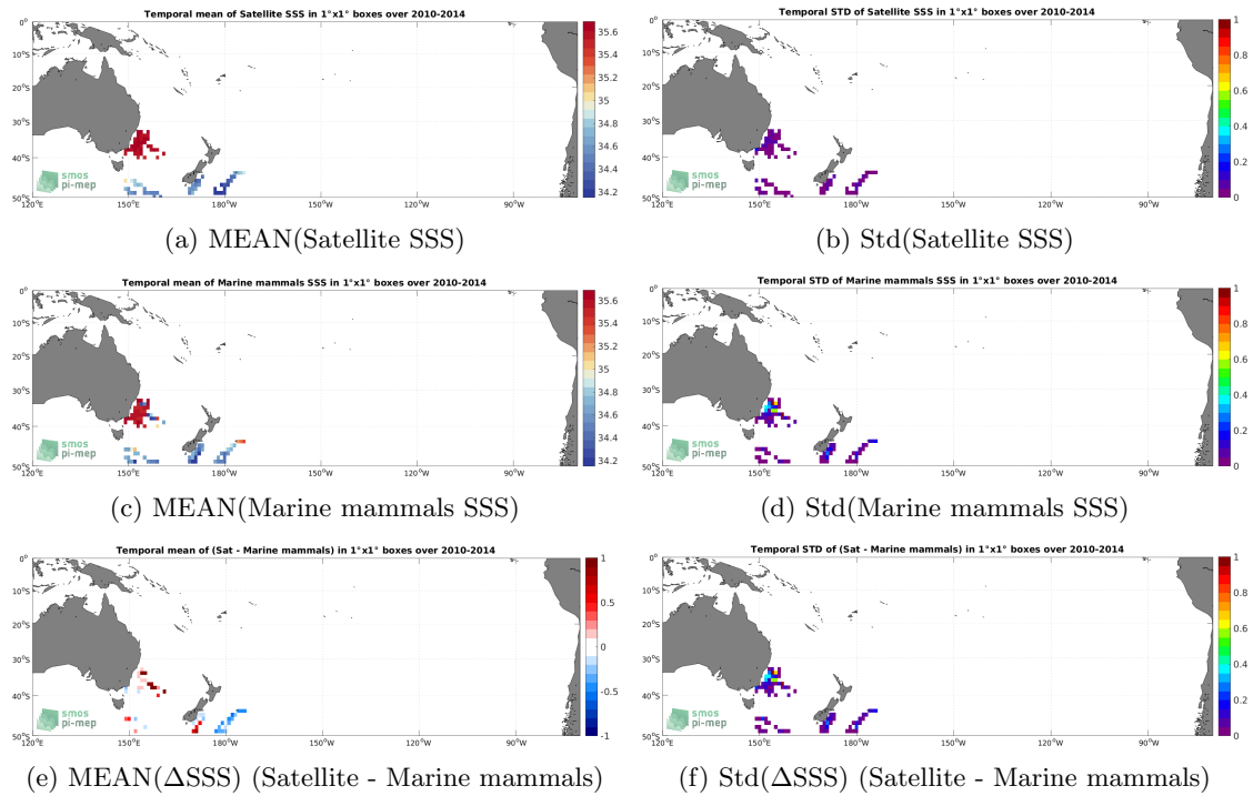
Figure 6: Temporal mean (left) and Std (right) of SSS from CCI SSS L4 Merged-OI v3.2 - 30-day running (ESA) (top), Marine mammals (middle), and of \Delta SSS (Satellite - Marine mammals). Only match-up pairs are used to generate these maps.
