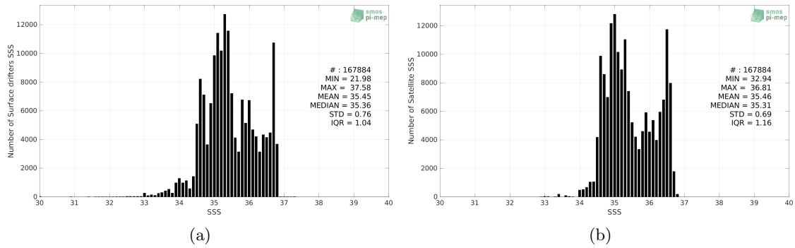
Figure 2: Histograms of SSS from Surface drifters (a) and CCI SSS L4 Merged-OI v3.2 - 30-day running (ESA) (b) considering all match-up pairs per bins of 0.1 over the South Pacific Ocean Pi-MEP region and for the full satellite product period.
