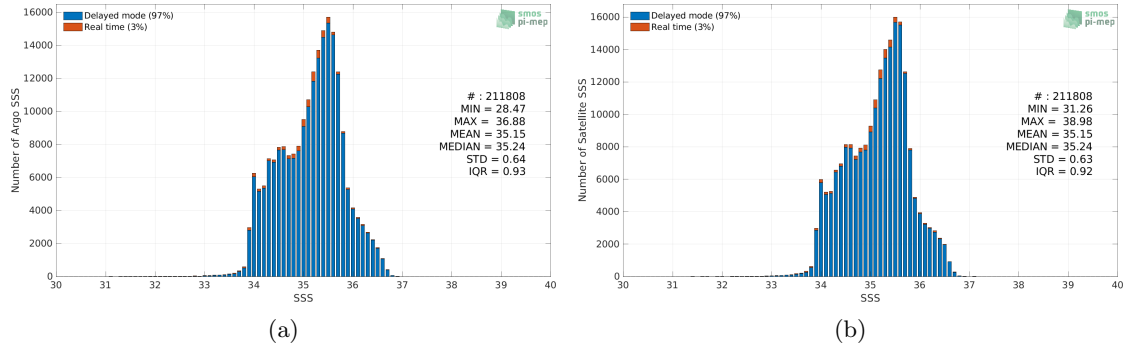
Figure 2: Histograms of SSS from Argo (a) and CCI SSS L4 Merged-OI v3.2 - 30-day running (ESA) (b) considering all match-up pairs per bins of 0.1 over the South Pacific Ocean Pi-MEP region and for the full satellite product period.
