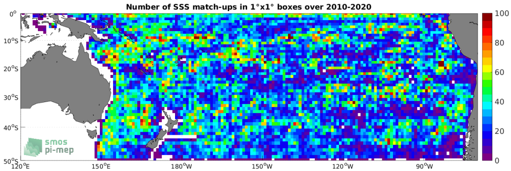
Figure 4: Number of SSS match-ups between Argo SSS and the CCI SSS L4 Merged-OI v3.2 - 30-day running (ESA) SSS product for the South Pacific Ocean Pi-MEP region over 1^\circ \times 1^\circ boxes and for the full satellite product period.
