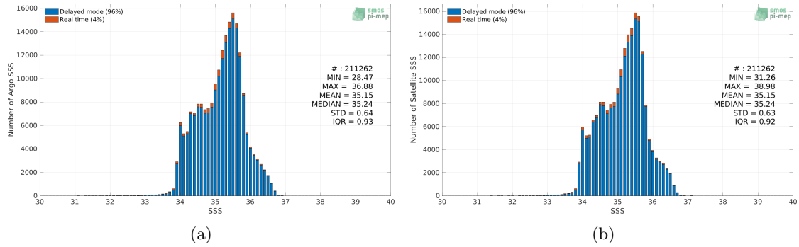
Figure 2: Histograms of SSS from Argo (a) and CCI SSS L4 Merged-OI v3.2 - 30-day running (ESA) (b) considering all match-up pairs per bins of 0.1 over the South Pacific Ocean Pi-MEP region and for the full satellite product period.
