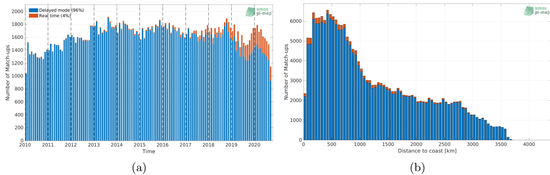
Figure 1: Number of match-ups between Argo and CCI SSS L4 Merged-OI v3.2 - 30-day running (ESA) SSS as a function of time (a) and as function of the distance to coast (b) over the South Pacific Ocean Pi-MEP region and for the full satellite product period.
