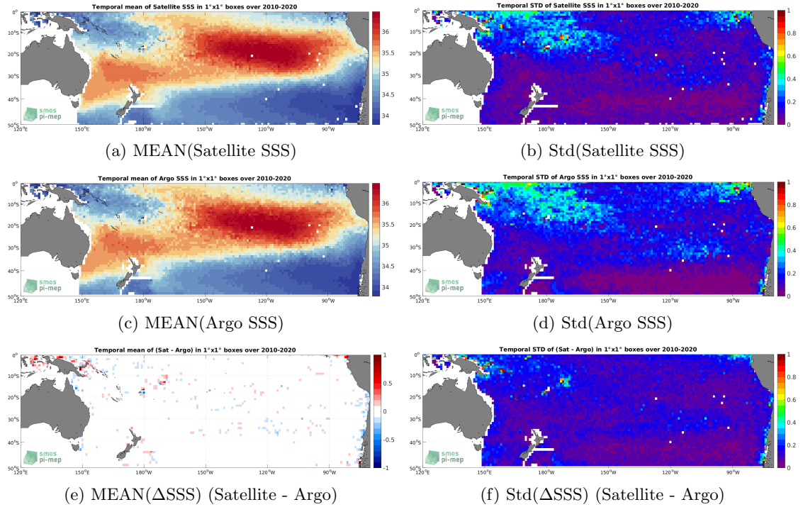
Figure 6: Temporal mean (left) and Std (right) of SSS from CCI SSS L4 Merged-OI v3.2 - 30-day running (ESA) (top), Argo (middle), and of \Delta SSS (Satellite - Argo). Only match-up pairs are used to generate these maps.
