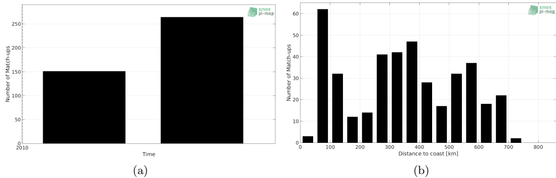
Figure 1: Number of match-ups between TSG (Polarstern) and CCI L4 Merged-OI v2.31 - 30-day running (ESA) SSS as a function of time (a) and as function of the distance to coast (b) over the South Pacific Ocean Pi-MEP region and for the full satellite product period.
