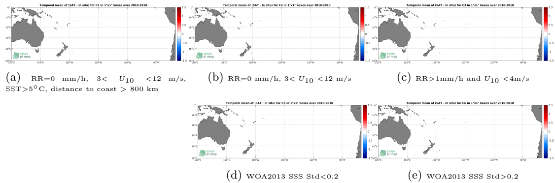
Figure 12: Temporal mean gridded over spatial boxes of size 1^{\circ}\times 1^{\circ} of \Delta\text{SSS} (CCI L4 Merged-OI v2.31 - 30-day running (ESA) - TSG (Polarstern)) for 5 different subdatasets corresponding to:RR=0 mm/h, 3 < U_{10} < 12 m/s, SST >5^{\circ}\text{C} , distance to coast > 800 km (a), RR=0 mm/h, 3 < U_{10} < 12 m/s (b), RR >1 mm/h and U_{10} < 4 m/s (c), WOA2013 SSS Std <0.2 (d), WOA2013 SSS Std >0.2 (e).
