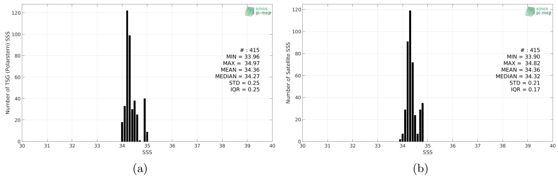
Figure 2: Histograms of SSS from TSG (Polarstern) (a) and CCI L4 Merged-OI v2.31 - 30-day running (ESA) (b) considering all match-up pairs per bins of 0.1 over the South Pacific Ocean Pi-MEP region and for the full satellite product period.
