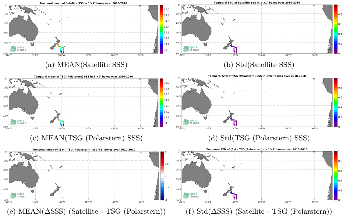
Figure 6: Temporal mean (left) and Std (right) of SSS from CCI L4 Merged-OI v2.31 - 30-day running (ESA) (top), TSG (Polarstern) (middle), and of \Delta SSS (Satellite - TSG (Polarstern)). Only match-up pairs are used to generate these maps.
