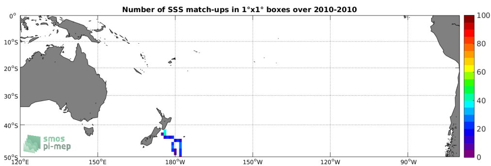
Figure 4: Number of SSS match-ups between TSG (Polarstern) SSS and the CCI L4 Merged-OI v2.31 - 30-day running (ESA) SSS product for the South Pacific Ocean Pi-MEP region over 1^\circ \times 1^\circ boxes and for the full satellite product period.
