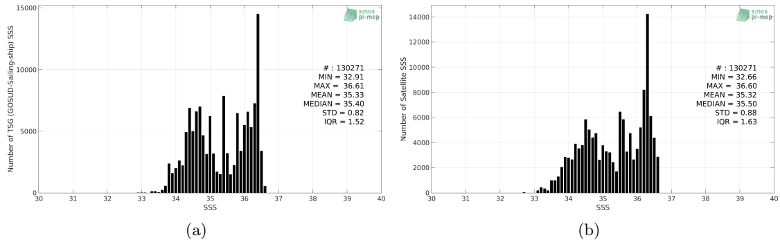
Figure 2: Histograms of SSS from TSG (GOSUD-Sailing-ship) (a) and CCI L4 Merged-OI v2.31 - 30-day running (ESA) (b) considering all match-up pairs per bins of 0.1 over the South Pacific Ocean Pi-MEP region and for the full satellite product period.
