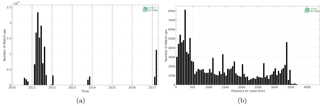
Figure 1: Number of match-ups between TSG (GOSUD-Sailing-ship) and CCI L4 Merged-OI v2.31 - 30-day running (ESA) SSS as a function of time (a) and as function of the distance to coast (b) over the South Pacific Ocean Pi-MEP region and for the full satellite product period.
