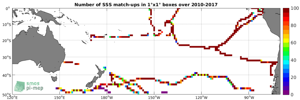
Figure 4: Number of SSS match-ups between TSG (GOSUD-Sailing-ship) SSS and the CCI L4 Merged-OI v2.31 - 30-day running (ESA) SSS product for the South Pacific Ocean Pi-MEP region over 1^\circ \times 1^\circ boxes and for the full satellite product period.
