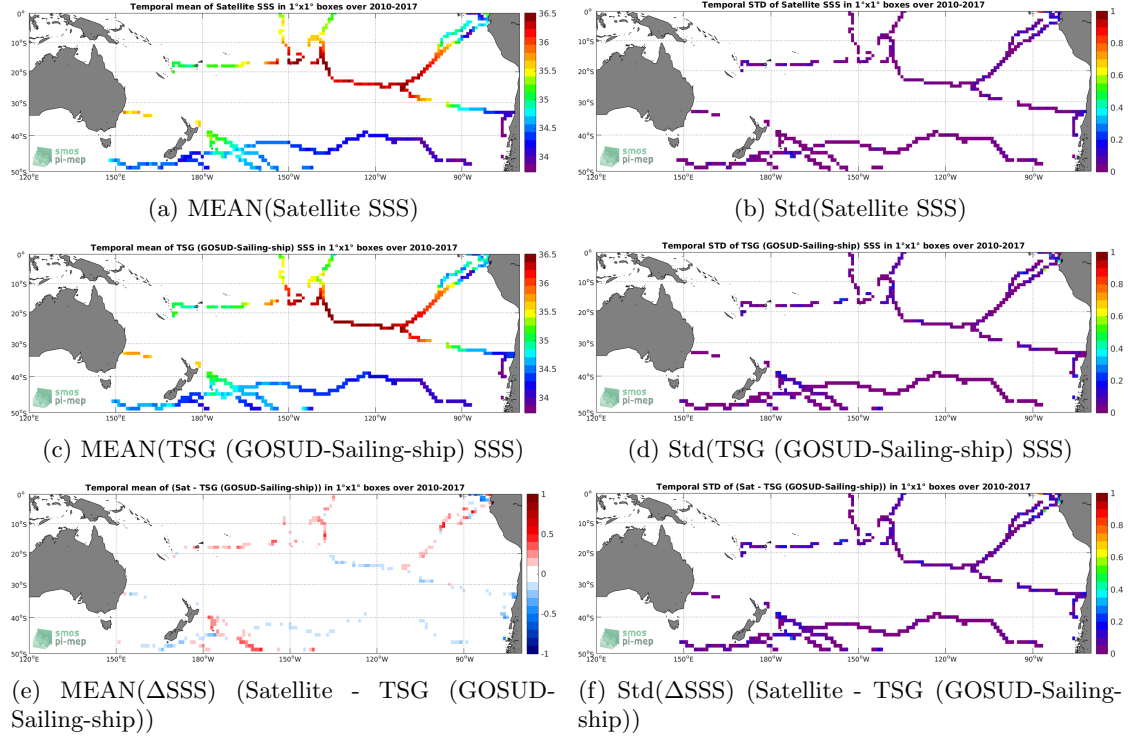
Figure 6: Temporal mean (left) and Std (right) of SSS from CCI L4 Merged-OI v2.31 - 30-day running (ESA) (top), TSG (GOSUD-Sailing-ship) (middle), and of \Delta SSS (Satellite - TSG (GOSUD-Sailing-ship)). Only match-up pairs are used to generate these maps.
