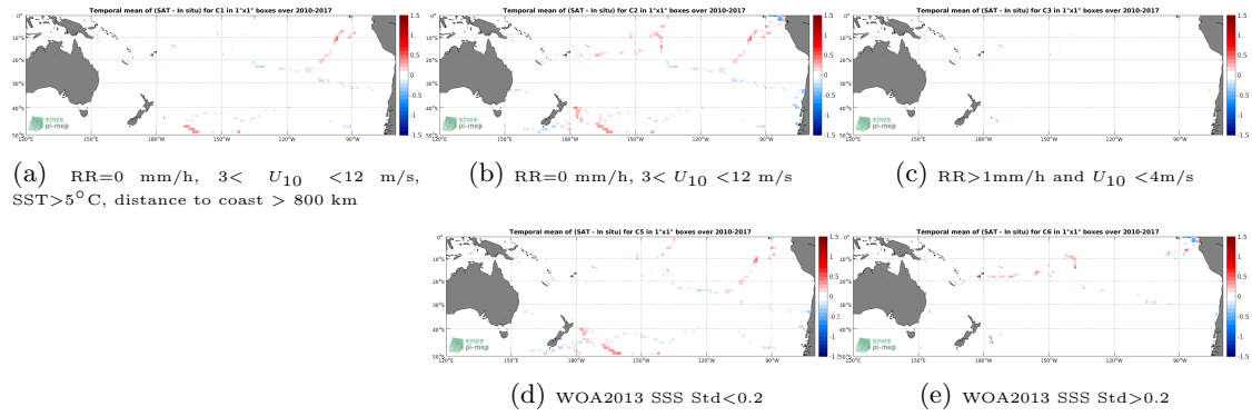
Figure 12: Temporal mean gridded over spatial boxes of size 1^\circ \times 1^\circ of \Delta SSS (CCI L4 Merged-OI v2.31 - 30-day running (ESA) - TSG (GOSUD-Sailing-ship)) for 5 different subdatasets corresponding to: RR=0 mm/h, 3 < U_{10} < 12 m/s, SST >5^\circ\text{C} , distance to coast > 800 km (a), RR=0 mm/h, 3 < U_{10} < 12 m/s (b), RR>1\text{mm/h} and U_{10} < 4\text{m/s} (c), WOA2013 SSS Std <0.2 (d), WOA2013 SSS Std >0.2 (e).
