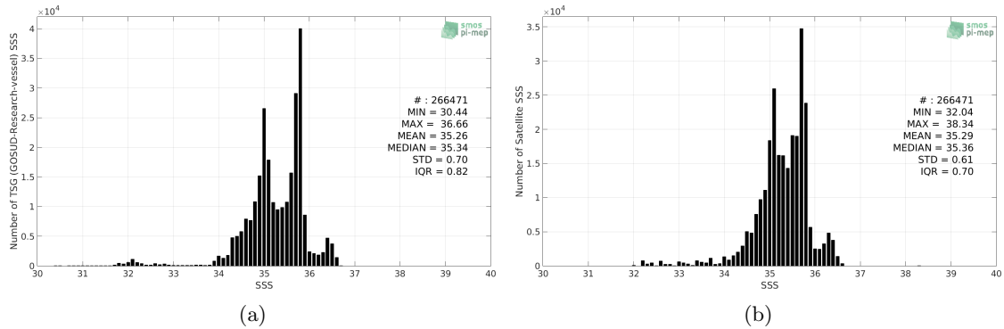
Figure 2: Histograms of SSS from TSG (GOSUD-Research-vessel) (a) and CCI SSS L4 Merged-OI v2.31 - 30-day running (ESA) (b) considering all match-up pairs per bins of 0.1 over the South Pacific Ocean Pi-MEP region and for the full satellite product period.
