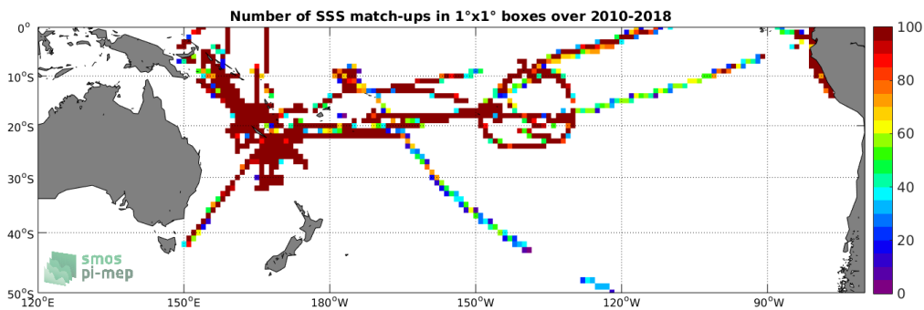
Figure 4: Number of SSS match-ups between TSG (GOSUD-Research-vessel) SSS and the CCI SSS L4 Merged-OI v2.31 - 30-day running (ESA) SSS product for the South Pacific Ocean Pi-MEP region over 1°x1° boxes and for the full satellite product period.
