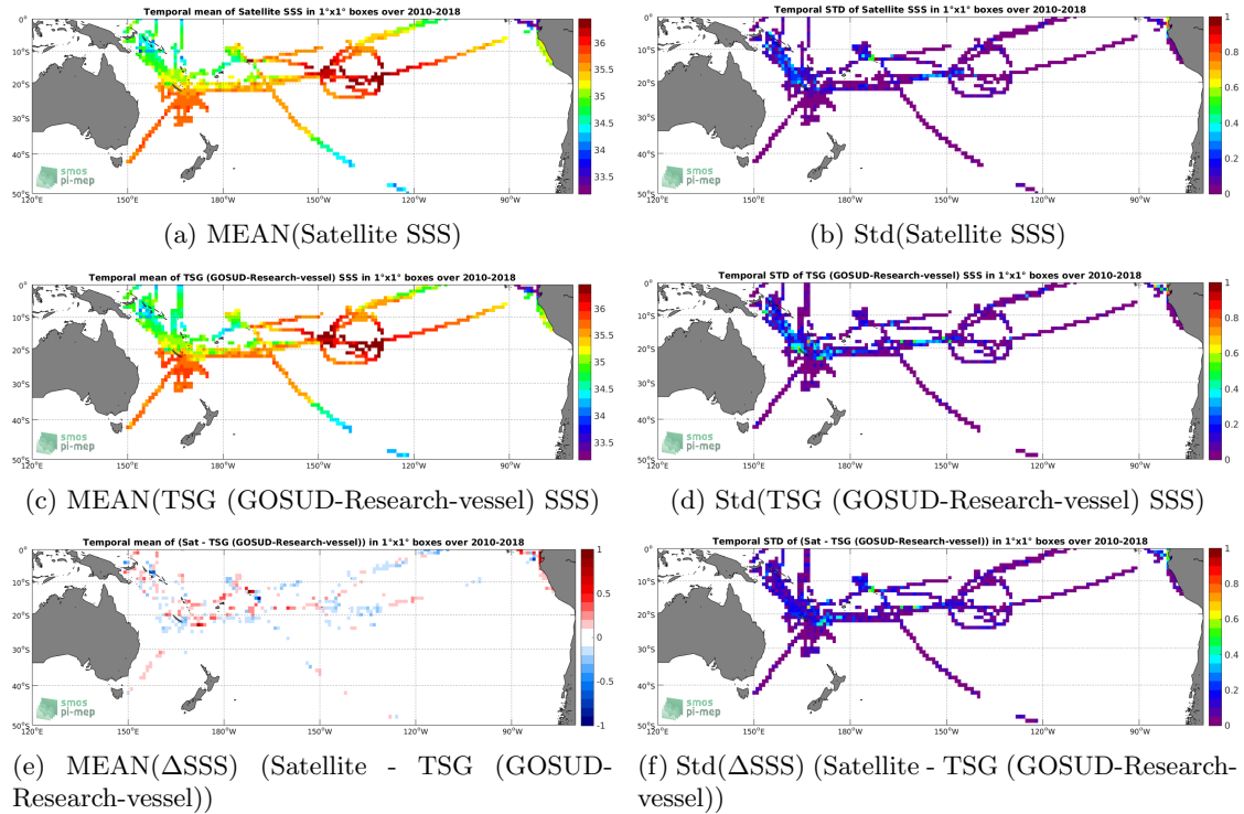
Figure 6: Temporal mean (left) and Std (right) of SSS from CCI SSS L4 Merged-OI v2.31 - 30-day running (ESA) (top), TSG (GOSUD-Research-vessel) (middle), and of \Delta SSS (Satellite - TSG (GOSUD-Research-vessel)). Only match-up pairs are used to generate these maps.
