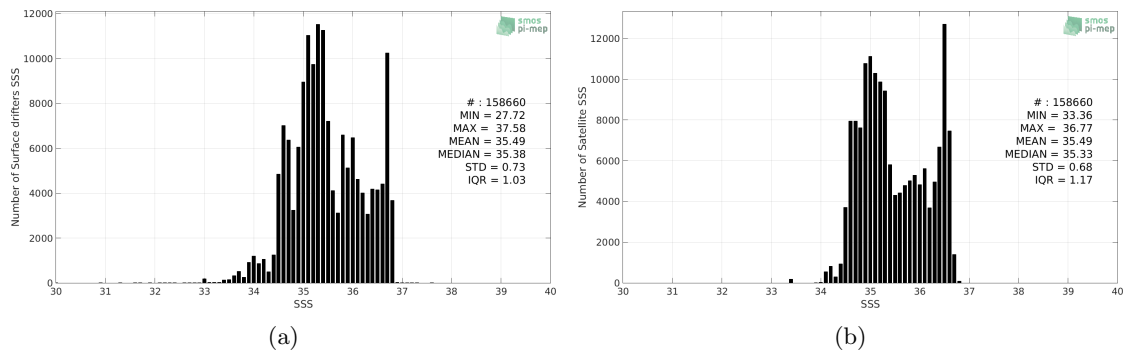
Figure 2: Histograms of SSS from Surface drifters (a) and CCI SSS L4 Merged-OI v2.31 - 30-day running (ESA) (b) considering all match-up pairs per bins of 0.1 over the South Pacific Ocean Pi-MEP region and for the full satellite product period.
