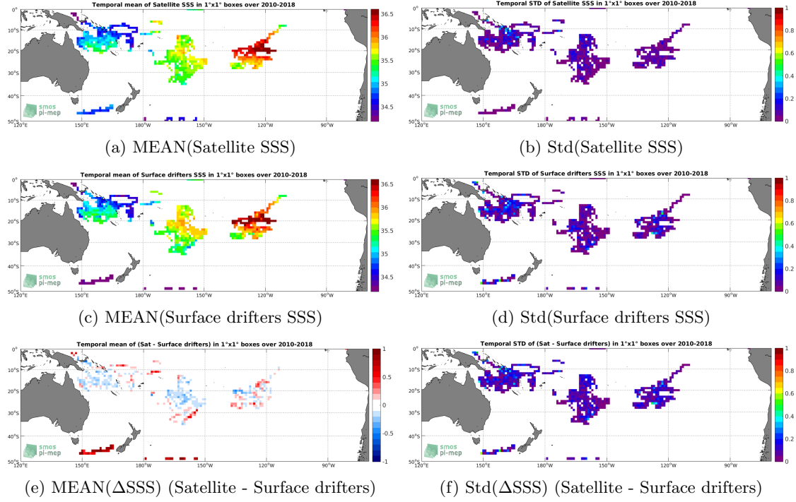
Figure 5: Temporal mean (left) and Std (right) of SSS from CCI SSS L4 Merged-OI v2.31 - 30-day running (ESA) (top), Surface drifters (middle), and of \Delta SSS (Satellite - Surface drifters). Only match-up pairs are used to generate these maps.
