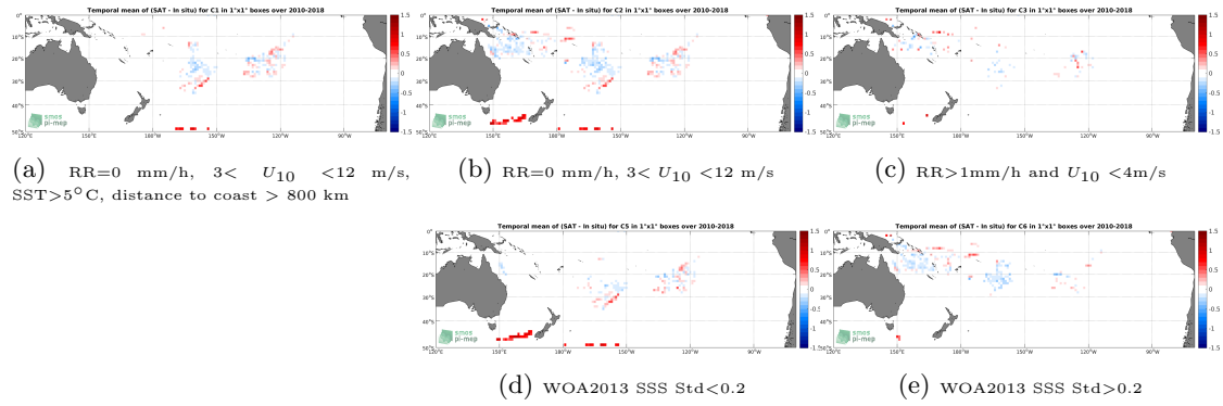
Figure 11: Temporal mean gridded over spatial boxes of size 1^\circ \times 1^\circ of \Delta SSS (CCI SSS L4 Merged-OI v2.31 - 30-day running (ESA) - Surface drifters) for 5 different subdatasets corresponding to: RR=0 mm/h, 3 < U_{10} < 12 m/s, SST >5^\circ\text{C} , distance to coast > 800 km (a), RR=0 mm/h, 3 < U_{10} < 12 m/s (b), RR>1\text{mm/h} and U_{10} < 4\text{m/s} (c), WOA2013 SSS Std <0.2 (d), WOA2013 SSS Std >0.2 (e).
