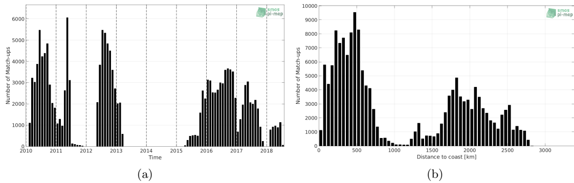
Figure 1: Number of match-ups between Surface drifters and CCI SSS L4 Merged-OI v2.31 - 30-day running (ESA) SSS as a function of time (a) and as function of the distance to coast (b) over the South Pacific Ocean Pi-MEP region and for the full satellite product period.
