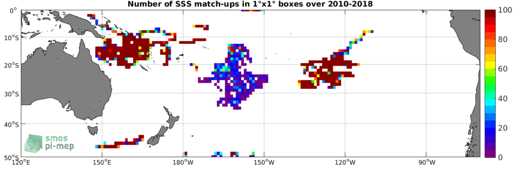
Figure 3: Number of SSS match-ups between Surface drifters SSS and the CCI L4 Merged-OI v2.31 - 30-day running (ESA) SSS product for the South Pacific Ocean Pi-MEP region over 1^\circ \times 1^\circ boxes and for the full satellite product period.
