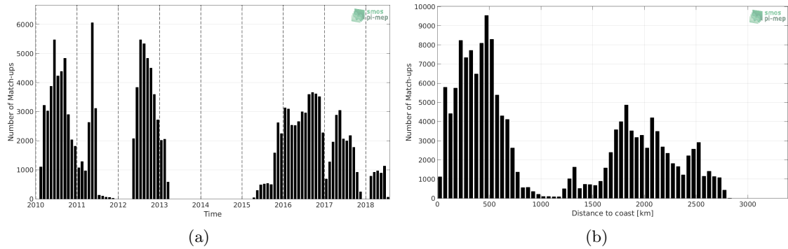
Figure 1: Number of match-ups between Surface drifters and CCI L4 Merged-OI v2.31 - 30-day running (ESA) SSS as a function of time (a) and as function of the distance to coast (b) over the South Pacific Ocean Pi-MEP region and for the full satellite product period.
