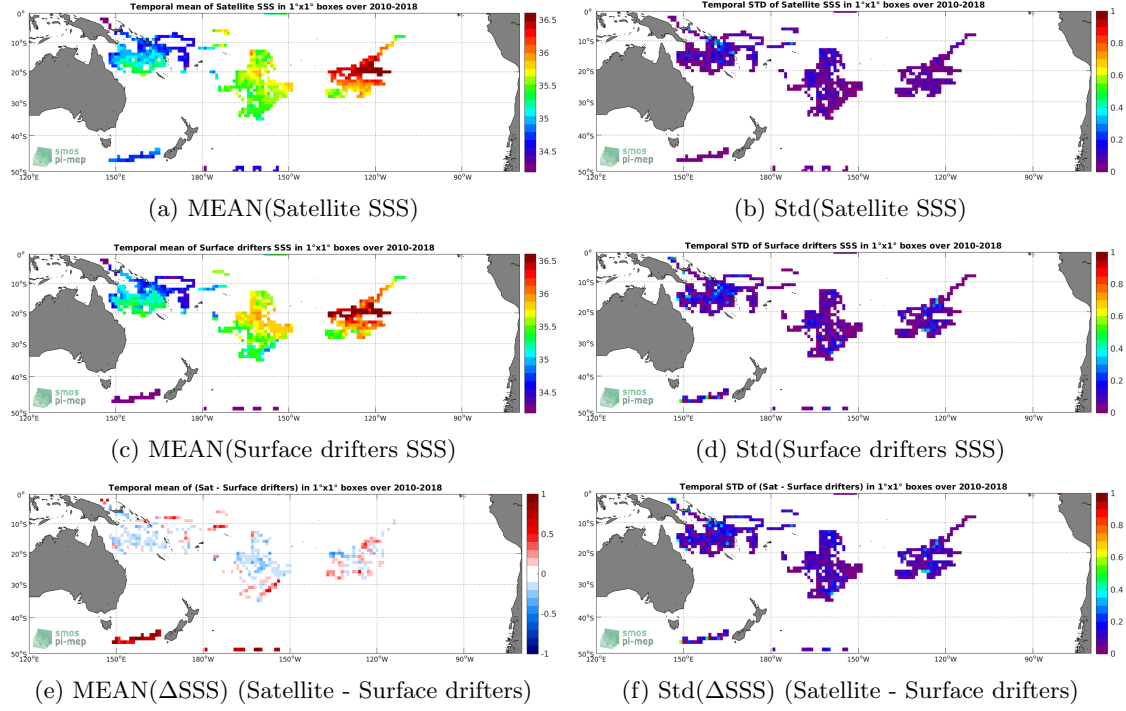
Figure 5: Temporal mean (left) and Std (right) of SSS from CCI L4 Merged-OI v2.31 - 30-day running (ESA) (top), Surface drifters (middle), and of \Delta SSS (Satellite - Surface drifters). Only match-up pairs are used to generate these maps.
