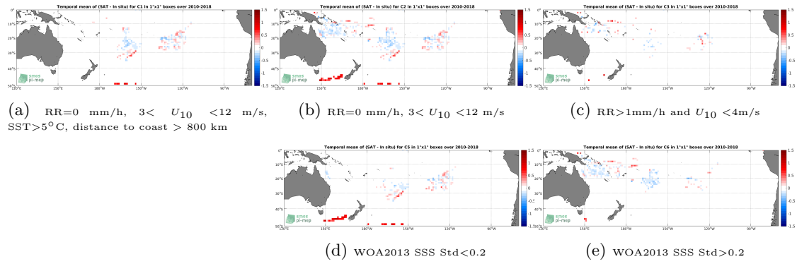
Figure 11: Temporal mean gridded over spatial boxes of size 1^\circ \times 1^\circ of \Delta SSS (CCI L4 Merged-OI v2.31 - 30-day running (ESA) - Surface drifters) for 5 different subdatasets corresponding to: RR=0 mm/h, 3 < U_{10} < 12 m/s, SST > 5^\circ\text{C} , distance to coast > 800 km (a), RR=0 mm/h, 3 < U_{10} < 12 m/s (b), RR > 1 mm/h and U_{10} < 4 m/s (c), WOA2013 SSS Std < 0.2 (d), WOA2013 SSS Std > 0.2 (e).
