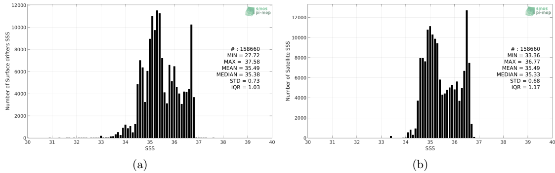
Figure 2: Histograms of SSS from Surface drifters (a) and CCI L4 Merged-OI v2.31 - 30-day running (ESA) (b) considering all match-up pairs per bins of 0.1 over the South Pacific Ocean Pi-MEP region and for the full satellite product period.
