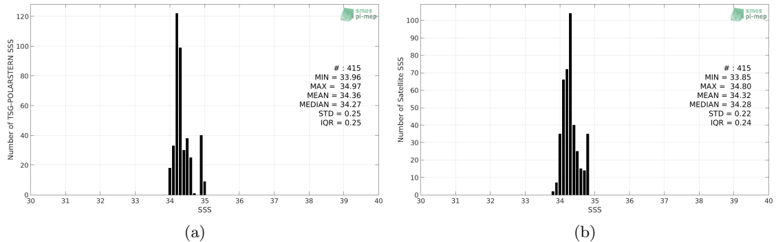
Figure 2: Histograms of SSS from TSG-POLARSTERN (a) and CCI L4 Merged-OI v1.8 - 30-day running (ESA) (b) considering all match-up pairs per bins of 0.1 over the South Pacific Ocean Pi-MEP region and for the full satellite product period.
