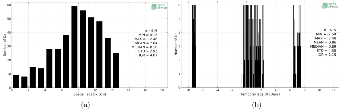
Figure 5: Histograms of the spatial (a) and temporal (b) lags between the time of the TSG-POLARSTERN measurements and the date of the corresponding CCI-L4-ESA-MERGED-OI-V1.8-30DAY-RUNNING SSS product.
