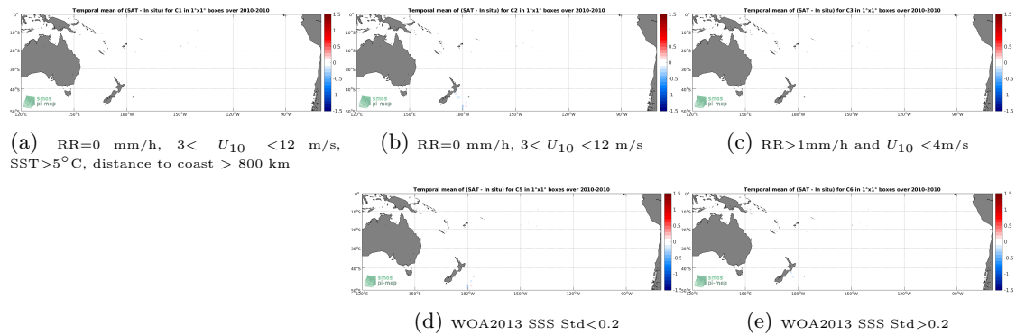
Figure 12: Temporal mean gridded over spatial boxes of size 1^\circ \times 1^\circ of \Delta SSS (CCI-L4-ESA-MERGED-OI-V1.8-30DAY-RUNNING - TSG-POLARSTERN) for 5 different subdatasets corresponding to:RR=0 mm/h, 3 < U_{10} < 12 m/s, SST >5^\circ C, distance to coast > 800 km (a), RR=0 mm/h, 3 < U_{10} < 12 m/s (b), RR >1 mm/h and U_{10} < 4 m/s (c), WOA2013 SSS Std <0.2 (d), WOA2013 SSS Std >0.2 (e).
