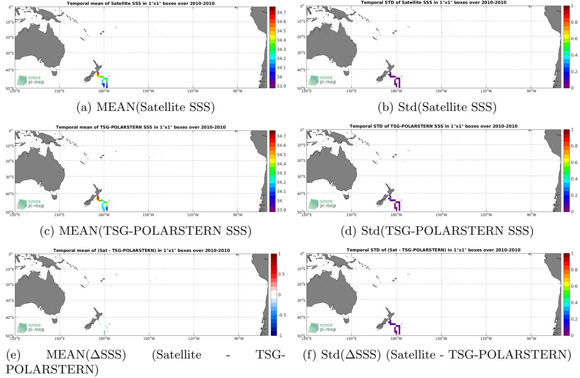
Figure 6: Temporal mean (left) and Std (right) of SSS from CCI-L4-ESA-MERGED-OI-V1.8-30DAY-RUNNING (top), TSG-POLARSTERN (middle), and of \Delta SSS (Satellite - TSG-POLARSTERN). Only match-up pairs are used to generate these maps.
