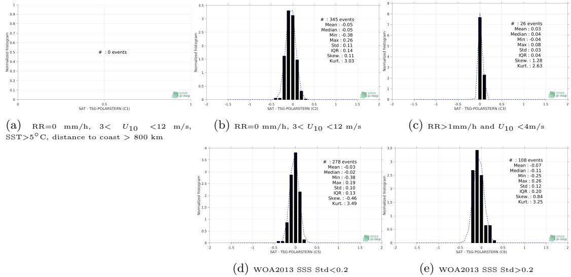
Figure 13: Normalized histogram of \Delta SSS (CCI-L4-ESA-MERGED-OI-V1.8-30DAY-RUNNING - TSG-POLARSTERN) for 5 different subdatasets corresponding to: RR=0 mm/h, 3 < U_{10} < 12 m/s, SST>5°C, distance to coast > 800 km (a), RR=0 mm/h, 3 < U_{10} < 12 m/s (b), RR>1mm/h and U_{10} < 4 m/s (c), WOA2013 SSS Std<0.2 (d), WOA2013 SSS Std>0.2 (e).
