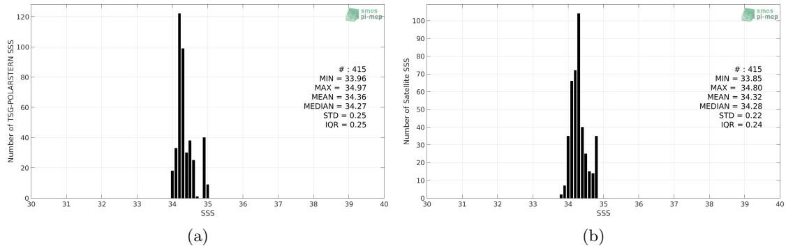
Figure 2: Histograms of SSS from TSG-POLARSTERN (a) and CCI-L4-ESA-MERGED-OI-V1.8-30DAY-RUNNING (b) considering all match-up pairs per bins of 0.1 over the South Pacific Ocean Pi-MEP region and for the full satellite product period.
