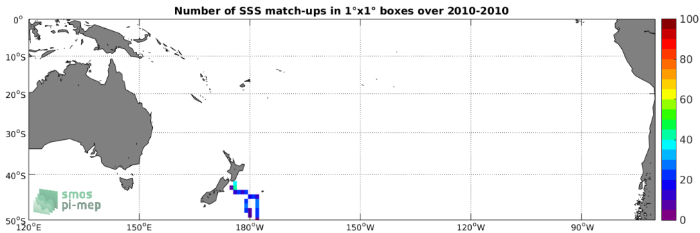
Figure 4: Number of SSS match-ups between TSG-POLARSTERN SSS and the CCI-L4-ESA-MERGED-OI-V1.8-30DAY-RUNNING SSS product for the South Pacific Ocean Pi-MEP region over 1°x1° boxes and for the full satellite product period.
