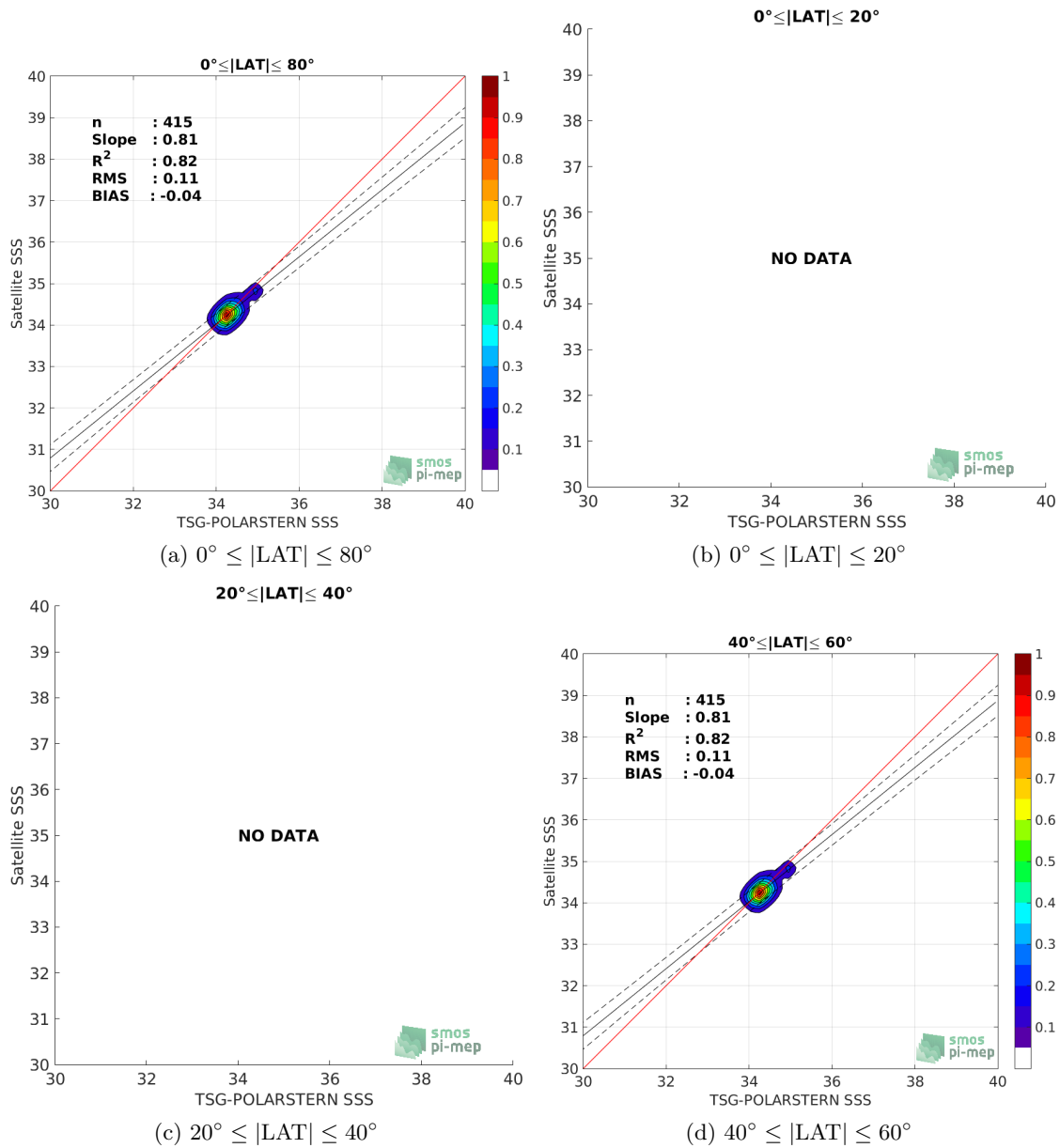
Figure 9: Contour maps of the concentration of CCI-L4-ESA-MERGED-OI-V1.8-30DAY-RUNNING SSS (y-axis) versus TSG-POLARSTERN SSS (x-axis) at match-up pairs for different latitude bands. For each plot, the red line shows x=y . The black thin and dashed lines indicate a linear fit through the data cloud and the \pm 95\% confidence levels, respectively. The number match-up pairs n , the slope and R^2 coefficient of the linear fit, the root mean square (RMS) and the mean bias between satellite and in situ data are indicated for each latitude band in each plots.
