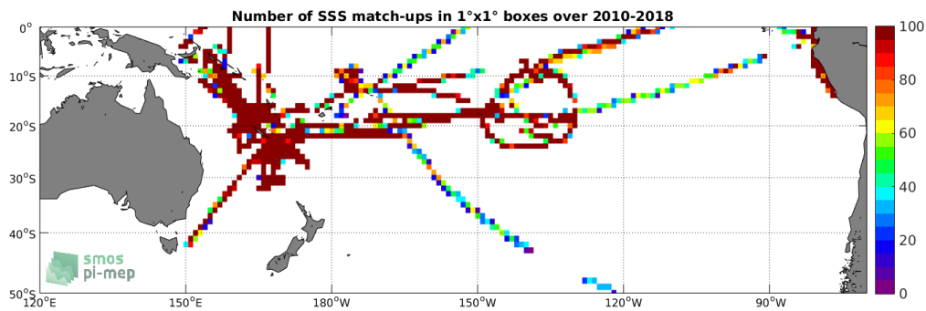
Figure 4: Number of SSS match-ups between TSG-GOSUD-Research-vessel SSS and the CCI L4 Merged-OI v1.8 - 30-day running (ESA) SSS product for the South Pacific Ocean Pi-MEP region over 1^\circ \times 1^\circ boxes and for the full satellite product period.
