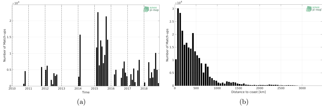
Figure 1: Number of match-ups between TSG-GOSUD-Research-vessel and CCI L4 Merged-OI v1.8 - 30-day running (ESA) SSS as a function of time (a) and as function of the distance to coast (b) over the South Pacific Ocean Pi-MEP region and for the full satellite product period.
