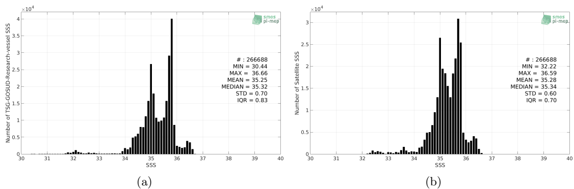
Figure 2: Histograms of SSS from TSG-GOSUD-Research-vessel (a) and CCI L4 Merged-OI v1.8 - 30-day running (ESA) (b) considering all match-up pairs per bins of 0.1 over the South Pacific Ocean Pi-MEP region and for the full satellite product period.
