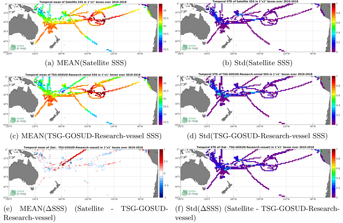
Figure 6: Temporal mean (left) and Std (right) of SSS from CCI L4 Merged-OI v1.8 - 30-day running (ESA) (top), TSG-GOSUD-Research-vessel (middle), and of \Delta SSS (Satellite - TSG-GOSUD-Research-vessel). Only match-up pairs are used to generate these maps.
