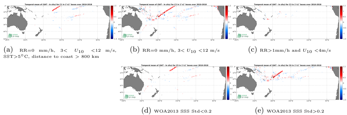
Figure 12: Temporal mean gridded over spatial boxes of size 1^\circ \times 1^\circ of \Delta SSS (CCI L4 Merged-OI v1.8 - 30-day running (ESA) - TSG-GOSUD-Research-vessel) for 5 different subdatasets corresponding to:RR=0 mm/h, 3 < U_{10} < 12 m/s, SST>5°C, distance to coast > 800 km (a), RR=0 mm/h, 3 < U_{10} < 12 m/s (b), RR>1mm/h and U_{10} < 4 m/s (c), WOA2013 SSS Std<0.2 (d), WOA2013 SSS Std>0.2 (e).
