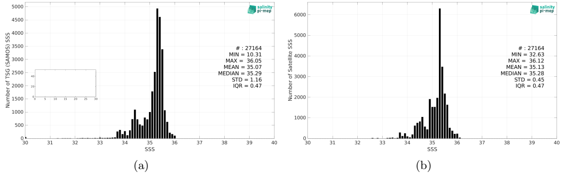
Figure 2: Histograms of SSS from TSG (SAMOS) (a) and Aquarius SSS L4 OI v5 - Weekly (IPRC) (b) considering all match-up pairs per bins of 0.1 over the South Pacific Ocean Pi-MEP region and for the full satellite product period.
