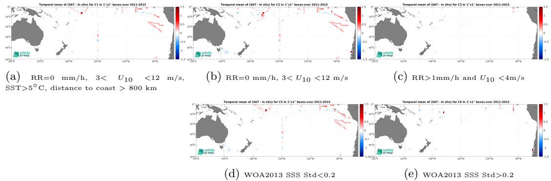
Figure 12: Temporal mean gridded over spatial boxes of size 1^\circ \times 1^\circ of \Delta SSS (Aquarius SSS L4 OI v5 - Weekly (IPRC) - TSG (SAMOS)) for 5 different subdatasets corresponding to:RR=0 mm/h, 3 < U_{10} < 12 m/s, SST >5^\circ C, distance to coast > 800 km (a), RR=0 mm/h, 3 < U_{10} < 12 m/s (b), RR >1 mm/h and U_{10} < 4 m/s (c), WOA2013 SSS Std <0.2 (d), WOA2013 SSS Std >0.2 (e).
