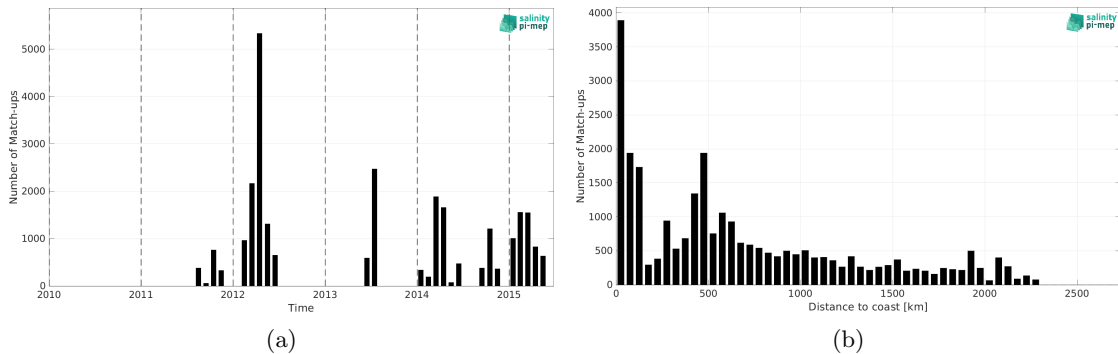
Figure 1: Number of match-ups between TSG (SAMOS) and Aquarius SSS L4 OI v5 - Weekly (IPRC) SSS as a function of time (a) and as function of the distance to coast (b) over the South Pacific Ocean Pi-MEP region and for the full satellite product period.
