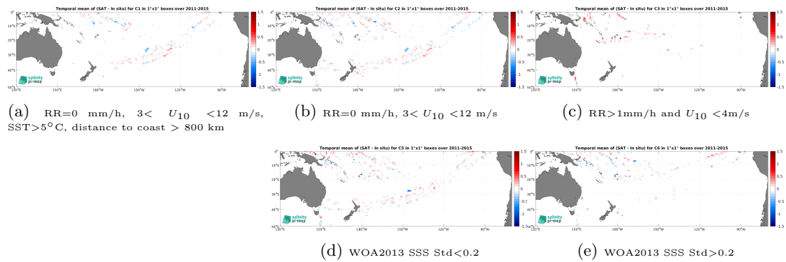
Figure 14: Temporal mean gridded over spatial boxes of size 1^\circ \times 1^\circ of \Delta\text{SSS} (Aquarius SSS L4 OI v5 - Weekly (IPRC) - TSG (LEGOS-DM)) for 5 different subdatasets corresponding to:RR=0 mm/h, 3 < U_{10} < 12 m/s, SST>5°C, distance to coast > 800 km (a), RR=0 mm/h, 3 < U_{10} < 12 m/s (b), RR>1mm/h and U_{10} < 4 m/s (c), WOA2013 SSS Std<0.2 (d), WOA2013 SSS Std>0.2 (e).
