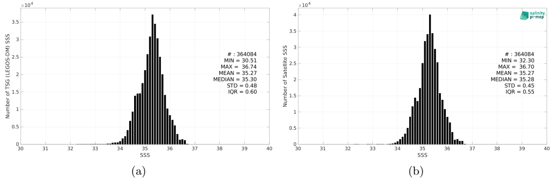
Figure 2: Histograms of SSS from TSG (LEGOS-DM) (a) and Aquarius SSS L4 OI v5 - Weekly (IPRC) (b) considering all match-up pairs per bins of 0.1 over the South Pacific Ocean Pi-MEP region and for the full satellite product period.
