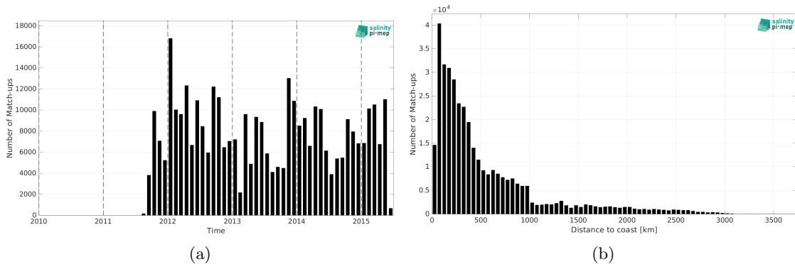
Figure 1: Number of match-ups between TSG (LEGOS-DM) and Aquarius SSS L4 OI v5 - Weekly (IPRC) SSS as a function of time (a) and as function of the distance to coast (b) over the South Pacific Ocean Pi-MEP region and for the full satellite product period.
