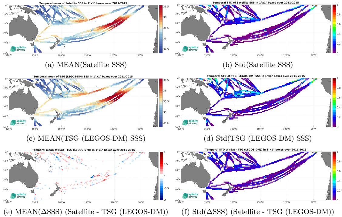
Figure 6: Temporal mean (left) and Std (right) of SSS from Aquarius SSS L4 OI v5 - Weekly (IPRC) (top), TSG (LEGOS-DM) (middle), and of \Delta SSS (Satellite - TSG (LEGOS-DM)). Only match-up pairs are used to generate these maps.
