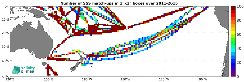
Figure 4: Number of SSS match-ups between TSG (LEGOS-DM) SSS and the Aquarius SSS L4 OI v5 - Weekly (IPRC) SSS product for the South Pacific Ocean Pi-MEP region over 1^\circ \times 1^\circ boxes and for the full satellite product period.
