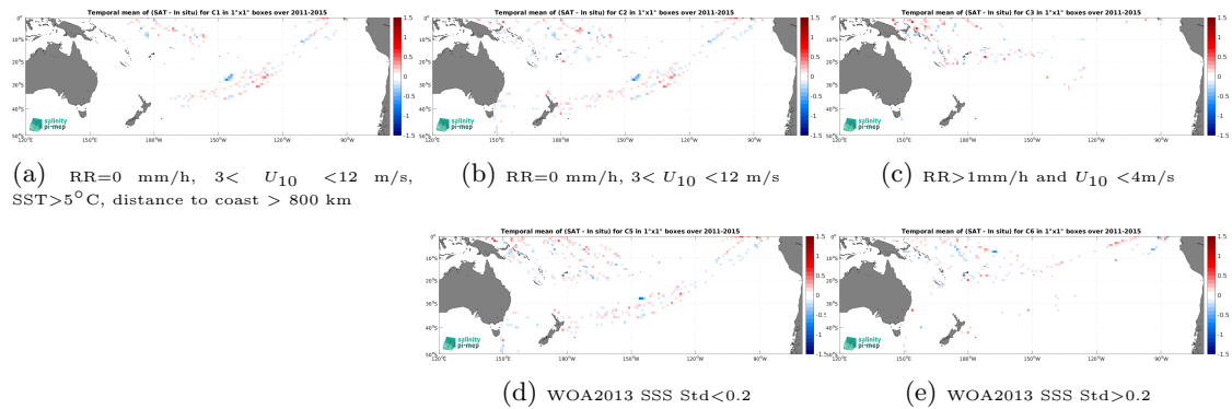
Figure 12: Temporal mean gridded over spatial boxes of size 1^\circ \times 1^\circ of \Delta SSS (Aquarius SSS L4 OI v5 - Weekly (IPRC) - TSG (LEGOS-DM)) for 5 different subdatasets corresponding to:RR=0 mm/h, 3 < U_{10} < 12 m/s, SST >5^\circ\text{C} , distance to coast > 800 km (a), RR=0 mm/h, 3 < U_{10} < 12 m/s (b), RR >1 mm/h and U_{10} < 4 m/s (c), WOA2013 SSS Std <0.2 (d), WOA2013 SSS Std >0.2 (e).
