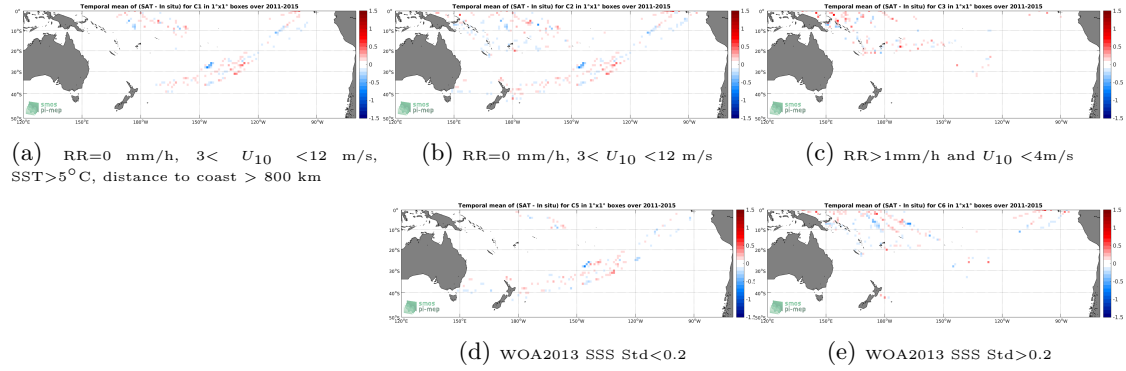
Figure 12: Temporal mean gridded over spatial boxes of size 1^\circ \times 1^\circ of \Delta SSS (Aquarius-L4-IPRC-V5-WEEKLY - TSG-LEGOS-DM) for 5 different subdatasets corresponding to: RR=0 mm/h, 3 < U_{10} < 12 m/s, SST >5^\circ\text{C} , distance to coast > 800 km (a), RR=0 mm/h, 3 < U_{10} < 12 m/s (b), RR >1 mm/h and U_{10} < 4 m/s (c), WOA2013 SSS Std <0.2 (d), WOA2013 SSS Std >0.2 (e).
