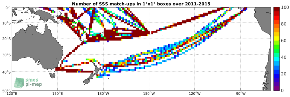
Figure 4: Number of SSS match-ups between TSG-LEGOS-DM SSS and the Aquarius-L4-IPRC-V5-WEEKLY SSS product for the South Pacific Ocean Pi-MEP region over 1^\circ \times 1^\circ boxes and for the full satellite product period.
