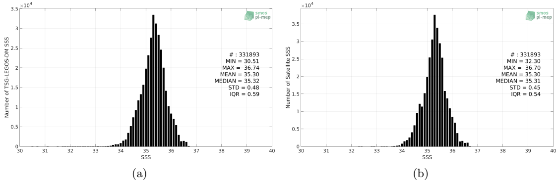
Figure 2: Histograms of SSS from TSG-LEGOS-DM (a) and Aquarius-L4-IPRC-V5-WEEKLY (b) considering all match-up pairs per bins of 0.1 over the South Pacific Ocean Pi-MEP region and for the full satellite product period.
