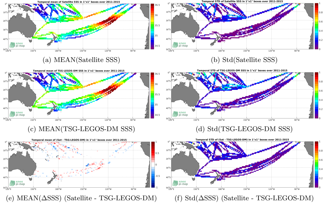
Figure 6: Temporal mean (left) and Std (right) of SSS from Aquarius-L4-IPRC-V5-WEEKLY (top), TSG-LEGOS-DM (middle), and of \Delta SSS (Satellite - TSG-LEGOS-DM). Only match-up pairs are used to generate these maps.
