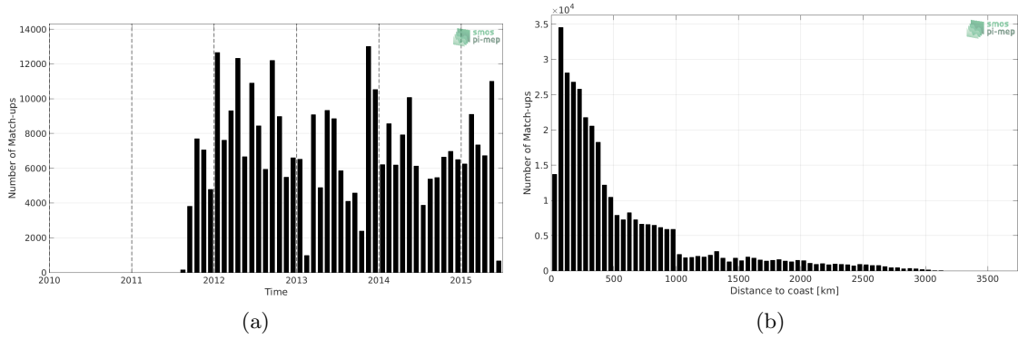
Figure 1: Number of match-ups between TSG-LEGOS-DM and Aquarius-L4-IPRC-V5-WEEKLY SSS as a function of time (a) and as function of the distance to coast (b) over the South Pacific Ocean Pi-MEP region and for the full satellite product period.
