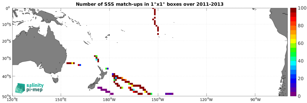
Figure 5: Number of SSS match-ups between TSG (GOSUD-Sailing-ship) SSS and the Aquarius SSS L4 OI v5 - Weekly (IPRC) SSS product for the South Pacific Ocean Pi-MEP region over 1^\circ \times 1^\circ boxes and for the full satellite product period.
