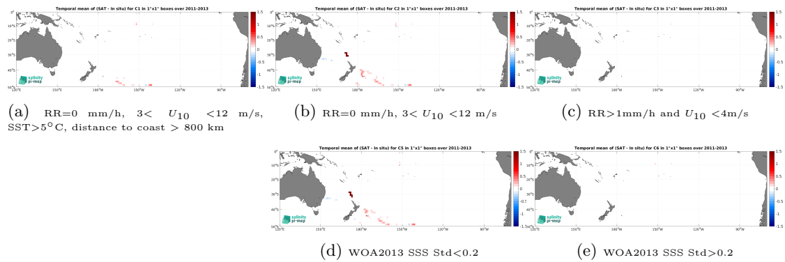
Figure 14: Temporal mean gridded over spatial boxes of size 1^\circ \times 1^\circ of \Delta SSS (Aquarius SSS L4 OI v5 - Weekly (IPRC) - TSG (GOSUD-Sailing-ship)) for 5 different subdatasets corresponding to:RR=0 mm/h, 3 < U_{10} < 12 m/s, SST>5°C, distance to coast > 800 km (a), RR=0 mm/h, 3 < U_{10} < 12 m/s (b), RR>1mm/h and U_{10} < 4 m/s (c), WOA2013 SSS Std<0.2 (d), WOA2013 SSS Std>0.2 (e).
