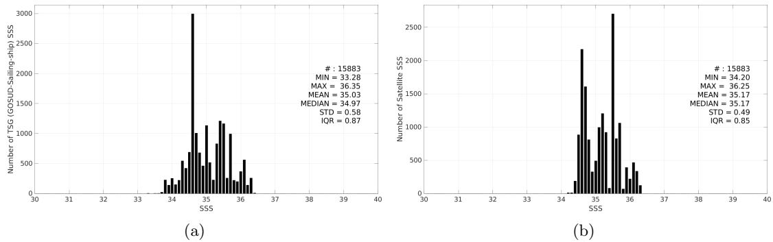
Figure 3: Histograms of SSS from TSG (GOSUD-Sailing-ship) (a) and Aquarius SSS L4 OI v5 - Weekly (IPRC) (b) considering all match-up pairs per bins of 0.1 over the South Pacific Ocean Pi-MEP region and for the full satellite product period.
