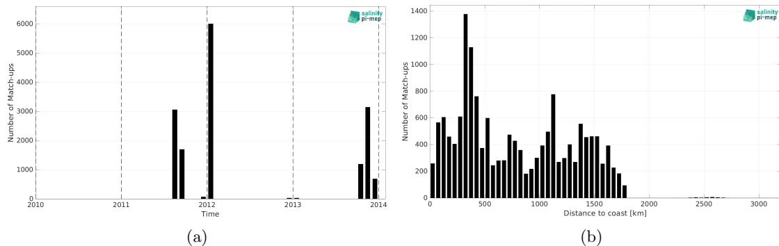
Figure 2: Number of match-ups between TSG (GOSUD-Sailing-ship) and Aquarius SSS L4 OI v5 - Weekly (IPRC) SSS as a function of time (a) and as function of the distance to coast (b) over the South Pacific Ocean Pi-MEP region and for the full satellite product period.
