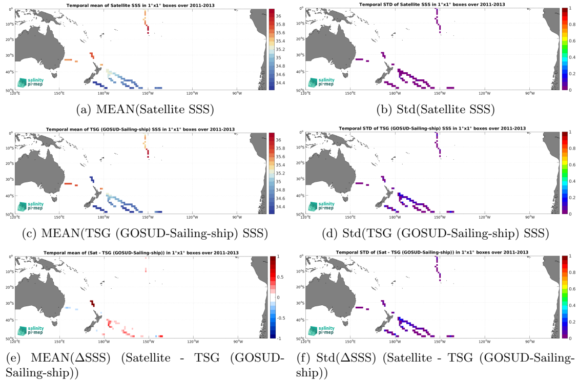
Figure 7: Temporal mean (left) and Std (right) of SSS from Aquarius SSS L4 OI v5 - Weekly (IPRC) (top), TSG (GOSUD-Sailing-ship) (middle), and of \Delta SSS (Satellite - TSG (GOSUD-Sailing-ship)). Only match-up pairs are used to generate these maps.
