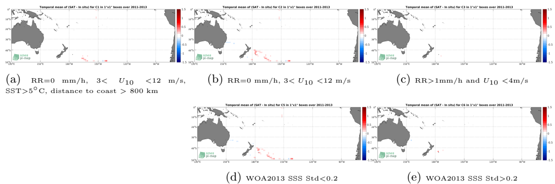
Figure 12: Temporal mean gridded over spatial boxes of size 1^\circ \times 1^\circ of \Delta\text{SSS} (Aquarius SSS L4 OI v5 - Weekly (IPRC) - TSG (GOSUD-Sailing-ship)) for 5 different subdatasets corresponding to: RR=0 mm/h, 3 < U_{10} < 12 m/s, SST > 5°C, distance to coast > 800 km (a), RR=0 mm/h, 3 < U_{10} < 12 m/s (b), RR > 1mm/h and U_{10} < 4 m/s (c), WOA2013 SSS Std < 0.2 (d), WOA2013 SSS Std > 0.2 (e).
