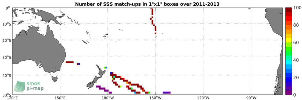
Figure 4: Number of SSS match-ups between TSG (GOSUD-Sailing-ship) SSS and the Aquarius SSS L4 OI v5 - Weekly (IPRC) SSS product for the South Pacific Ocean Pi-MEP region over 1^\circ \times 1^\circ boxes and for the full satellite product period.
