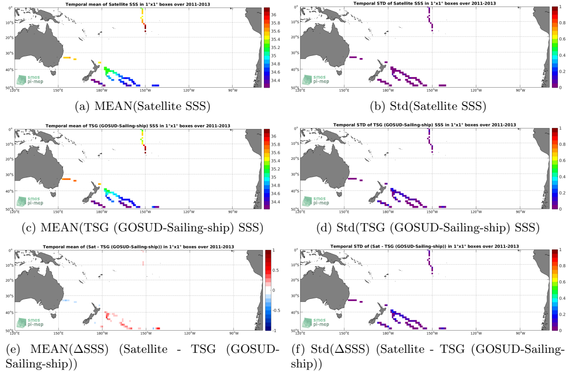
Figure 6: Temporal mean (left) and Std (right) of SSS from Aquarius SSS L4 OI v5 - Weekly (IPRC) (top), TSG (GOSUD-Sailing-ship) (middle), and of \Delta SSS (Satellite - TSG (GOSUD-Sailing-ship)). Only match-up pairs are used to generate these maps.
