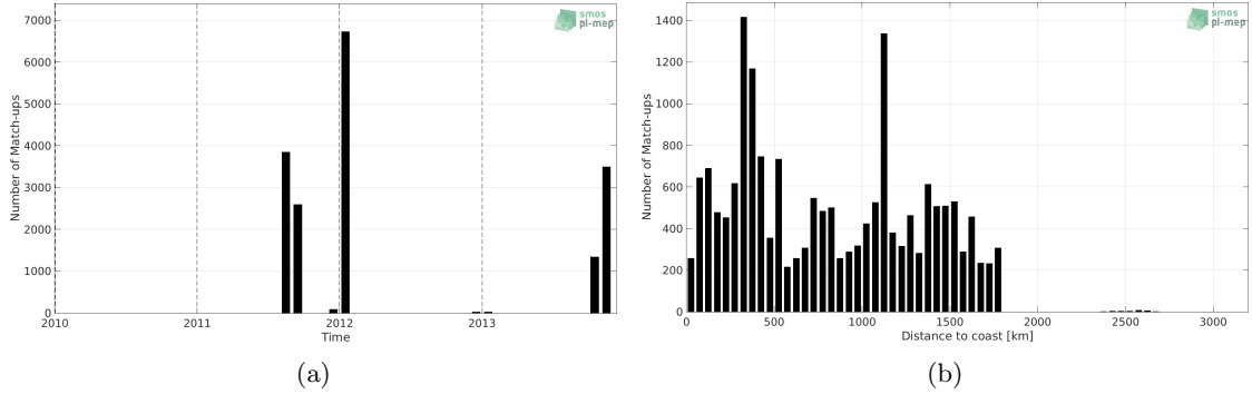
Figure 1: Number of match-ups between TSG (GOSUD-Sailing-ship) and Aquarius SSS L4 OI v5 - Weekly (IPRC) SSS as a function of time (a) and as function of the distance to coast (b) over the South Pacific Ocean Pi-MEP region and for the full satellite product period.
