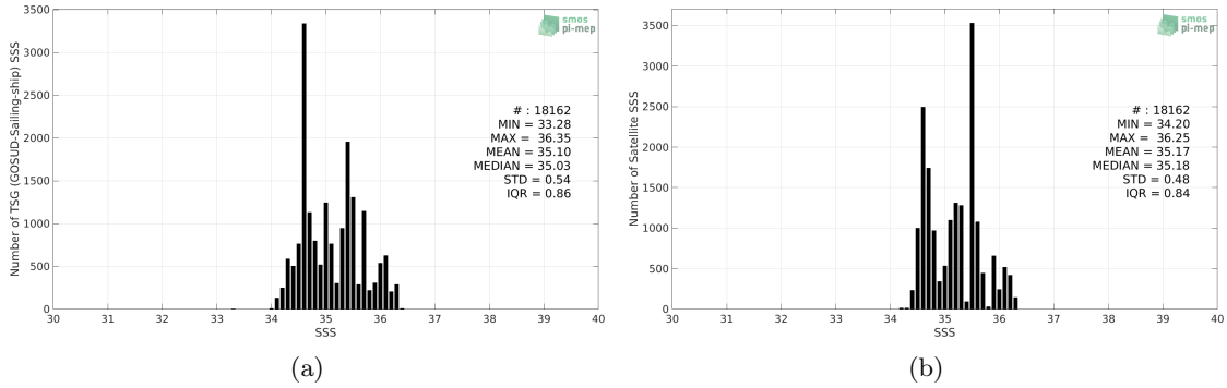
Figure 2: Histograms of SSS from TSG (GOSUD-Sailing-ship) (a) and Aquarius SSS L4 OI v5 - Weekly (IPRC) (b) considering all match-up pairs per bins of 0.1 over the South Pacific Ocean Pi-MEP region and for the full satellite product period.
