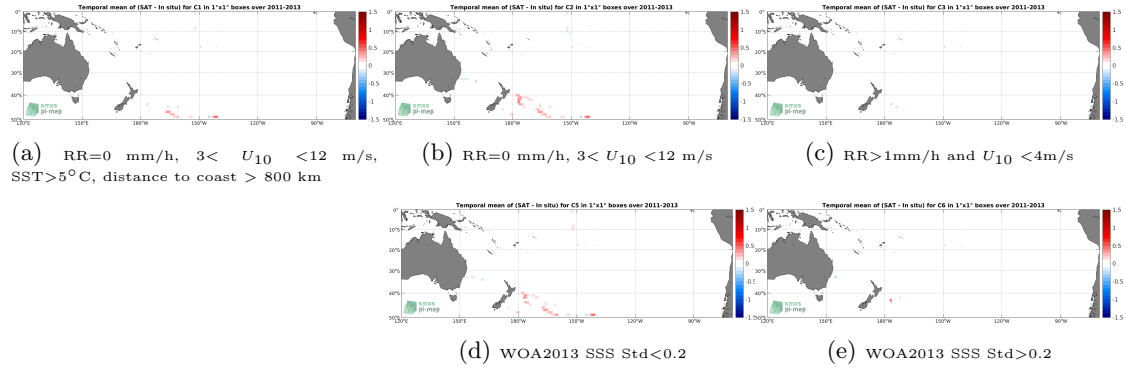
Figure 12: Temporal mean gridded over spatial boxes of size 1^\circ \times 1^\circ of \Delta SSS (Aquarius SSS L4 OI v5 - Weekly (IPRC) - TSG (GOSUD-Sailing-ship)) for 5 different subdatasets corresponding to: RR=0 mm/h, 3 < U_{10} < 12 m/s, SST >5^\circ\text{C} , distance to coast > 800 km (a), RR=0 mm/h, 3 < U_{10} < 12 m/s (b), RR>1\text{mm/h} and U_{10} < 4\text{m/s} (c), WOA2013 SSS Std <0.2 (d), WOA2013 SSS Std >0.2 (e).
