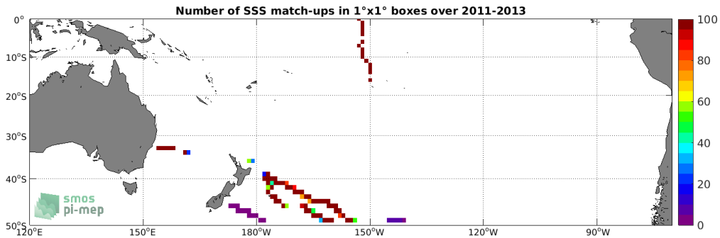
Figure 4: Number of SSS match-ups between TSG (GOSUD-Sailing-ship) SSS and the Aquarius SSS L4 OI v5 - Weekly (IPRC) SSS product for the South Pacific Ocean Pi-MEP region over 1°x1° boxes and for the full satellite product period.
