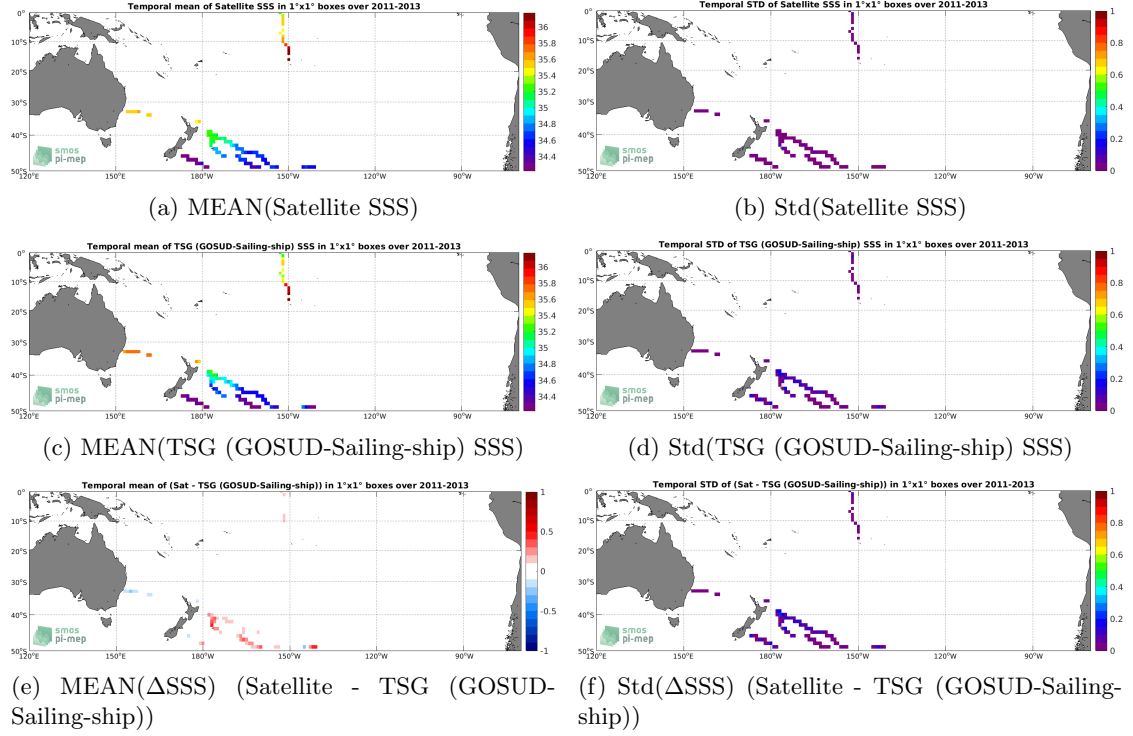
Figure 6: Temporal mean (left) and Std (right) of SSS from Aquarius SSS L4 OI v5 - Weekly (IPRC) (top), TSG (GOSUD-Sailing-ship) (middle), and of \Delta SSS (Satellite - TSG (GOSUD-Sailing-ship)). Only match-up pairs are used to generate these maps.
