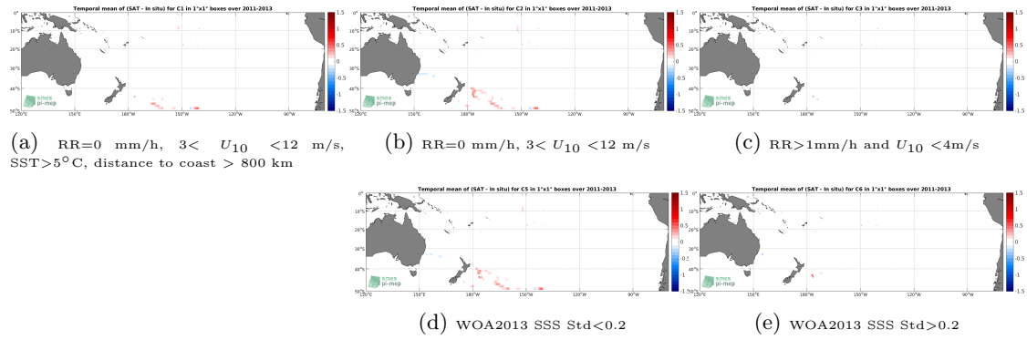
Figure 12: Temporal mean gridded over spatial boxes of size 1^\circ \times 1^\circ of \Delta SSS (Aquarius-L4-IPRC-V5-WEEKLY - TSG-GOSUD-Sailing-ship) for 5 different subdatasets corresponding to: RR=0 mm/h, 3 < U_{10} < 12 m/s, SST > 5^\circ C , distance to coast > 800 km (a), RR=0 mm/h, 3 < U_{10} < 12 m/s (b), RR > 1 mm/h and U_{10} < 4 m/s (c), WOA2013 SSS Std < 0.2 (d), WOA2013 SSS Std > 0.2 (e).
