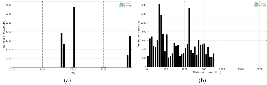
Figure 1: Number of match-ups between TSG-GOSUD-Sailing-ship and Aquarius-L4-IPRC-V5-WEEKLY SSS as a function of time (a) and as function of the distance to coast (b) over the South Pacific Ocean Pi-MEP region and for the full satellite product period.
