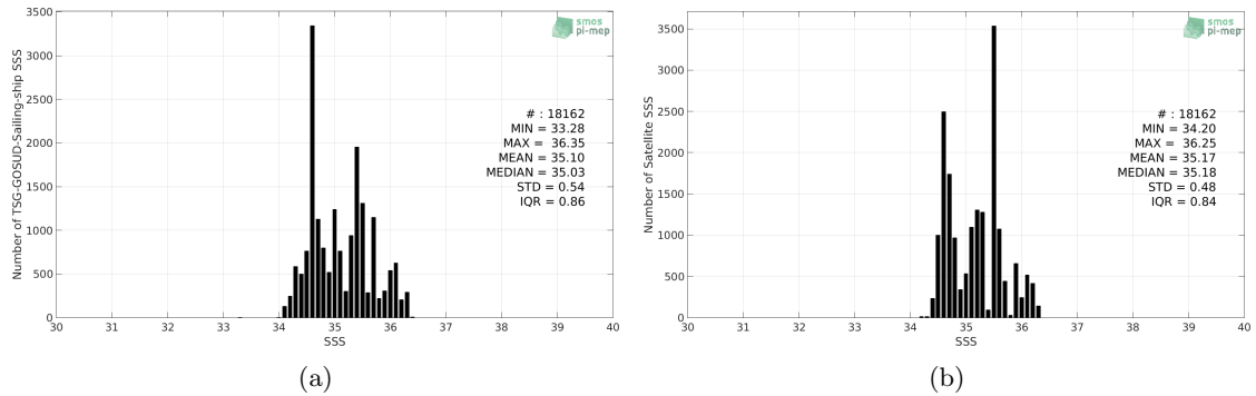
Figure 2: Histograms of SSS from TSG-GOSUD-Sailing-ship (a) and Aquarius-L4-IPRC-V5-WEEKLY (b) considering all match-up pairs per bins of 0.1 over the South Pacific Ocean Pi-MEP region and for the full satellite product period.
