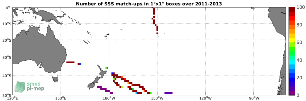
Figure 4: Number of SSS match-ups between TSG-GOSUD-Sailing-ship SSS and the Aquarius-L4-IPRC-V5-WEEKLY SSS product for the South Pacific Ocean Pi-MEP region over 1^\circ \times 1^\circ boxes and for the full satellite product period.
