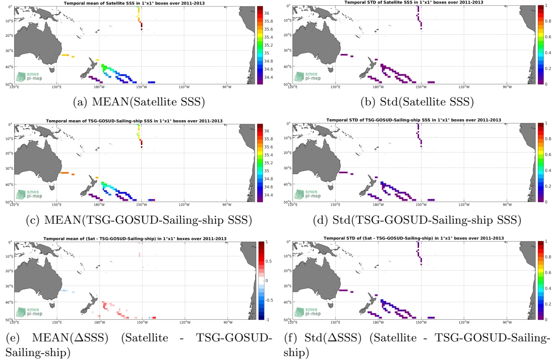
Figure 6: Temporal mean (left) and Std (right) of SSS from Aquarius-L4-IPRC-V5-WEEKLY (top), TSG-GOSUD-Sailing-ship (middle), and of \Delta SSS (Satellite - TSG-GOSUD-Sailing-ship). Only match-up pairs are used to generate these maps.
