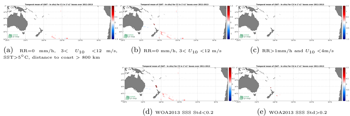
Figure 12: Temporal mean gridded over spatial boxes of size 1^\circ \times 1^\circ of \Delta SSS (Aquarius-L4-IPRC-V5-WEEKLY - TSG-GOSUD-Sailing-ship) for 5 different subdatasets corresponding to:RR=0 mm/h, 3 < U_{10} < 12 m/s, SST >5^\circ C, distance to coast > 800 km (a), RR=0 mm/h, 3 < U_{10} < 12 m/s (b), RR >1 mm/h and U_{10} < 4 m/s (c), WOA2013 SSS Std <0.2 (d), WOA2013 SSS Std >0.2 (e).
