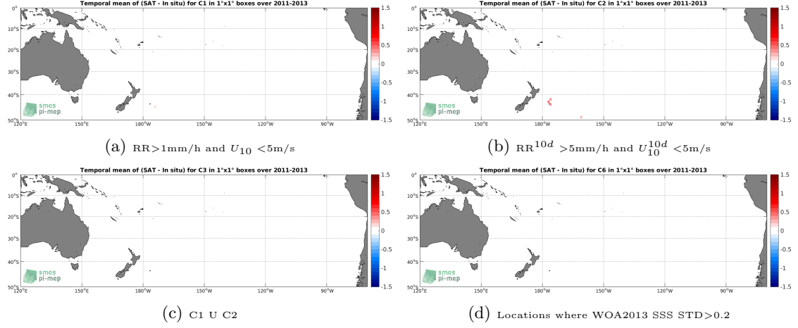
Figure 12: Temporal mean gridded over spatial boxes of size 1^\circ \times 1^\circ of \Delta SSS (Aquarius-L4-IPRC-V5-WEEKLY - TSG-GOSUD-Sailing-ship) for 4 different subdatasets corresponding to: RR > 1mm/h and U_{10} < 5\text{m/s} (a), RR^{10d} > 5\text{mm/h} and U_{10}^{10d} < 5\text{m/s} (b), C1 U C2 (c), Locations where WOA2013 SSS STD > 0.2 (d).
