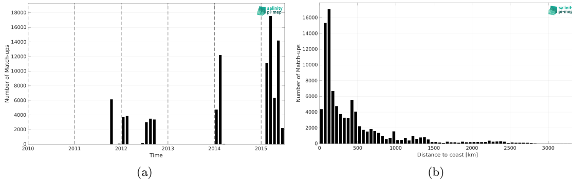
Figure 2: Number of match-ups between TSG (GOSUD-Research-vessel) and Aquarius SSS L4 OI v5 - Weekly (IPRC) SSS as a function of time (a) and as function of the distance to coast (b) over the South Pacific Ocean Pi-MEP region and for the full satellite product period.
