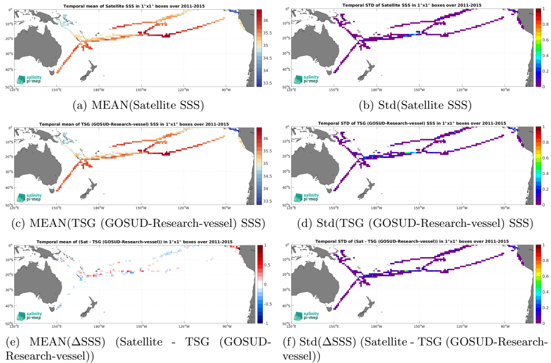
Figure 7: Temporal mean (left) and Std (right) of SSS from Aquarius SSS L4 OI v5 - Weekly (IPRC) (top), TSG (GOSUD-Research-vessel) (middle), and of \Delta SSS (Satellite - TSG (GOSUD-Research-vessel)). Only match-up pairs are used to generate these maps.
