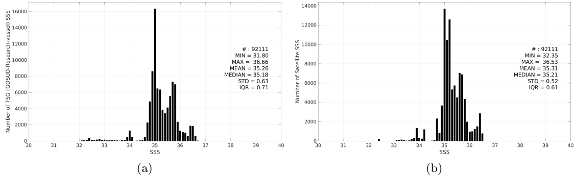
Figure 3: Histograms of SSS from TSG (GOSUD-Research-vessel) (a) and Aquarius SSS L4 OI v5 - Weekly (IPRC) (b) considering all match-up pairs per bins of 0.1 over the South Pacific Ocean Pi-MEP region and for the full satellite product period.
