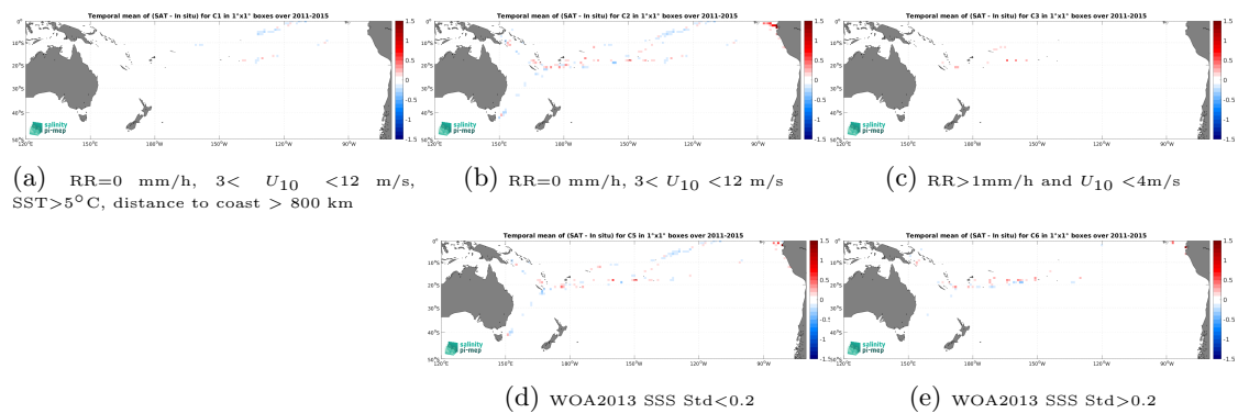
Figure 14: Temporal mean gridded over spatial boxes of size 1^\circ \times 1^\circ of \Delta SSS (Aquarius SSS L4 OI v5 - Weekly (IPRC) - TSG (GOSUD-Research-vessel)) for 5 different subdatasets corresponding to:RR=0 mm/h, 3 < U_{10} < 12 m/s, SST >5^\circ\text{C} , distance to coast > 800 km (a), RR=0 mm/h, 3 < U_{10} < 12 m/s (b), RR >1 mm/h and U_{10} < 4 m/s (c), WOA2013 SSS Std <0.2 (d), WOA2013 SSS Std >0.2 (e).
