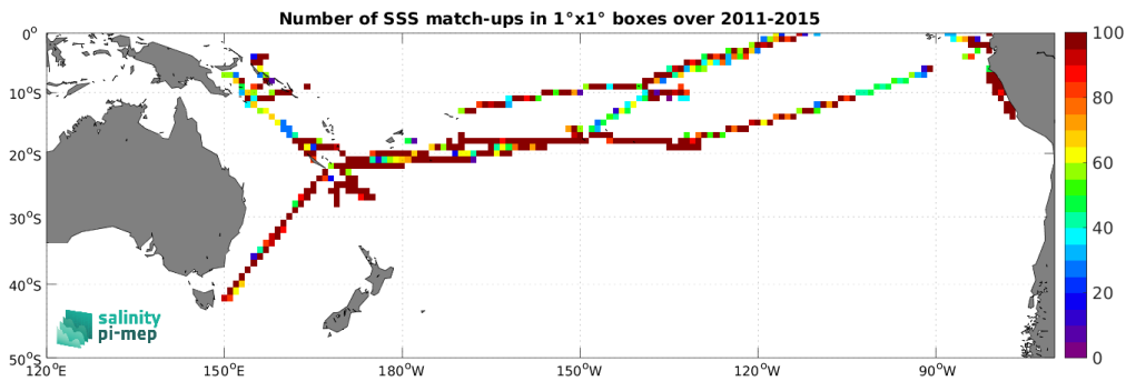
Figure 5: Number of SSS match-ups between TSG (GOSUD-Research-vessel) SSS and the Aquarius SSS L4 OI v5 - Weekly (IPRC) SSS product for the South Pacific Ocean Pi-MEP region over 1^\circ \times 1^\circ boxes and for the full satellite product period.
