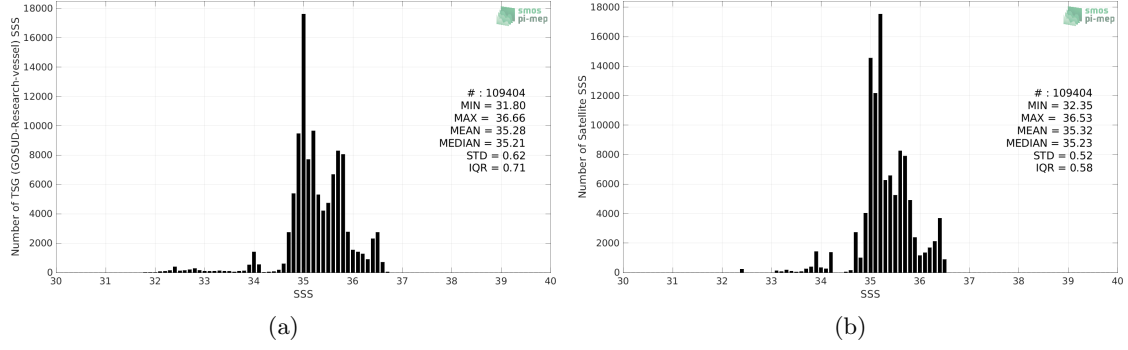
Figure 2: Histograms of SSS from TSG (GOSUD-Research-vessel) (a) and Aquarius SSS L4 OI v5 - Weekly (IPRC) (b) considering all match-up pairs per bins of 0.1 over the South Pacific Ocean Pi-MEP region and for the full satellite product period.
