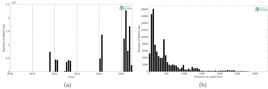
Figure 1: Number of match-ups between TSG (GOSUD-Research-vessel) and Aquarius SSS L4 OI v5 - Weekly (IPRC) SSS as a function of time (a) and as function of the distance to coast (b) over the South Pacific Ocean Pi-MEP region and for the full satellite product period.
