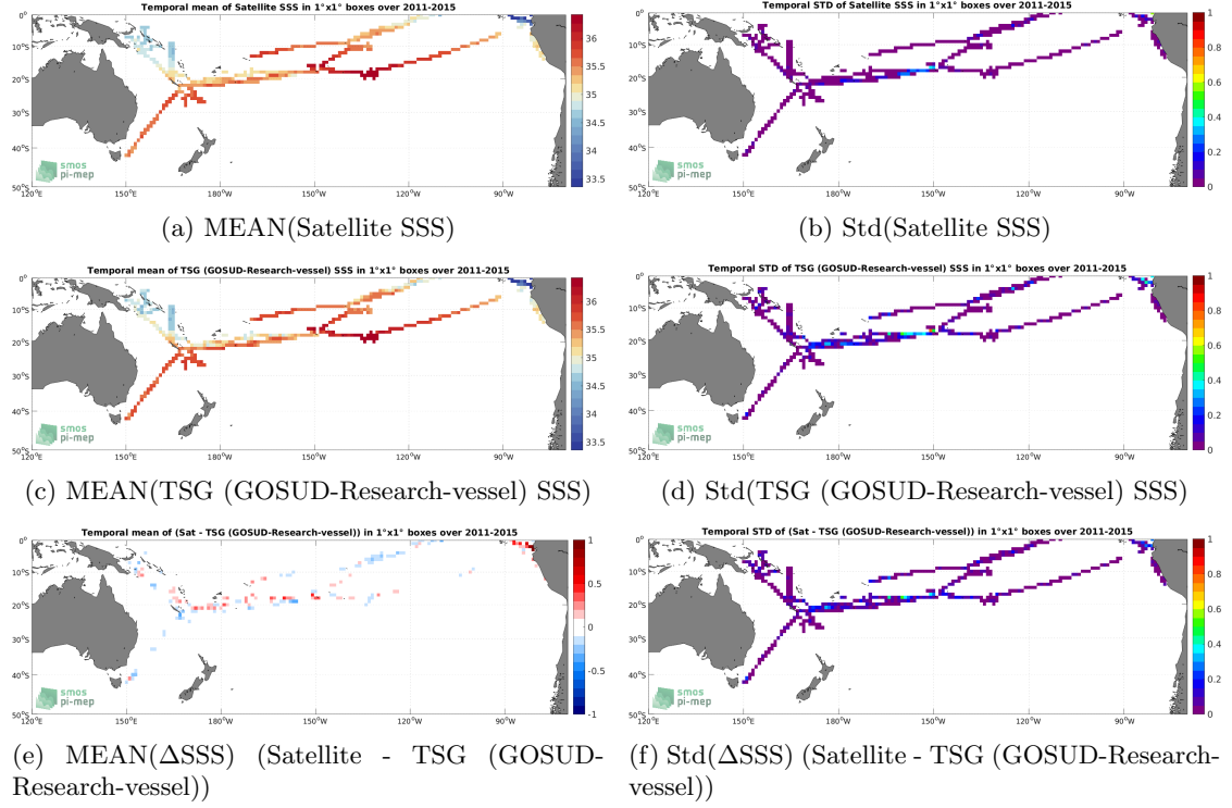
Figure 6: Temporal mean (left) and Std (right) of SSS from Aquarius SSS L4 OI v5 - Weekly (IPRC) (top), TSG (GOSUD-Research-vessel) (middle), and of \Delta SSS (Satellite - TSG (GOSUD-Research-vessel)). Only match-up pairs are used to generate these maps.
