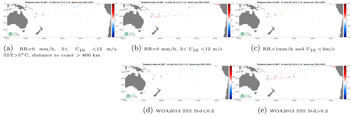
Figure 12: Temporal mean gridded over spatial boxes of size 1^\circ \times 1^\circ of \Delta SSS (Aquarius SSS L4 OI v5 - Weekly (IPRC) - TSG (GOSUD-Research-vessel)) for 5 different subdatasets corresponding to: RR=0 mm/h, 3 < U_{10} < 12 m/s, SST > 5^\circ C , distance to coast > 800 km (a), RR=0 mm/h, 3 < U_{10} < 12 m/s (b), RR > 1 mm/h and U_{10} < 4 m/s (c), WOA2013 SSS Std < 0.2 (d), WOA2013 SSS Std > 0.2 (e).
