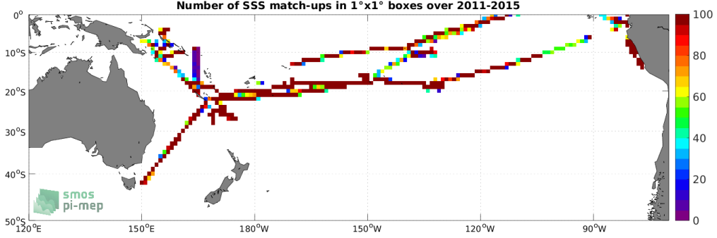
Figure 4: Number of SSS match-ups between TSG (GOSUD-Research-vessel) SSS and the Aquarius SSS L4 OI v5 - Weekly (IPRC) SSS product for the South Pacific Ocean Pi-MEP region over 1^\circ \times 1^\circ boxes and for the full satellite product period.
