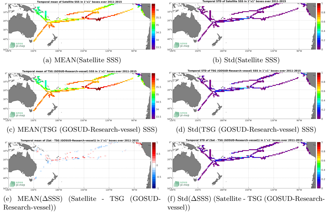
Figure 6: Temporal mean (left) and Std (right) of SSS from Aquarius SSS L4 OI v5 - Weekly (IPRC) (top), TSG (GOSUD-Research-vessel) (middle), and of \Delta SSS (Satellite - TSG (GOSUD-Research-vessel)). Only match-up pairs are used to generate these maps.
