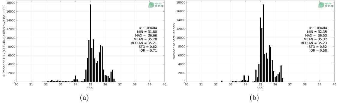
Figure 2: Histograms of SSS from TSG (GOSUD-Research-vessel) (a) and Aquarius SSS L4 OI v5 - Weekly (IPRC) (b) considering all match-up pairs per bins of 0.1 over the South Pacific Ocean Pi-MEP region and for the full satellite product period.
