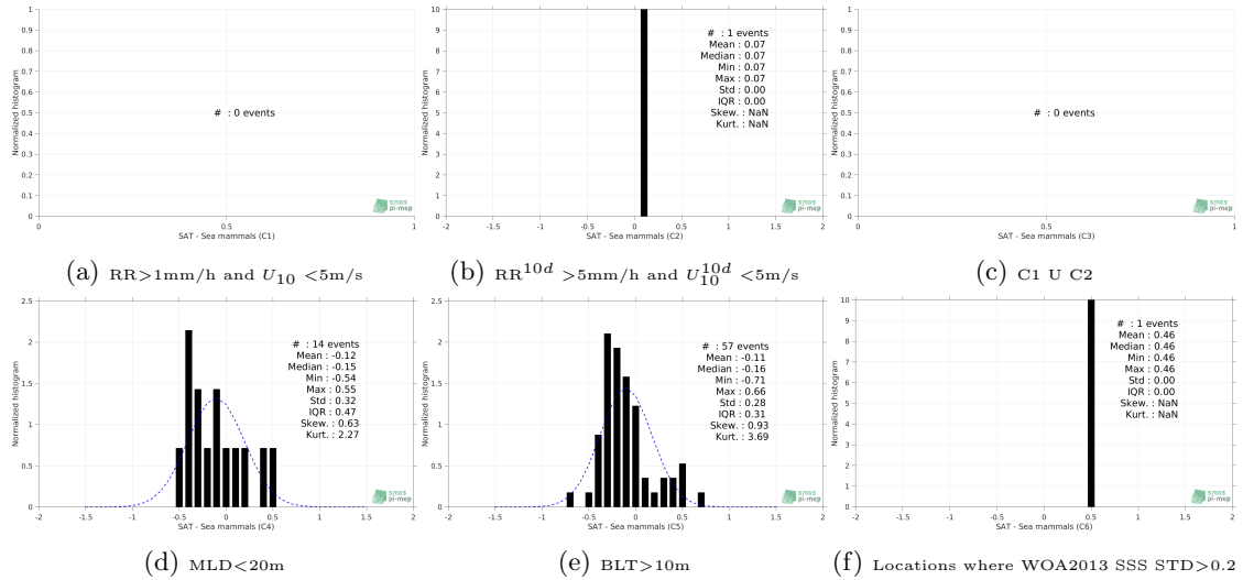
Figure 13: Normalized histogram of \Delta SSS (Aquarius-L4-IPRC-V5-WEEKLY - Sea mammals) for 6 different subdatasets corresponding to: RR>1\text{mm/h} and U_{10}<5\text{m/s} (a), RR^{10d}>5\text{mm/h} and U_{10}^{10d}<5\text{m/s} (b), C1 U C2 (c), MLD<20\text{m} (d), BLT>10\text{m} (e), Locations where WOA2013 SSS STD>0.2 (f).
