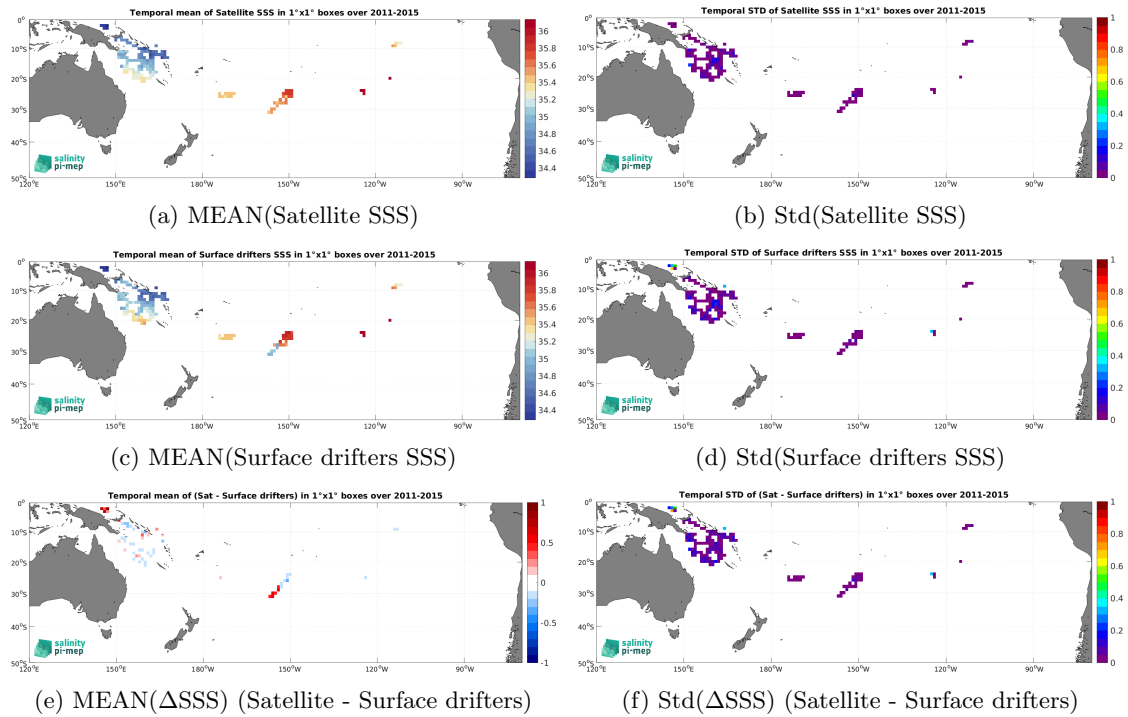
Figure 6: Temporal mean (left) and Std (right) of SSS from Aquarius SSS L4 OI v5 - Weekly (IPRC) (top), Surface drifters (middle), and of \Delta SSS (Satellite - Surface drifters). Only match-up pairs are used to generate these maps.
