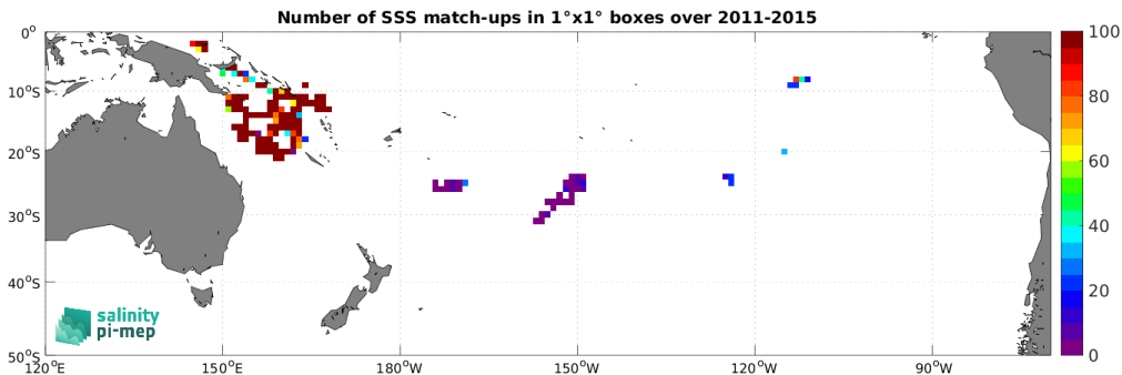
Figure 4: Number of SSS match-ups between Surface drifters SSS and the Aquarius SSS L4 OI v5 - Weekly (IPRC) SSS product for the South Pacific Ocean Pi-MEP region over 1^\circ \times 1^\circ boxes and for the full satellite product period.
