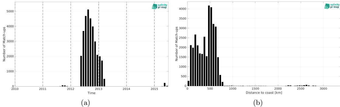
Figure 2: Number of match-ups between Surface drifters and Aquarius SSS L4 OI v5 - Weekly (IPRC) SSS as a function of time (a) and as function of the distance to coast (b) over the South Pacific Ocean Pi-MEP region and for the full satellite product period.
