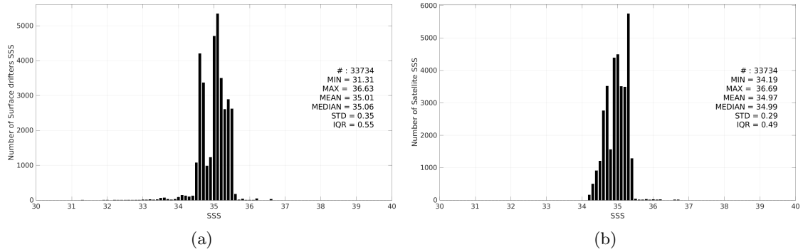
Figure 3: Histograms of SSS from Surface drifters (a) and Aquarius SSS L4 OI v5 - Weekly (IPRC) (b) considering all match-up pairs per bins of 0.1 over the South Pacific Ocean Pi-MEP region and for the full satellite product period.
