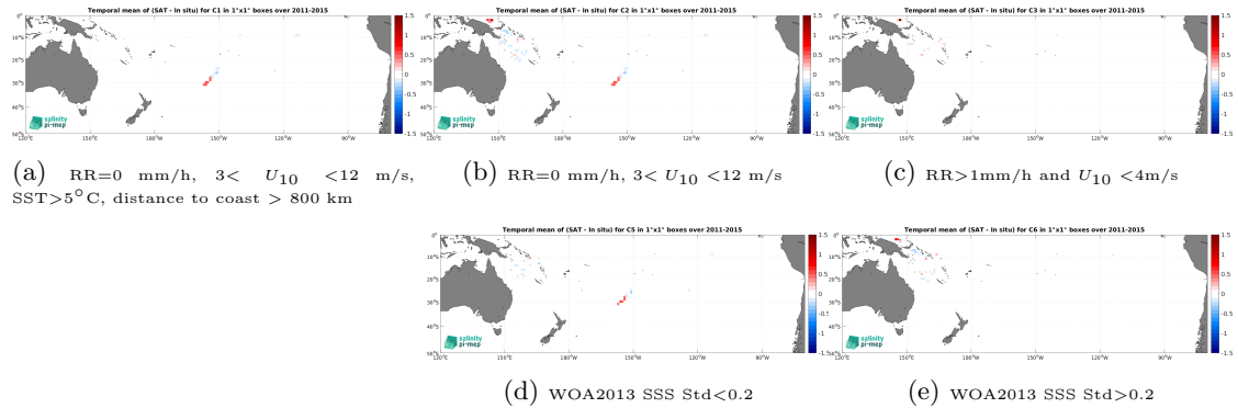
Figure 13: Temporal mean gridded over spatial boxes of size 1^\circ \times 1^\circ of \Delta SSS (Aquarius SSS L4 OI v5 - Weekly (IPRC) - Surface drifters) for 5 different subdatasets corresponding to:RR=0 mm/h, 3 < U_{10} < 12 m/s, SST >5^\circ\text{C} , distance to coast > 800 km (a), RR=0 mm/h, 3 < U_{10} < 12 m/s (b), RR >1 mm/h and U_{10} < 4 m/s (c), WOA2013 SSS Std <0.2 (d), WOA2013 SSS Std >0.2 (e).
