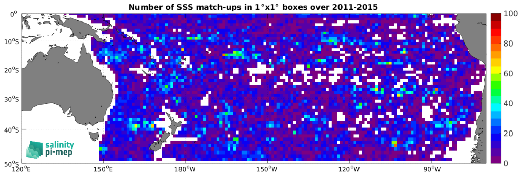
Figure 5: Number of SSS match-ups between Argo SSS and the Aquarius SSS L4 OI v5 - Weekly (IPRC) SSS product for the South Pacific Ocean Pi-MEP region over 1^\circ \times 1^\circ boxes and for the full satellite product period.
