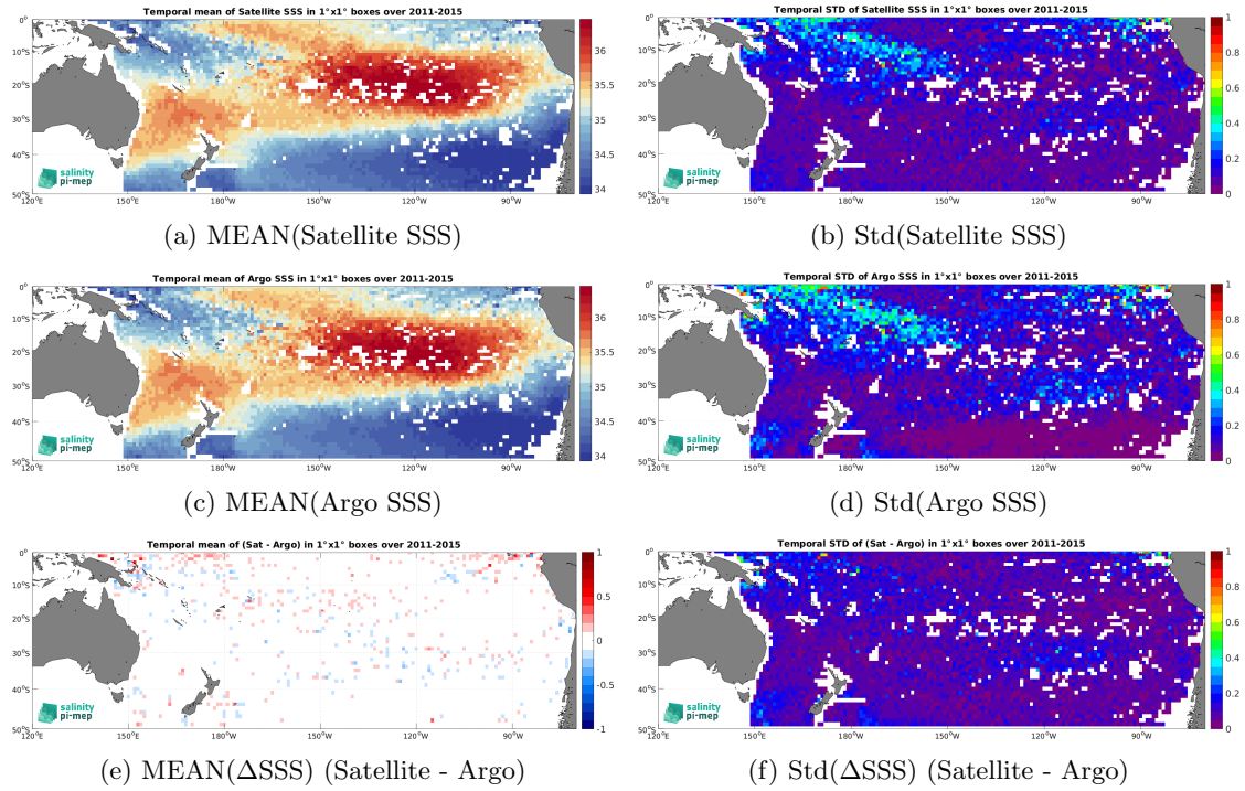
Figure 7: Temporal mean (left) and Std (right) of SSS from Aquarius SSS L4 OI v5 - Weekly (IPRC) (top), Argo (middle), and of \Delta SSS (Satellite - Argo). Only match-up pairs are used to generate these maps.
