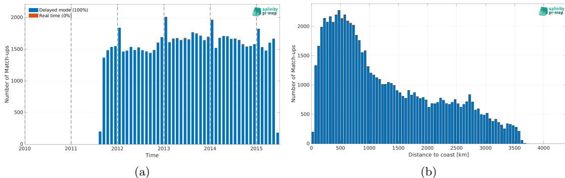
Figure 2: Number of match-ups between Argo and Aquarius SSS L4 OI v5 - Weekly (IPRC) SSS as a function of time (a) and as function of the distance to coast (b) over the South Pacific Ocean Pi-MEP region and for the full satellite product period.
