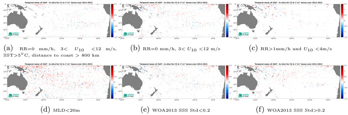
Figure 14: Temporal mean gridded over spatial boxes of size 1^\circ \times 1^\circ of \Delta SSS (Aquarius SSS L4 OI v5 - Weekly (IPRC) - Argo) for 6 different subdatasets corresponding to:RR=0 mm/h, 3 < U_{10} < 12 m/s, SST >5^\circ\text{C} , distance to coast > 800 km (a), RR=0 mm/h, 3 < U_{10} < 12 m/s (b), RR >1 mm/h and U_{10} < 4 m/s (c),MLD <20 m (d),WOA2013 SSS Std <0.2 (e),WOA2013 SSS Std >0.2 (f).
