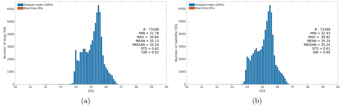
Figure 3: Histograms of SSS from Argo (a) and Aquarius SSS L4 OI v5 - Weekly (IPRC) (b) considering all match-up pairs per bins of 0.1 over the South Pacific Ocean Pi-MEP region and for the full satellite product period.
