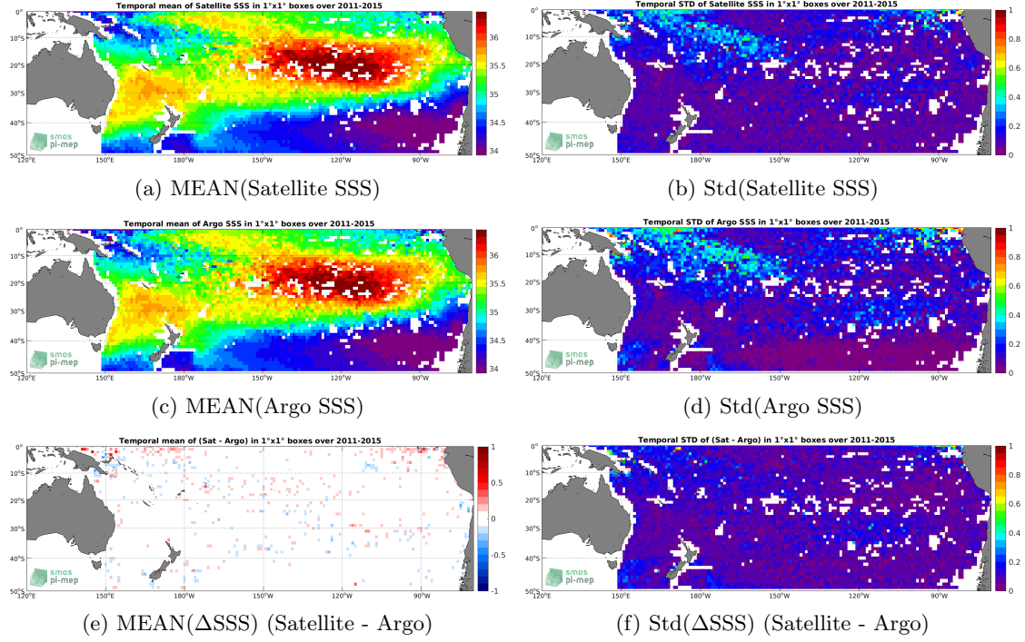
Figure 6: Temporal mean (left) and Std (right) of SSS from Aquarius SSS L4 OI v5 - Weekly (IPRC) (top), Argo (middle), and of \Delta SSS (Satellite - Argo). Only match-up pairs are used to generate these maps.
