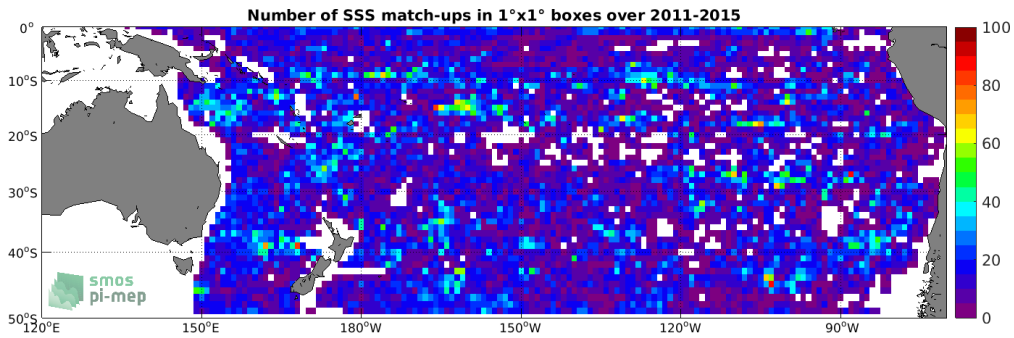
Figure 4: Number of SSS match-ups between Argo SSS and the Aquarius SSS L4 OI v5 - Weekly (IPRC) SSS product for the South Pacific Ocean Pi-MEP region over 1^\circ \times 1^\circ boxes and for the full satellite product period.
