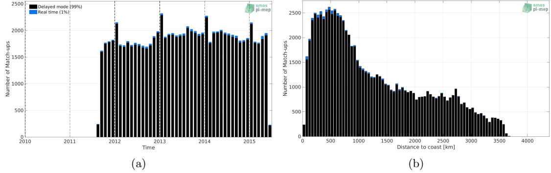
Figure 1: Number of match-ups between Argo and Aquarius SSS L4 OI v5 - Weekly (IPRC) SSS as a function of time (a) and as function of the distance to coast (b) over the South Pacific Ocean Pi-MEP region and for the full satellite product period.
