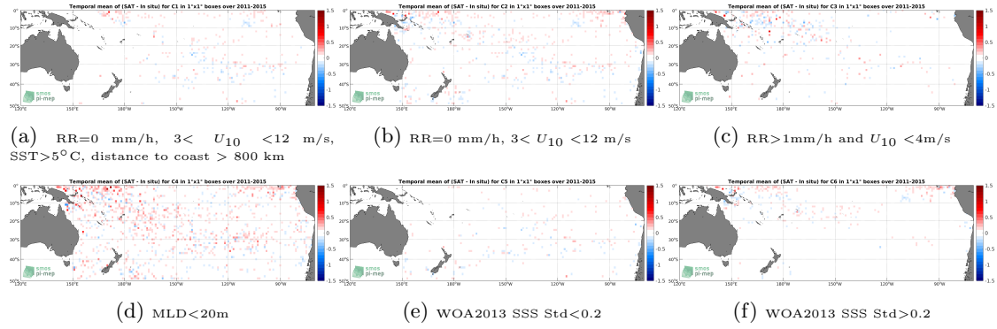
Figure 12: Temporal mean gridded over spatial boxes of size 1^\circ \times 1^\circ of \Delta SSS (Aquarius SSS L4 OI v5 - Weekly (IPRC) - Argo) for 6 different subdatasets corresponding to: RR=0 mm/h, 3 < U_{10} < 12 m/s, SST > 5^\circ C , distance to coast > 800 km (a), RR=0 mm/h, 3 < U_{10} < 12 m/s (b), RR > 1 mm/h and U_{10} < 4 m/s (c), MLD < 20 m (d), WOA2013 SSS Std < 0.2 (e), WOA2013 SSS Std > 0.2 (f).
