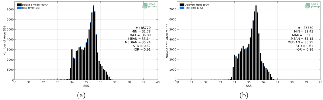
Figure 2: Histograms of SSS from Argo (a) and Aquarius SSS L4 OI v5 - Weekly (IPRC) (b) considering all match-up pairs per bins of 0.1 over the South Pacific Ocean Pi-MEP region and for the full satellite product period.
