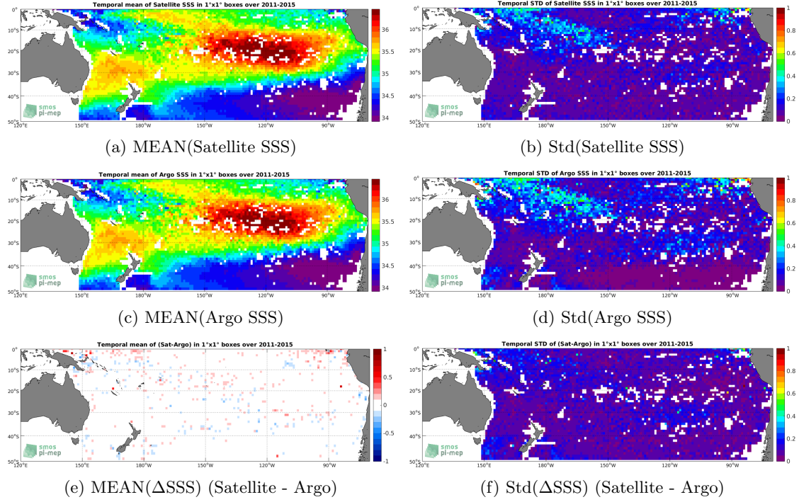
Figure 6: Temporal mean (left) and Std (right) of SSS from Aquarius-L4-IPRC-V5-WEEKLY (top), Argo (middle), and of \Delta SSS (Satellite - Argo). Only match-up pairs are used to generate these maps.
