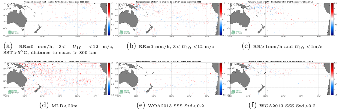
Figure 12: Temporal mean gridded over spatial boxes of size 1^\circ \times 1^\circ of \Delta SSS (Aquarius-L4-IPRC-V5-WEEKLY - Argo) for 6 different subdatasets corresponding to: RR=0 mm/h, 3 < U_{10} < 12 m/s, SST > 5^\circ\text{C} , distance to coast > 800 km (a), RR=0 mm/h, 3 < U_{10} < 12 m/s (b), RR > 1 mm/h and U_{10} < 4 m/s (c), MLD < 20 m (d), WOA2013 SSS Std < 0.2 (e), WOA2013 SSS Std > 0.2 (f).
