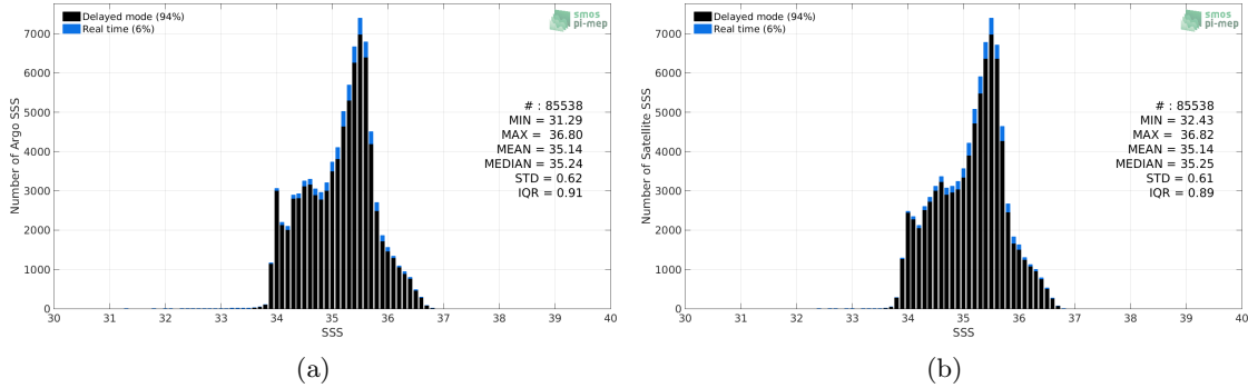
Figure 2: Histograms of SSS from Argo (a) and Aquarius-L4-IPRC-V5-WEEKLY (b) considering all match-up pairs per bins of 0.1 over the South Pacific Ocean Pi-MEP region and for the full satellite product period.
