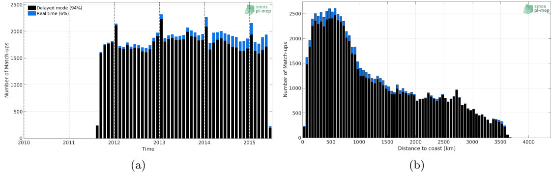
Figure 1: Number of match-ups between Argo and Aquarius-L4-IPRC-V5-WEEKLY SSS as a function of time (a) and as function of the distance to coast (b) over the South Pacific Ocean Pi-MEP region and for the full satellite product period.
