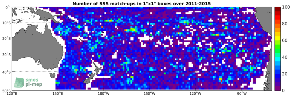
Figure 4: Number of SSS match-ups between Argo SSS and the Aquarius-L4-IPRC-V5-WEEKLY SSS product for the South Pacific Ocean Pi-MEP region over 1^\circ \times 1^\circ boxes and for the full satellite product period.
