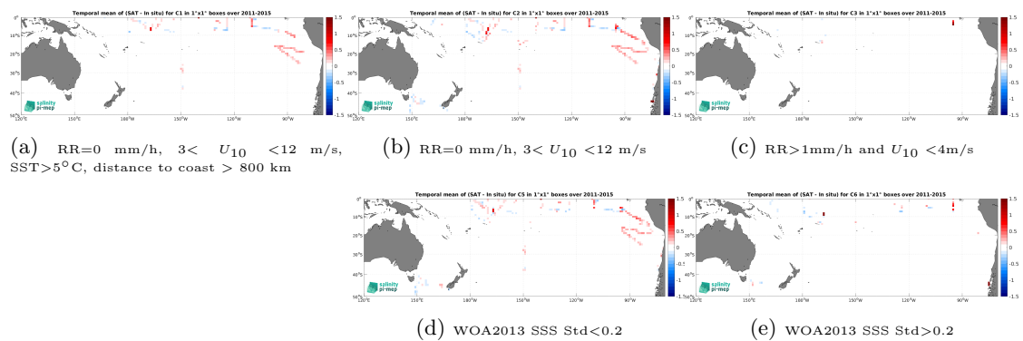
Figure 14: Temporal mean gridded over spatial boxes of size 1^\circ \times 1^\circ of \Delta SSS (Aquarius SSS L4 OI v5 - Monthly (IPRC) - TSG (SAMOS)) for 5 different subdatasets corresponding to:RR=0 mm/h, 3 < U_{10} < 12 m/s, SST >5^\circ\text{C} , distance to coast > 800 km (a), RR=0 mm/h, 3 < U_{10} < 12 m/s (b), RR >1 mm/h and U_{10} < 4 m/s (c), WOA2013 SSS Std <0.2 (d), WOA2013 SSS Std >0.2 (e).
