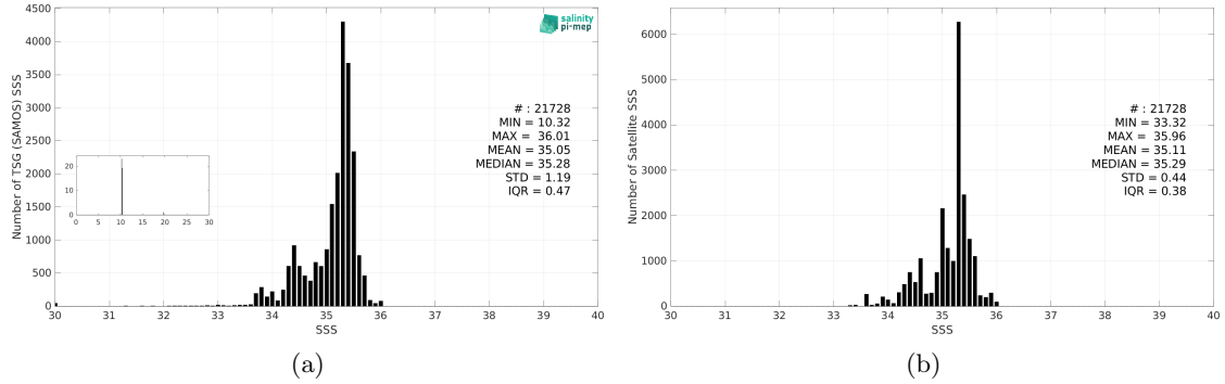
Figure 3: Histograms of SSS from TSG (SAMOS) (a) and Aquarius SSS L4 OI v5 - Monthly (IPRC) (b) considering all match-up pairs per bins of 0.1 over the South Pacific Ocean Pi-MEP region and for the full satellite product period.
