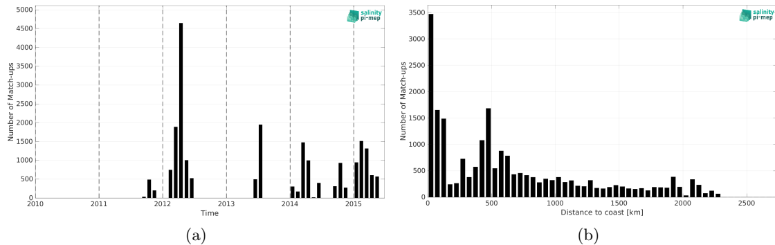
Figure 2: Number of match-ups between TSG (SAMOS) and Aquarius SSS L4 OI v5 - Monthly (IPRC) SSS as a function of time (a) and as function of the distance to coast (b) over the South Pacific Ocean Pi-MEP region and for the full satellite product period.
