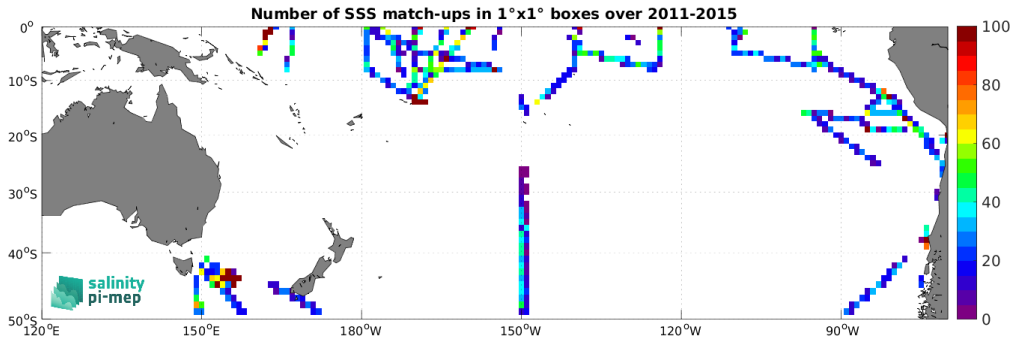
Figure 5: Number of SSS match-ups between TSG (SAMOS) SSS and the Aquarius SSS L4 OI v5 - Monthly (IPRC) SSS product for the South Pacific Ocean Pi-MEP region over 1^\circ \times 1^\circ boxes and for the full satellite product period.
