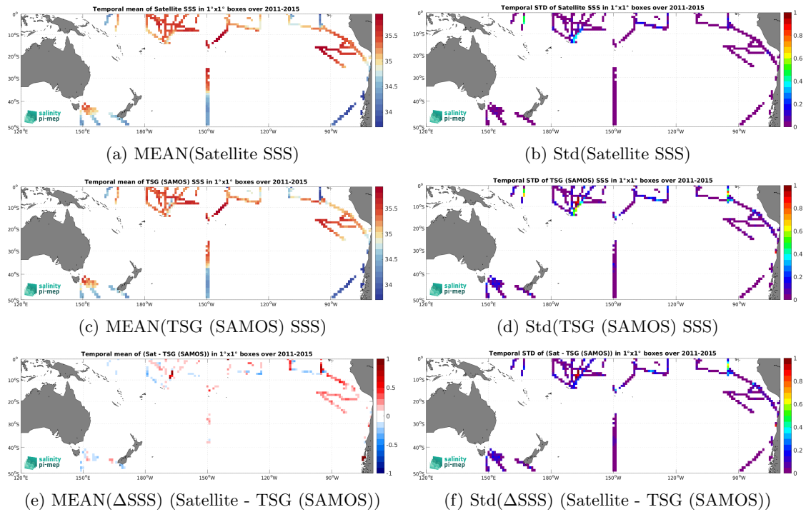
Figure 7: Temporal mean (left) and Std (right) of SSS from Aquarius SSS L4 OI v5 - Monthly (IPRC) (top), TSG (SAMOS) (middle), and of \Delta SSS (Satellite - TSG (SAMOS)). Only match-up pairs are used to generate these maps.
