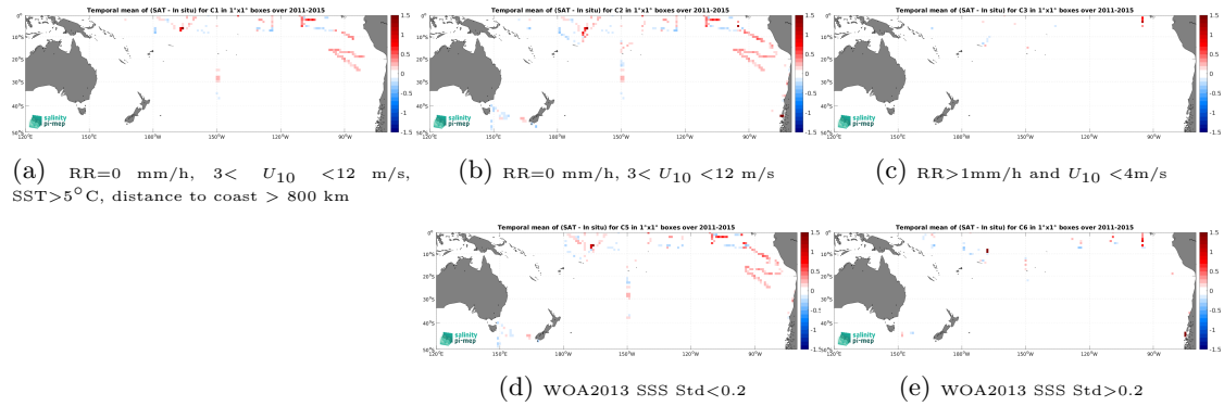
Figure 12: Temporal mean gridded over spatial boxes of size 1^\circ \times 1^\circ of \Delta SSS (Aquarius SSS L4 OI v5 - Monthly (IPRC) - TSG (SAMOS)) for 5 different subdatasets corresponding to:RR=0 mm/h, 3 < U_{10} < 12 m/s, SST >5^\circ\text{C} , distance to coast > 800 km (a), RR=0 mm/h, 3 < U_{10} < 12 m/s (b), RR >1 mm/h and U_{10} < 4 m/s (c), WOA2013 SSS Std <0.2 (d), WOA2013 SSS Std >0.2 (e).
