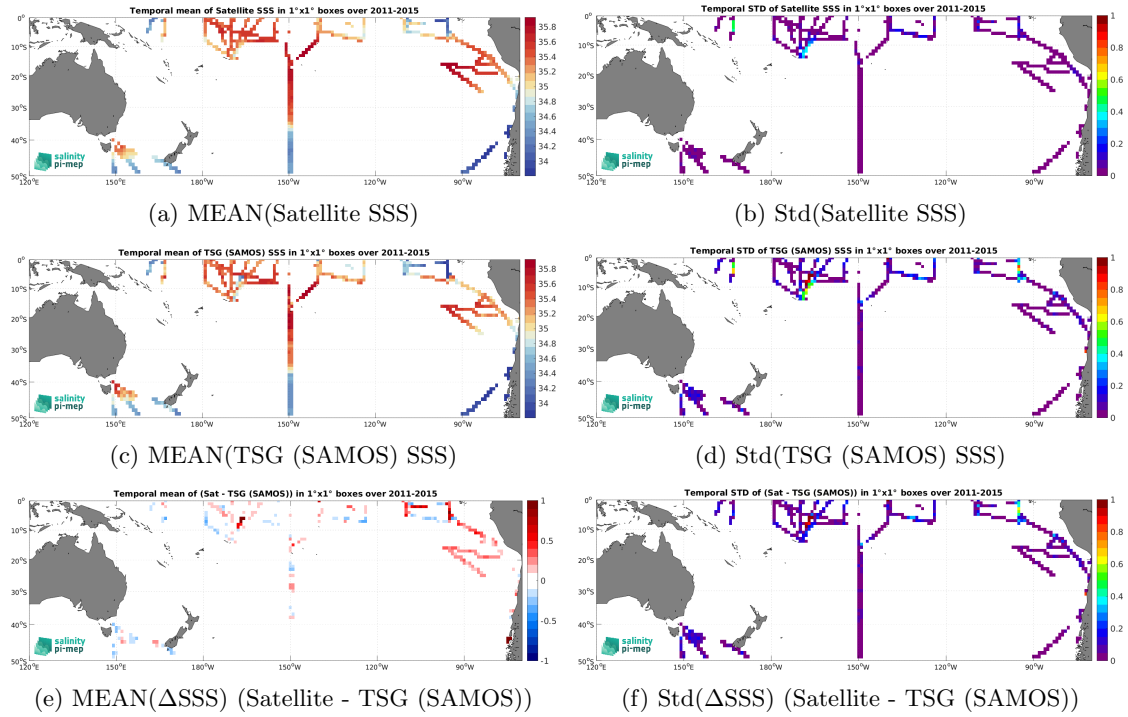
Figure 6: Temporal mean (left) and Std (right) of SSS from Aquarius SSS L4 OI v5 - Monthly (IPRC) (top), TSG (SAMOS) (middle), and of \Delta SSS (Satellite - TSG (SAMOS)). Only match-up pairs are used to generate these maps.
