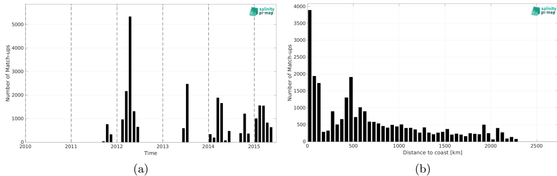
Figure 1: Number of match-ups between TSG (SAMOS) and Aquarius SSS L4 OI v5 - Monthly (IPRC) SSS as a function of time (a) and as function of the distance to coast (b) over the South Pacific Ocean Pi-MEP region and for the full satellite product period.
