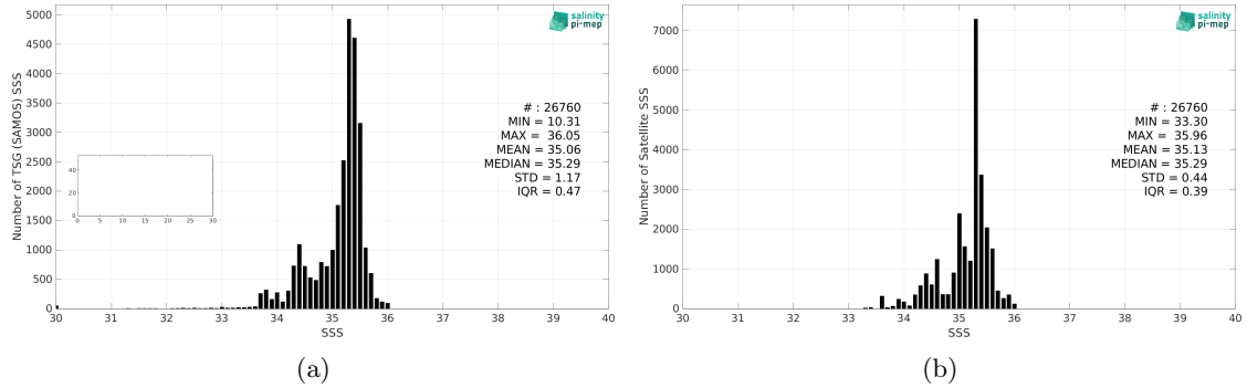
Figure 2: Histograms of SSS from TSG (SAMOS) (a) and Aquarius SSS L4 OI v5 - Monthly (IPRC) (b) considering all match-up pairs per bins of 0.1 over the South Pacific Ocean Pi-MEP region and for the full satellite product period.
