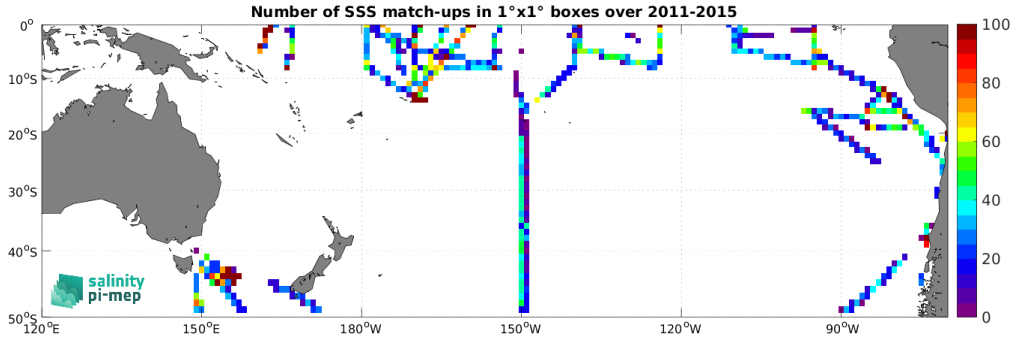
Figure 4: Number of SSS match-ups between TSG (SAMOS) SSS and the Aquarius SSS L4 OI v5 - Monthly (IPRC) SSS product for the South Pacific Ocean Pi-MEP region over 1^\circ \times 1^\circ boxes and for the full satellite product period.
