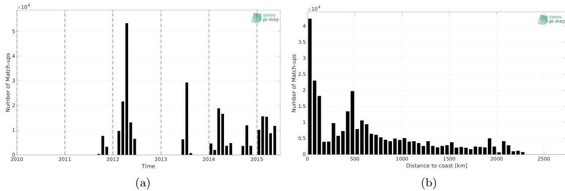
Figure 1: Number of match-ups between TSG (SAMOS) and Aquarius SSS L4 OI v5 - Monthly (IPRC) SSS as a function of time (a) and as function of the distance to coast (b) over the South Pacific Ocean Pi-MEP region and for the full satellite product period.
