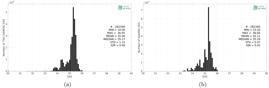
Figure 2: Histograms of SSS from TSG (SAMOS) (a) and Aquarius SSS L4 OI v5 - Monthly (IPRC) (b) considering all match-up pairs per bins of 0.1 over the South Pacific Ocean Pi-MEP region and for the full satellite product period.
