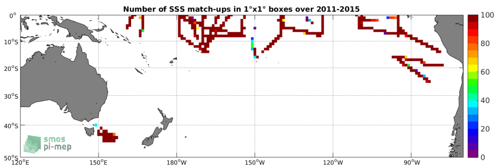
Figure 4: Number of SSS match-ups between TSG-SAMOS SSS and the Aquarius-L4-IPRC-V5-MONTHLY SSS product for the South Pacific Ocean Pi-MEP region over 1°x1° boxes and for the full satellite product period.
