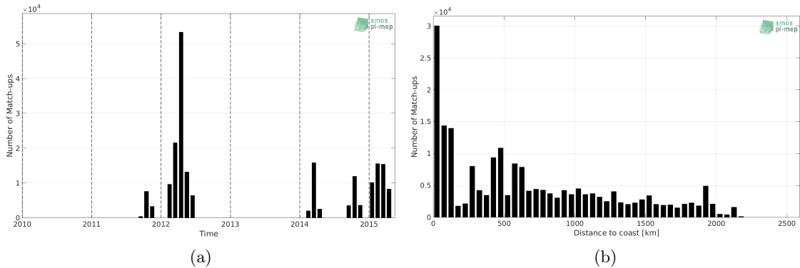
Figure 1: Number of match-ups between TSG-SAMOS and Aquarius-L4-IPRC-V5-MONTHLY SSS as a function of time (a) and as function of the distance to coast (b) over the South Pacific Ocean Pi-MEP region and for the full satellite product period.
