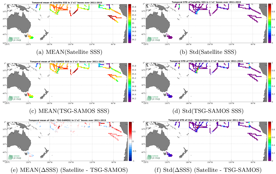
Figure 6: Temporal mean (left) and Std (right) of SSS from Aquarius-L4-IPRC-V5-MONTHLY (top), TSG-SAMOS (middle), and of \Delta SSS (Satellite - TSG-SAMOS). Only match-up pairs are used to generate these maps.
