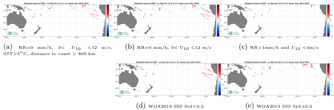
Figure 12: Temporal mean gridded over spatial boxes of size 1^\circ \times 1^\circ of \Delta SSS (Aquarius-L4-IPRC-V5-MONTHLY - TSG-SAMOS) for 5 different subdatasets corresponding to:RR=0 mm/h, 3 < U_{10} < 12 m/s, SST >5^\circ\text{C} , distance to coast > 800 km (a), RR=0 mm/h, 3 < U_{10} < 12 m/s (b), RR >1 mm/h and U_{10} < 4 m/s (c), WOA2013 SSS Std <0.2 (d), WOA2013 SSS Std >0.2 (e).
