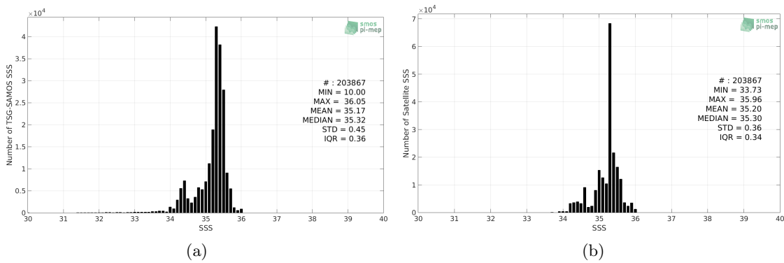
Figure 2: Histograms of SSS from TSG-SAMOS (a) and Aquarius-L4-IPRC-V5-MONTHLY (b) considering all match-up pairs per bins of 0.1 over the South Pacific Ocean Pi-MEP region and for the full satellite product period.
