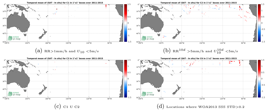
Figure 12: Temporal mean gridded over spatial boxes of size 1^\circ \times 1^\circ of \Delta SSS (Aquarius-L4-IPRC-V5-MONTHLY - TSG-SAMOS) for 4 different subdatasets corresponding to: RR > 1\text{mm/h} and U_{10} < 5\text{m/s} (a), RR^{10d} > 5\text{mm/h} and U_{10}^{10d} < 5\text{m/s} (b), C1 U C2 (c), Locations where WOA2013 SSS STD > 0.2 (d).
