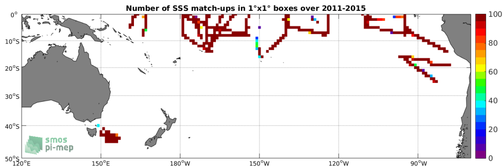
Figure 4: Number of SSS match-ups between TSG-SAMOS SSS and the Aquarius-L4-IPRC-V5-MONTHLY SSS product for the South Pacific Ocean Pi-MEP region over 1^\circ \times 1^\circ boxes and for the full satellite product period.
