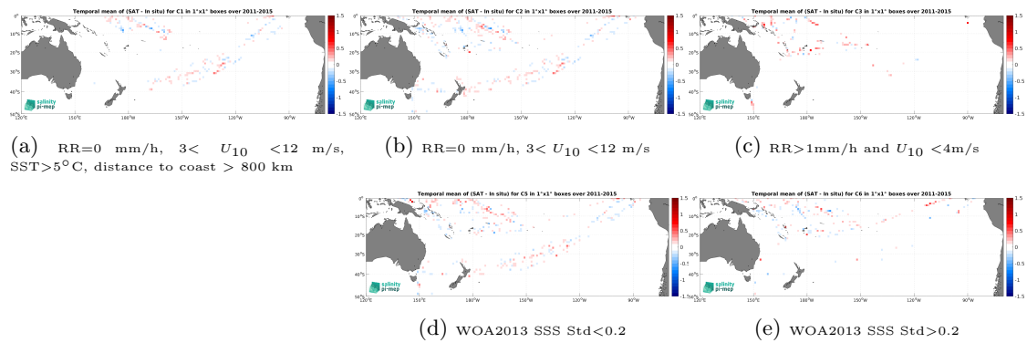
Figure 14: Temporal mean gridded over spatial boxes of size 1^\circ \times 1^\circ of \Delta\text{SSS} (Aquarius SSS L4 OI v5 - Monthly (IPRC) - TSG (LEGOS-DM)) for 5 different subdatasets corresponding to:RR=0 mm/h, 3 < U_{10} < 12 m/s, SST>5°C, distance to coast > 800 km (a), RR=0 mm/h, 3 < U_{10} < 12 m/s (b), RR>1mm/h and U_{10} < 4 m/s (c), WOA2013 SSS Std<0.2 (d), WOA2013 SSS Std>0.2 (e).
