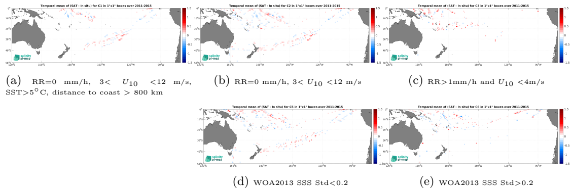
Figure 12: Temporal mean gridded over spatial boxes of size 1^\circ \times 1^\circ of \Delta\text{SSS} (Aquarius SSS L4 OI v5 - Monthly (IPRC) - TSG (LEGOS-DM)) for 5 different subdatasets corresponding to:RR=0 mm/h, 3 < U_{10} < 12 m/s, SST >5^\circ\text{C} , distance to coast > 800 km (a), RR=0 mm/h, 3 < U_{10} < 12 m/s (b), RR >1 mm/h and U_{10} < 4 m/s (c), WOA2013 SSS Std <0.2 (d), WOA2013 SSS Std >0.2 (e).
