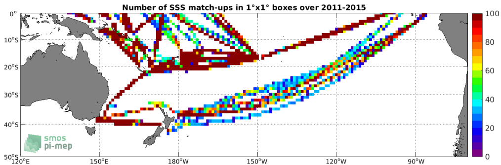
Figure 4: Number of SSS match-ups between TSG (LEGOS-DM) SSS and the Aquarius SSS L4 OI v5 - Monthly (IPRC) SSS product for the South Pacific Ocean Pi-MEP region over 1^\circ \times 1^\circ boxes and for the full satellite product period.
