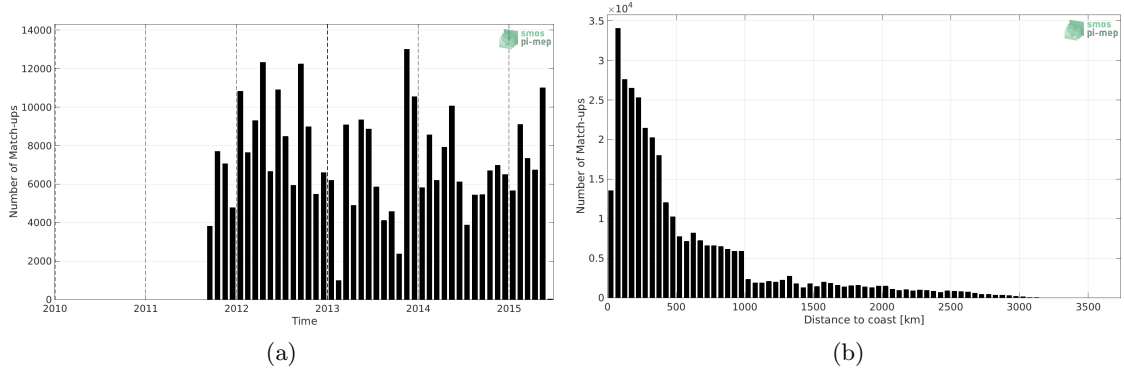
Figure 1: Number of match-ups between TSG (LEGOS-DM) and Aquarius SSS L4 OI v5 - Monthly (IPRC) SSS as a function of time (a) and as function of the distance to coast (b) over the South Pacific Ocean Pi-MEP region and for the full satellite product period.
