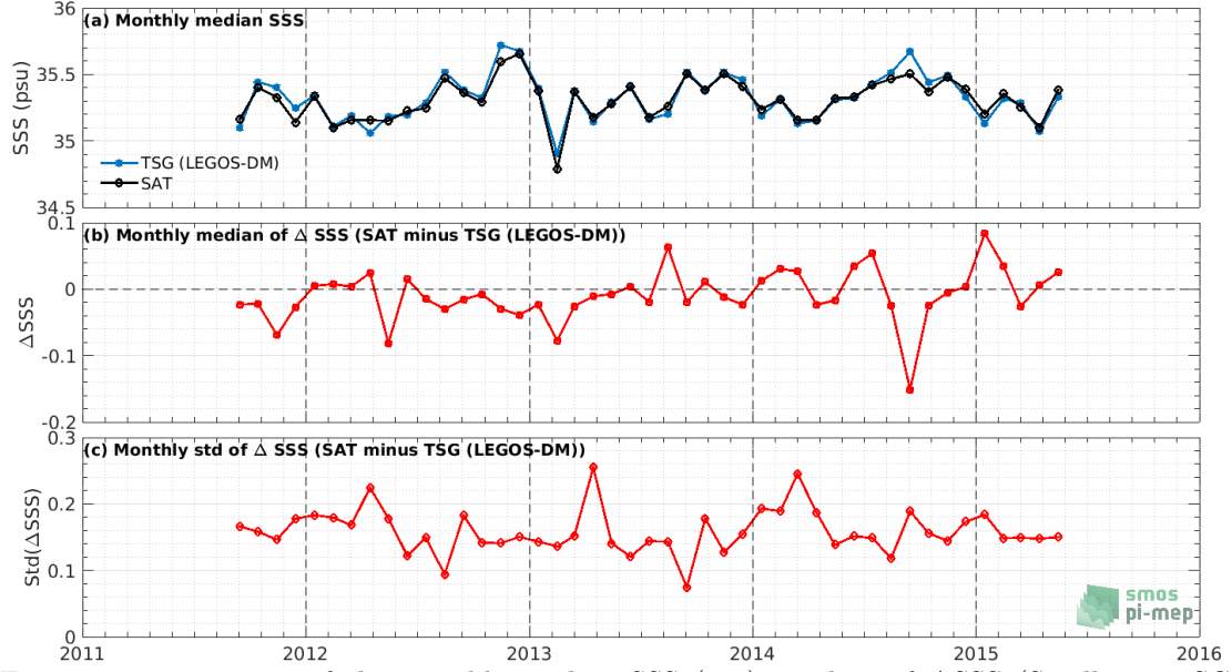
Figure 7: Time series of the monthly median SSS (top), median of \Delta\text{SSS} (Satellite - TSG (LEGOS-DM)) and Std of \Delta\text{SSS} (Satellite - TSG (LEGOS-DM)) over the South Pacific Ocean Pi-MEP region considering all match-ups collected by the Pi-MEP.
