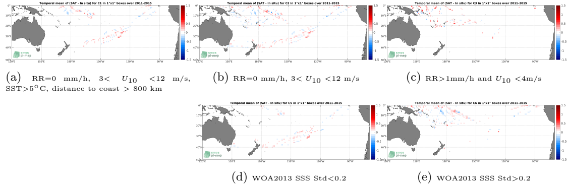
Figure 12: Temporal mean gridded over spatial boxes of size 1^\circ \times 1^\circ of \Delta SSS (Aquarius SSS L4 OI v5 - Monthly (IPRC) - TSG (LEGOS-DM)) for 5 different subdatasets corresponding to: RR=0 mm/h, 3 < U_{10} < 12 m/s, SST > 5^\circ C , distance to coast > 800 km (a), RR=0 mm/h, 3 < U_{10} < 12 m/s (b), RR > 1 mm/h and U_{10} < 4 m/s (c), WOA2013 SSS Std < 0.2 (d), WOA2013 SSS Std > 0.2 (e).
