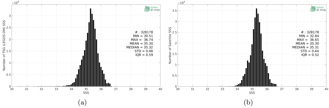
Figure 2: Histograms of SSS from TSG (LEGOS-DM) (a) and Aquarius SSS L4 OI v5 - Monthly (IPRC) (b) considering all match-up pairs per bins of 0.1 over the South Pacific Ocean Pi-MEP region and for the full satellite product period.
