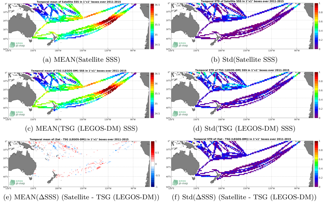
Figure 6: Temporal mean (left) and Std (right) of SSS from Aquarius SSS L4 OI v5 - Monthly (IPRC) (top), TSG (LEGOS-DM) (middle), and of \Delta SSS (Satellite - TSG (LEGOS-DM)). Only match-up pairs are used to generate these maps.
