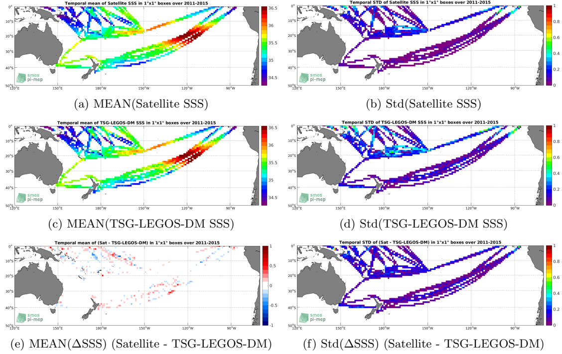
Figure 6: Temporal mean (left) and Std (right) of SSS from Aquarius-L4-IPRC-V5-MONTHLY (top), TSG-LEGOS-DM (middle), and of \Delta SSS (Satellite - TSG-LEGOS-DM). Only match-up pairs are used to generate these maps.
