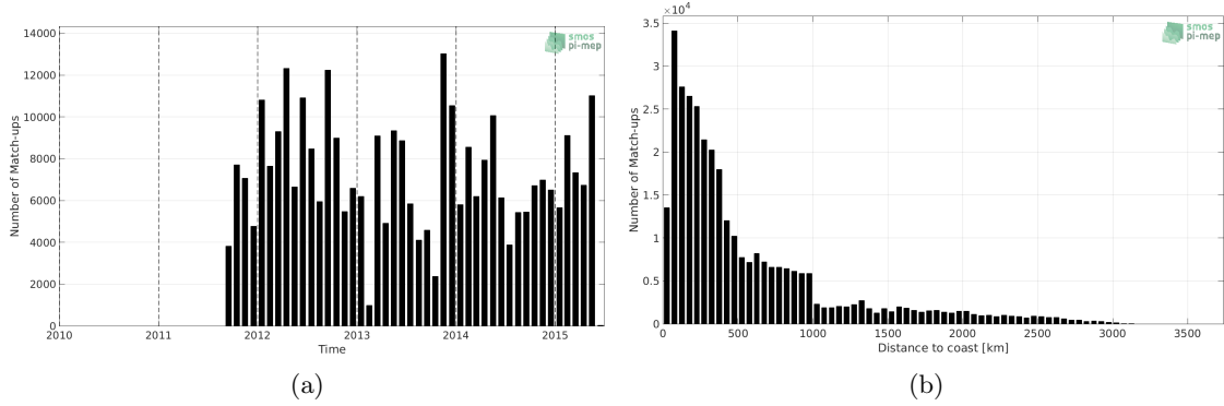
Figure 1: Number of match-ups between TSG-LEGOS-DM and Aquarius-L4-IPRC-V5-MONTHLY SSS as a function of time (a) and as function of the distance to coast (b) over the South Pacific Ocean Pi-MEP region and for the full satellite product period.
