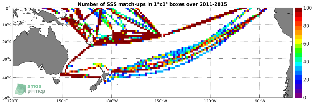
Figure 4: Number of SSS match-ups between TSG-LEGOS-DM SSS and the Aquarius-L4-IPRC-V5-MONTHLY SSS product for the South Pacific Ocean Pi-MEP region over 1°x1° boxes and for the full satellite product period.
