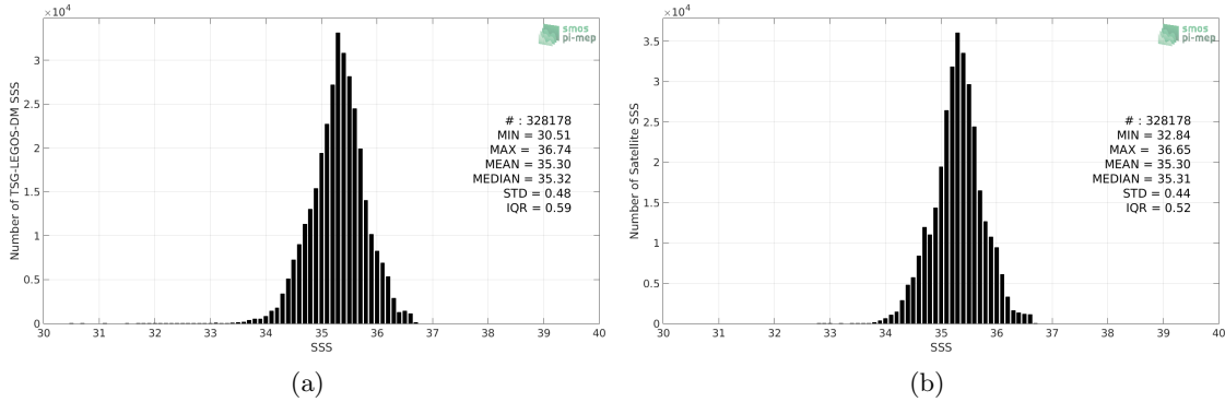
Figure 2: Histograms of SSS from TSG-LEGOS-DM (a) and Aquarius-L4-IPRC-V5-MONTHLY (b) considering all match-up pairs per bins of 0.1 over the South Pacific Ocean Pi-MEP region and for the full satellite product period.
