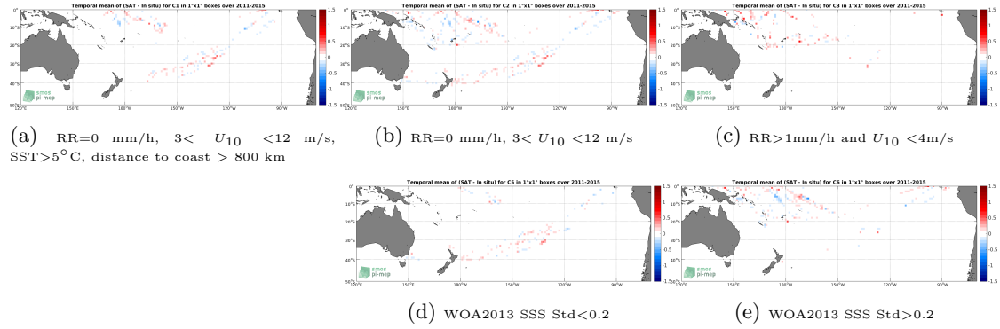
Figure 12: Temporal mean gridded over spatial boxes of size 1^\circ \times 1^\circ of \Delta SSS (Aquarius-L4-IPRC-V5-MONTHLY - TSG-LEGOS-DM) for 5 different subdatasets corresponding to: RR=0 mm/h, 3 < U_{10} < 12 m/s, SST > 5^\circ\text{C} , distance to coast > 800 km (a), RR=0 mm/h, 3 < U_{10} < 12 m/s (b), RR > 1 mm/h and U_{10} < 4 m/s (c), WOA2013 SSS Std < 0.2 (d), WOA2013 SSS Std > 0.2 (e).
