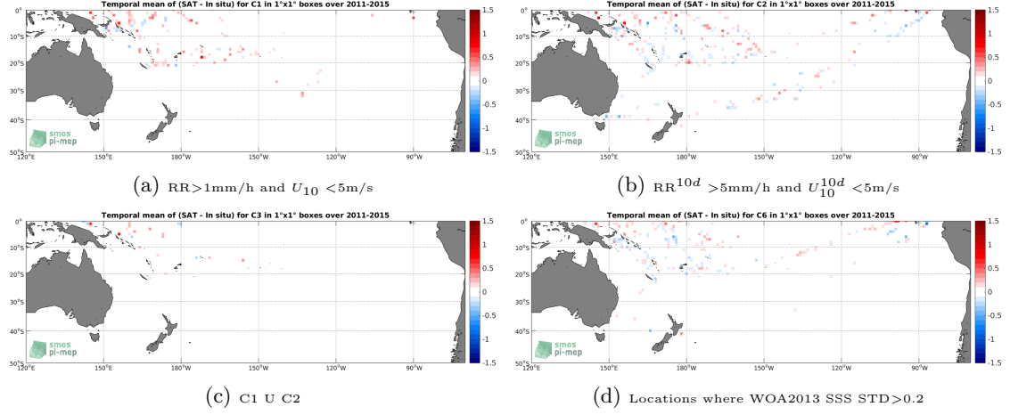
Figure 12: Temporal mean gridded over spatial boxes of size 1^\circ \times 1^\circ of \Delta SSS (Aquarius-L4-IPRC-V5-MONTHLY - TSG-LEGOS-DM) for 4 different subdatasets corresponding to: RR > 1\text{mm/h} and U_{10} < 5\text{m/s} (a), RR^{10d} > 5\text{mm/h} and U_{10}^{10d} < 5\text{m/s} (b), C1 U C2 (c), Locations where WOA2013 SSS STD > 0.2 (d).
