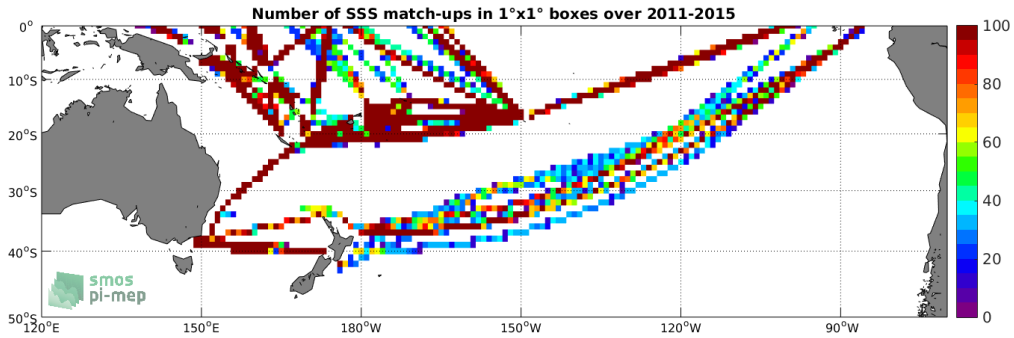
Figure 4: Number of SSS match-ups between TSG-LEGOS-DM SSS and the Aquarius-L4-IPRC-V5-MONTHLY SSS product for the South Pacific Ocean Pi-MEP region over 1^\circ \times 1^\circ boxes and for the full satellite product period.
