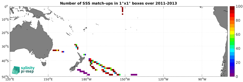
Figure 5: Number of SSS match-ups between TSG (GOSUD-Sailing-ship) SSS and the Aquarius SSS L4 OI v5 - Monthly (IPRC) SSS product for the South Pacific Ocean Pi-MEP region over 1^\circ \times 1^\circ boxes and for the full satellite product period.
