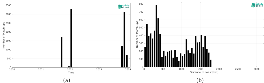
Figure 2: Number of match-ups between TSG (GOSUD-Sailing-ship) and Aquarius SSS L4 OI v5 - Monthly (IPRC) SSS as a function of time (a) and as function of the distance to coast (b) over the South Pacific Ocean Pi-MEP region and for the full satellite product period.
