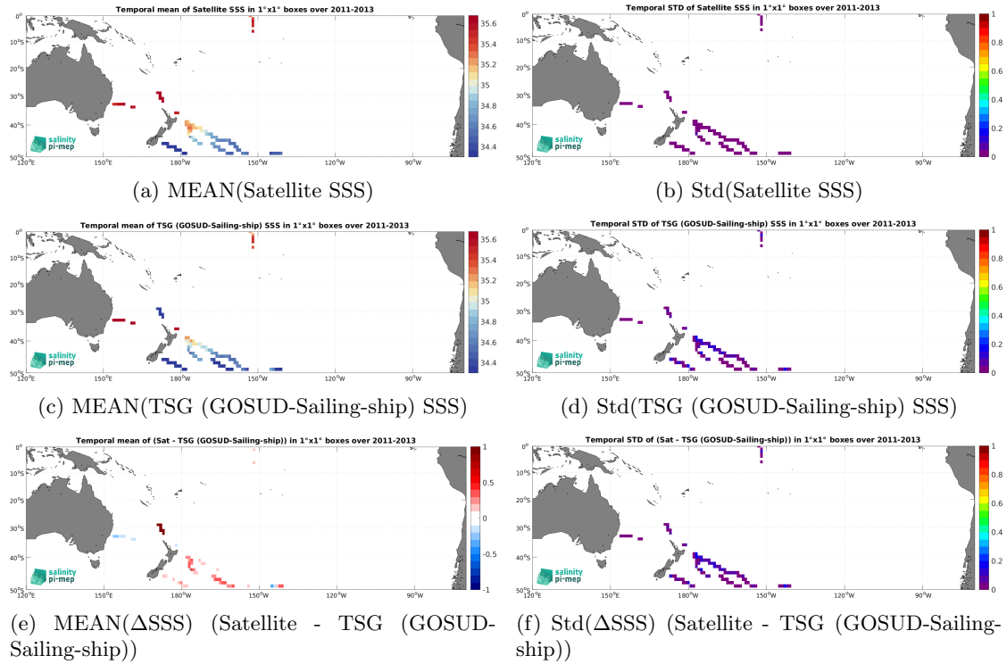
Figure 7: Temporal mean (left) and Std (right) of SSS from Aquarius SSS L4 OI v5 - Monthly (IPRC) (top), TSG (GOSUD-Sailing-ship) (middle), and of \Delta SSS (Satellite - TSG (GOSUD-Sailing-ship)). Only match-up pairs are used to generate these maps.
