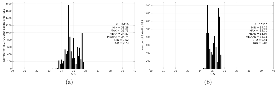
Figure 3: Histograms of SSS from TSG (GOSUD-Sailing-ship) (a) and Aquarius SSS L4 OI v5 - Monthly (IPRC) (b) considering all match-up pairs per bins of 0.1 over the South Pacific Ocean Pi-MEP region and for the full satellite product period.
