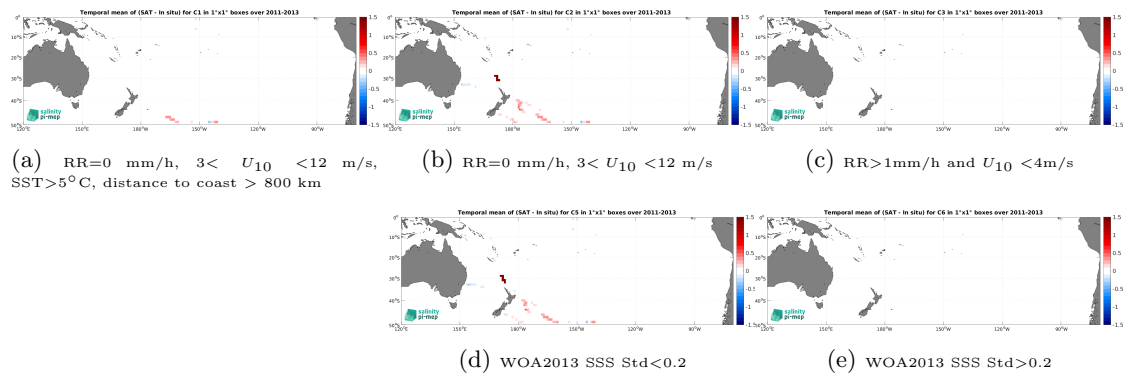
Figure 14: Temporal mean gridded over spatial boxes of size 1^\circ \times 1^\circ of \Delta SSS (Aquarius SSS L4 OI v5 - Monthly (IPRC) - TSG (GOSUD-Sailing-ship)) for 5 different subdatasets corresponding to:RR=0 mm/h, 3 < U_{10} < 12 m/s, SST >5^\circ\text{C} , distance to coast > 800 km (a), RR=0 mm/h, 3 < U_{10} < 12 m/s (b), RR >1 mm/h and U_{10} < 4 m/s (c), WOA2013 SSS Std <0.2 (d), WOA2013 SSS Std >0.2 (e).
