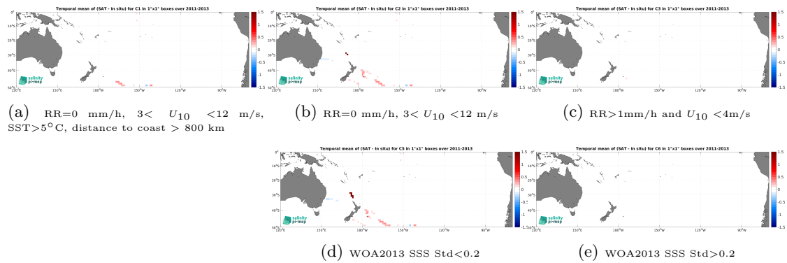
Figure 12: Temporal mean gridded over spatial boxes of size 1^\circ \times 1^\circ of \Delta\text{SSS} (Aquarius SSS L4 OI v5 - Monthly (IPRC) - TSG (GOSUD-Sailing-ship)) for 5 different subdatasets corresponding to:RR=0 mm/h, 3 < U_{10} < 12 m/s, SST>5°C, distance to coast > 800 km (a), RR=0 mm/h, 3 < U_{10} < 12 m/s (b), RR>1mm/h and U_{10} < 4 m/s (c), WOA2013 SSS Std<0.2 (d), WOA2013 SSS Std>0.2 (e).
