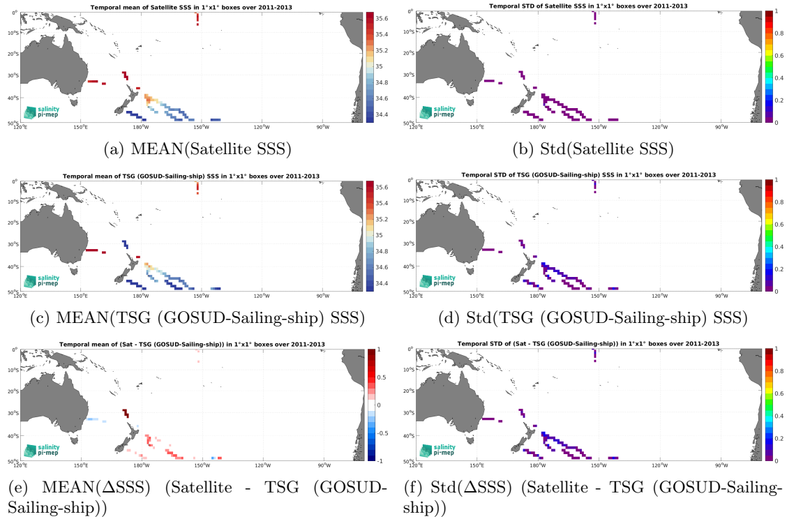
Figure 6: Temporal mean (left) and Std (right) of SSS from Aquarius SSS L4 OI v5 - Monthly (IPRC) (top), TSG (GOSUD-Sailing-ship) (middle), and of \Delta SSS (Satellite - TSG (GOSUD-Sailing-ship)). Only match-up pairs are used to generate these maps.
