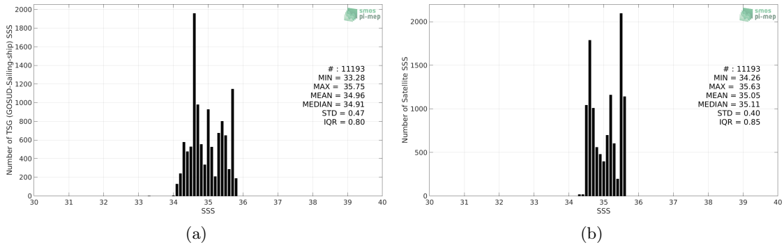
Figure 2: Histograms of SSS from TSG (GOSUD-Sailing-ship) (a) and Aquarius SSS L4 OI v5 - Monthly (IPRC) (b) considering all match-up pairs per bins of 0.1 over the South Pacific Ocean Pi-MEP region and for the full satellite product period.
