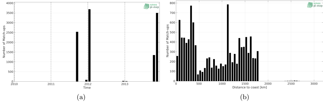
Figure 1: Number of match-ups between TSG (GOSUD-Sailing-ship) and Aquarius SSS L4 OI v5 - Monthly (IPRC) SSS as a function of time (a) and as function of the distance to coast (b) over the South Pacific Ocean Pi-MEP region and for the full satellite product period.
