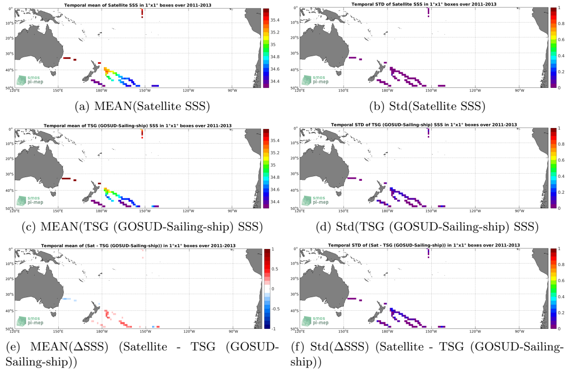
Figure 6: Temporal mean (left) and Std (right) of SSS from Aquarius SSS L4 OI v5 - Monthly (IPRC) (top), TSG (GOSUD-Sailing-ship) (middle), and of \Delta SSS (Satellite - TSG (GOSUD-Sailing-ship)). Only match-up pairs are used to generate these maps.
