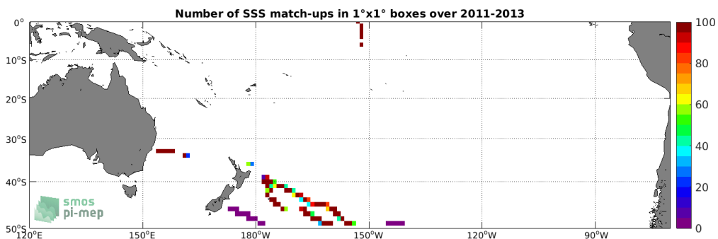
Figure 4: Number of SSS match-ups between TSG (GOSUD-Sailing-ship) SSS and the Aquarius SSS L4 OI v5 - Monthly (IPRC) SSS product for the South Pacific Ocean Pi-MEP region over 1^\circ \times 1^\circ boxes and for the full satellite product period.
