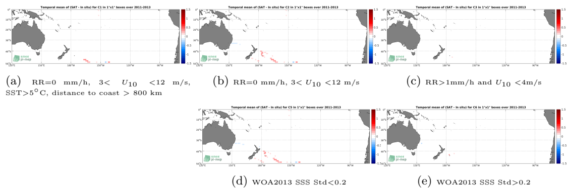
Figure 12: Temporal mean gridded over spatial boxes of size 1^\circ \times 1^\circ of \Delta SSS (Aquarius-L4-IPRC-V5-MONTHLY - TSG-GOSUD-Sailing-ship) for 5 different subdatasets corresponding to:RR=0 mm/h, 3 < U_{10} < 12 m/s, SST >5^\circ\text{C} , distance to coast > 800 km (a), RR=0 mm/h, 3 < U_{10} < 12 m/s (b), RR >1 mm/h and U_{10} < 4 m/s (c), WOA2013 SSS Std <0.2 (d), WOA2013 SSS Std >0.2 (e).
