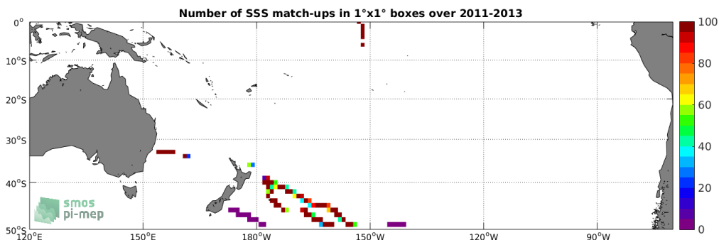
Figure 4: Number of SSS match-ups between TSG-GOSUD-Sailing-ship SSS and the Aquarius-L4-IPRC-V5-MONTHLY SSS product for the South Pacific Ocean Pi-MEP region over 1°x1° boxes and for the full satellite product period.
