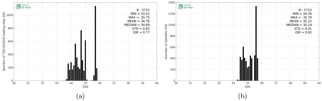
Figure 2: Histograms of SSS from TSG-GOSUD-Sailing-ship (a) and Aquarius-L4-IPRC-V5-MONTHLY (b) considering all match-up pairs per bins of 0.1 over the South Pacific Ocean Pi-MEP region and for the full satellite product period.
