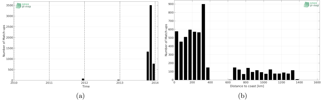
Figure 1: Number of match-ups between TSG-GOSUD-Sailing-ship and Aquarius-L4-IPRC-V5-MONTHLY SSS as a function of time (a) and as function of the distance to coast (b) over the South Pacific Ocean Pi-MEP region and for the full satellite product period.
