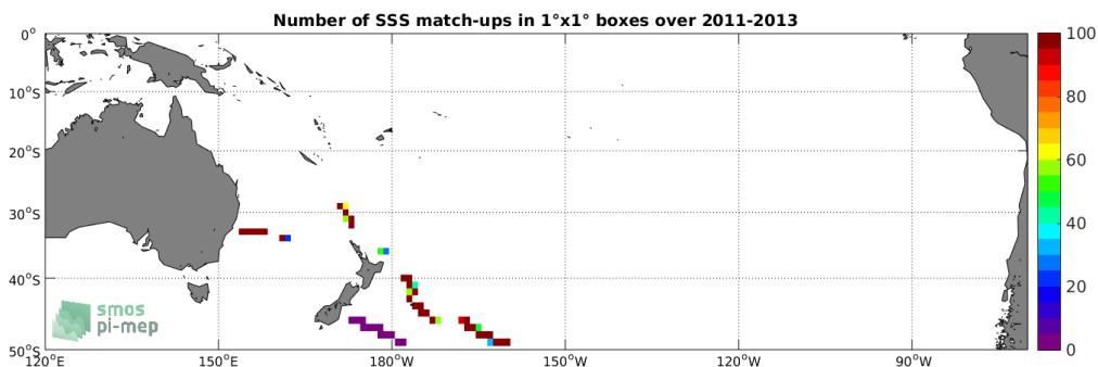
Figure 4: Number of SSS match-ups between TSG-GOSUD-Sailing-ship SSS and the Aquarius-L4-IPRC-V5-MONTHLY SSS product for the South Pacific Ocean Pi-MEP region over 1^\circ \times 1^\circ boxes and for the full satellite product period.
