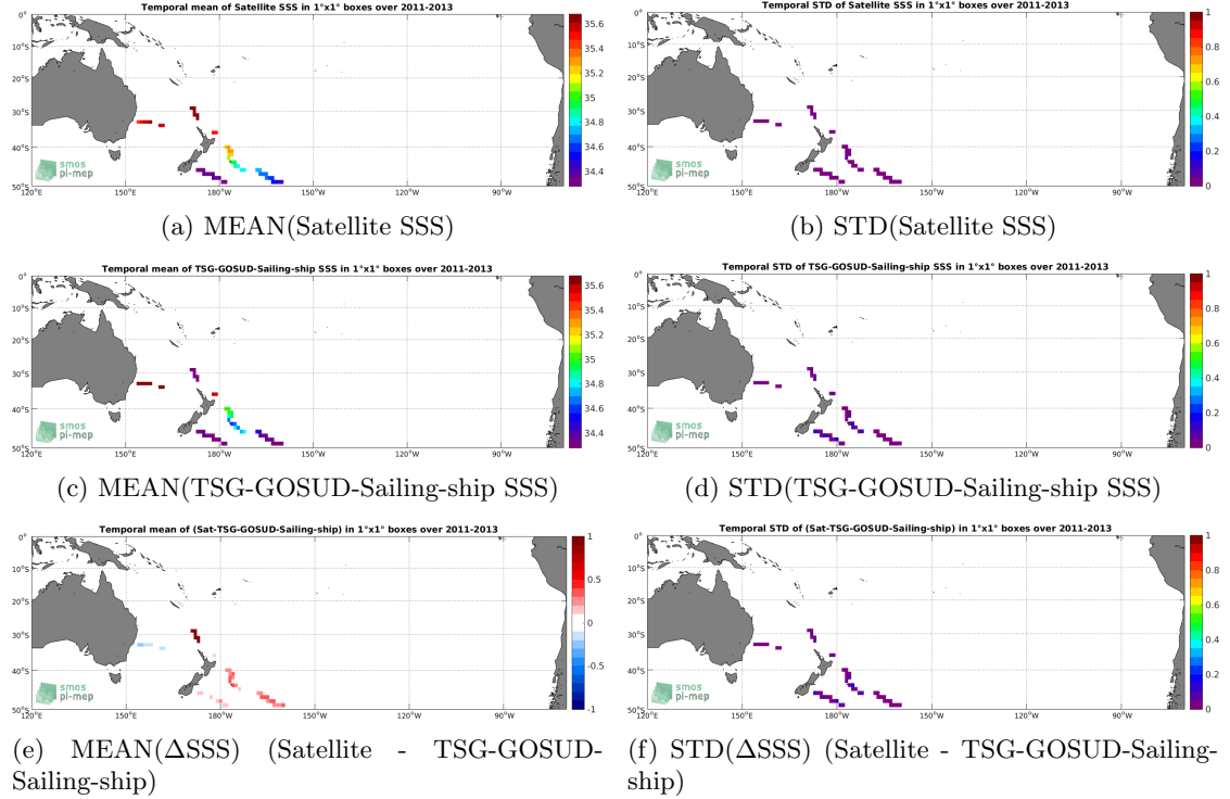
Figure 6: Temporal mean (left) and STD (right) of SSS from Aquarius-L4-IPRC-V5-MONTHLY (top), TSG-GOSUD-Sailing-ship (middle), and of \Delta SSS (Satellite - TSG-GOSUD-Sailing-ship). Only match-up pairs are used to generate these maps.
