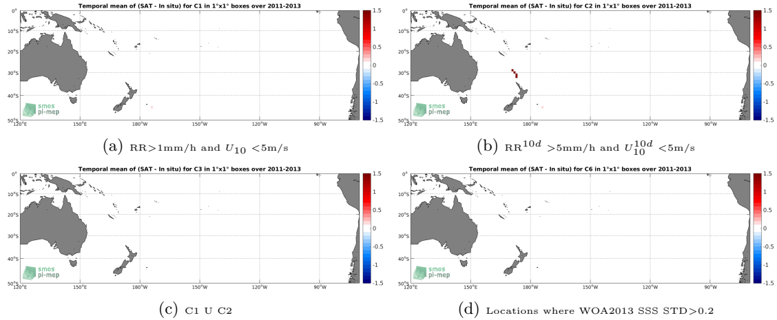
Figure 12: Temporal mean gridded over spatial boxes of size 1^\circ \times 1^\circ of \Delta SSS (Aquarius-L4-IPRC-V5-MONTHLY - TSG-GOSUD-Sailing-ship) for 4 different subdatasets corresponding to: RR > 1\text{mm/h} and U_{10} < 5\text{m/s} (a), RR^{10d} > 5\text{mm/h} and U_{10}^{10d} < 5\text{m/s} (b), C1 U C2 (c), Locations where WOA2013 SSS STD > 0.2 (d).
